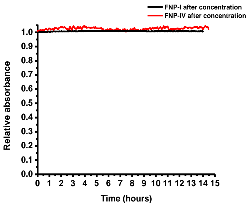
Figure 3. 20. Relative absorbance of FNP-I (black; OD =1.1) and FNP-IV (red; OD = 0.7) after concentration, in 0.9 %wt salt solution for 15 hours recorded at \lambda = 470 nm and \lambda = 480 nm respectively.
