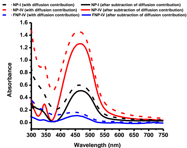
Figure 2. 25. Absorbance spectra of NP-I, NP-IV and FNP-IV, before (dotted) and after removal of diffusion contribution (solid).
