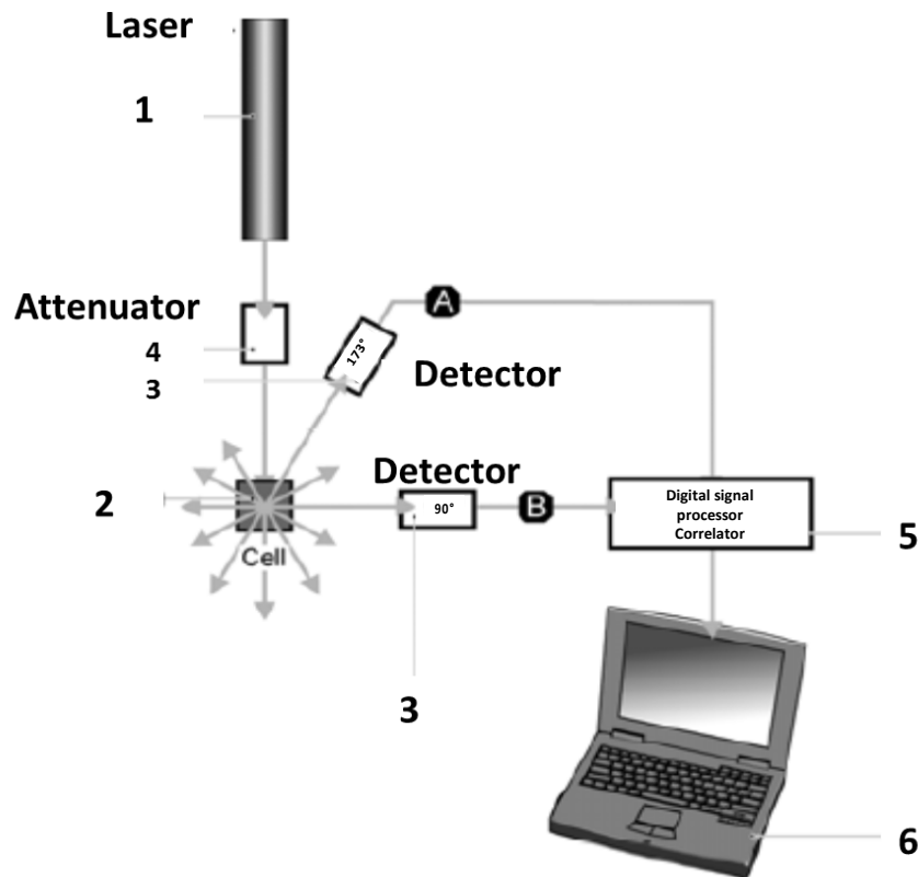
Figure A2.6. Optical configurations of a commercial DLS setup 1
