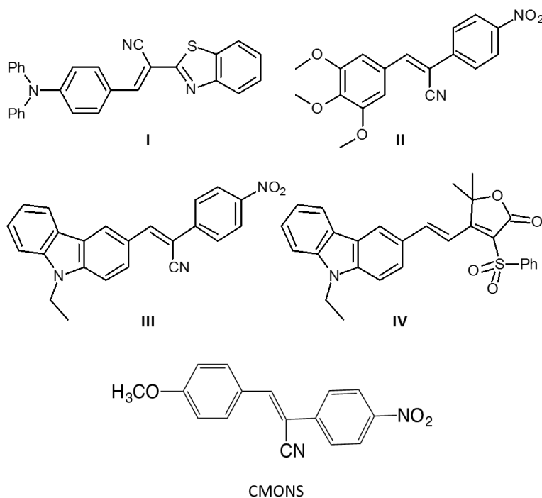
Figure 2. 4. Structure of the organic dyes
