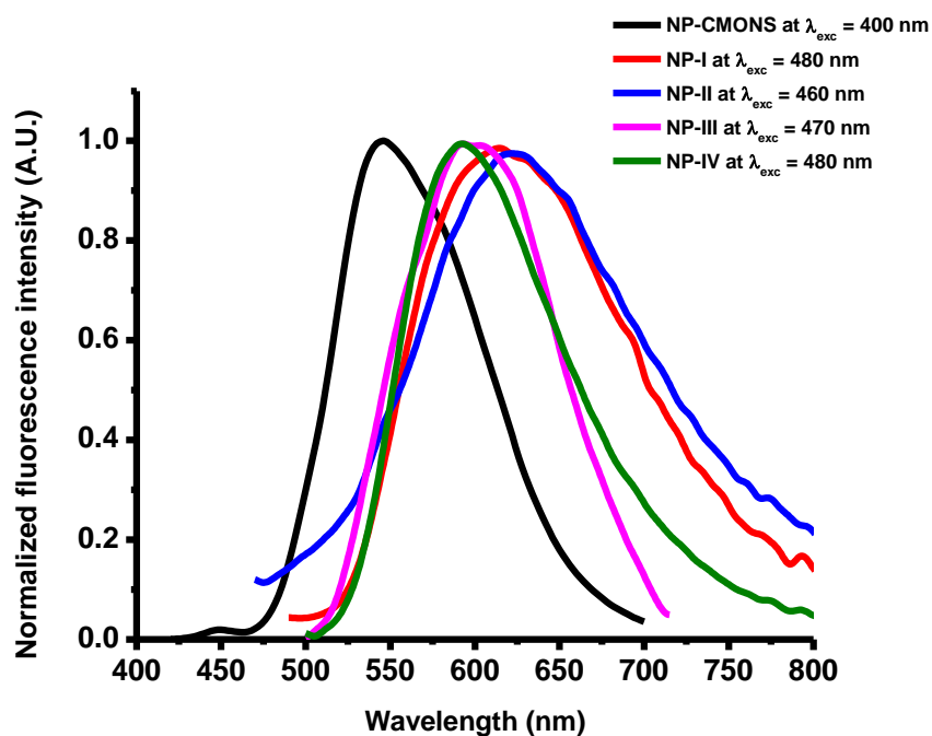
Figure 2. 24. Fluorescence spectra of organic dyes confined in NPs
