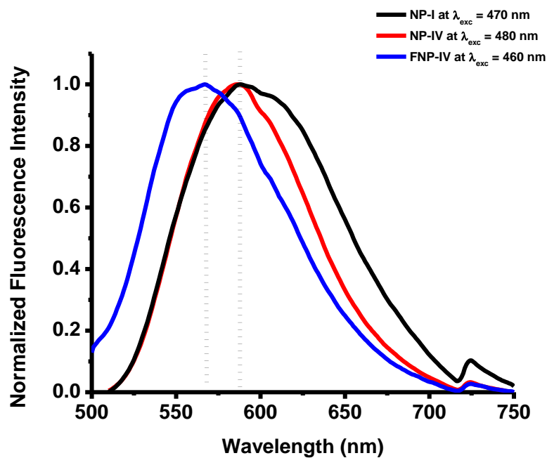
Figure 2. 26. Normalized fluorescence emission spectra of NP-I, NP-IV and FNP-IV
