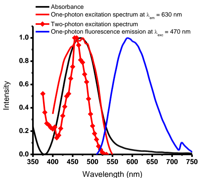
Figure 2. 28. Absorbance (black), one-photon (red) and two-photon excitation spectra (red symbol, raw data) and emission spectra (blue) of NP-I
