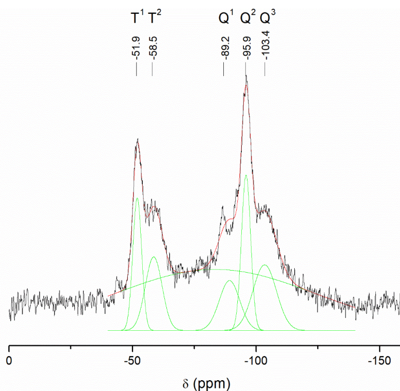
Figure 2. 7. ^{29}\text{Si} NMR-spectrum of sol made using protocol B
