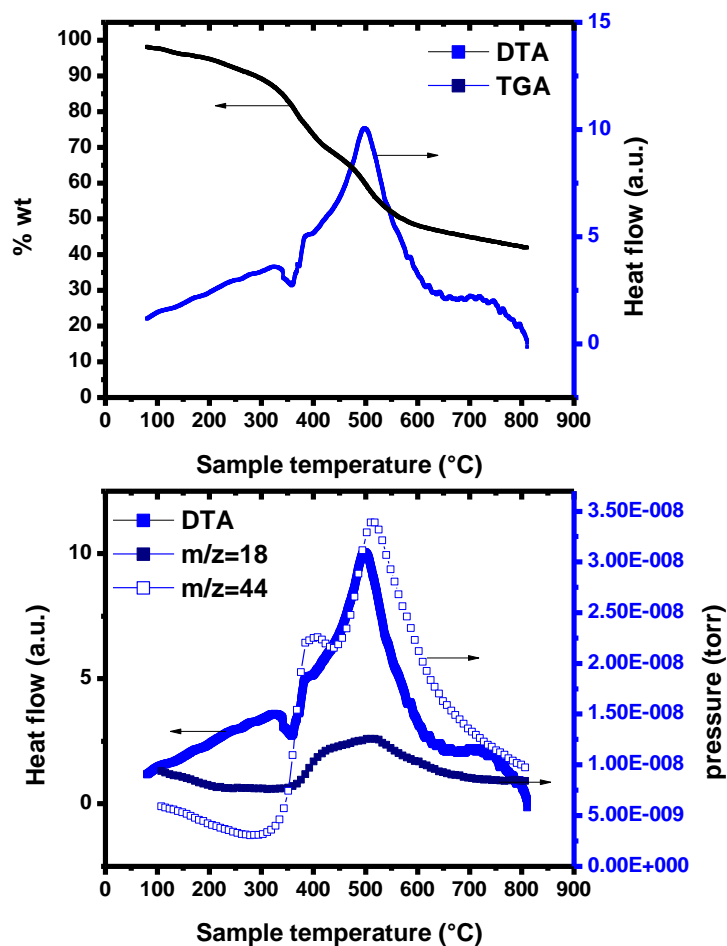
Figure 2. 20. TGA-DTA-MS analysis of NP-I at 8K/min under Ar/O 2
