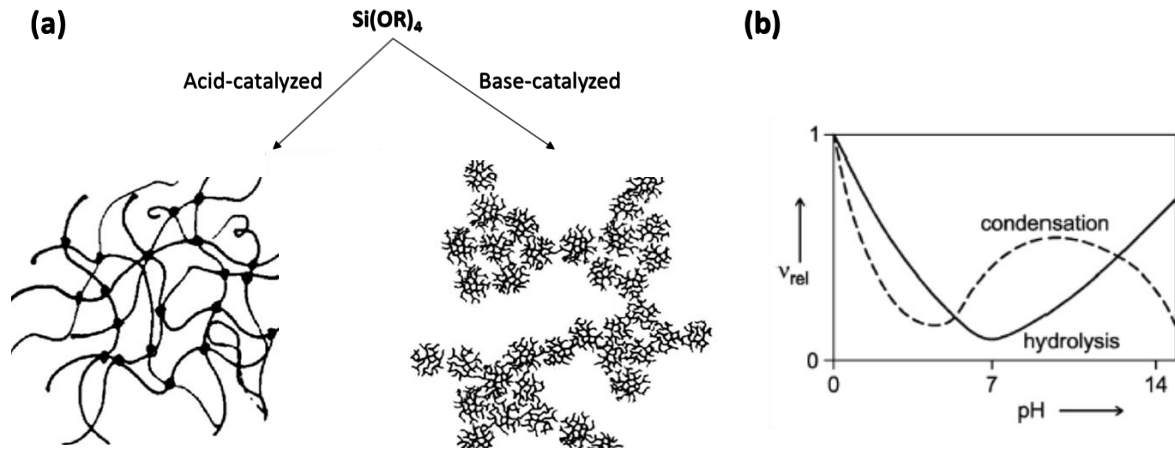
Figure 1. 10. (a) Typical structures from acid and base catalyzed sols 135 and (b) Dependence of relative rates of hydrolysis and condensation on pH 134
