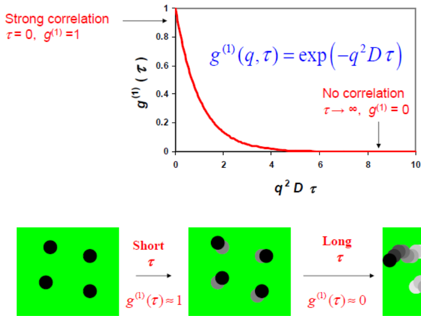
Figure A2.3. Different correlator conditions 2
