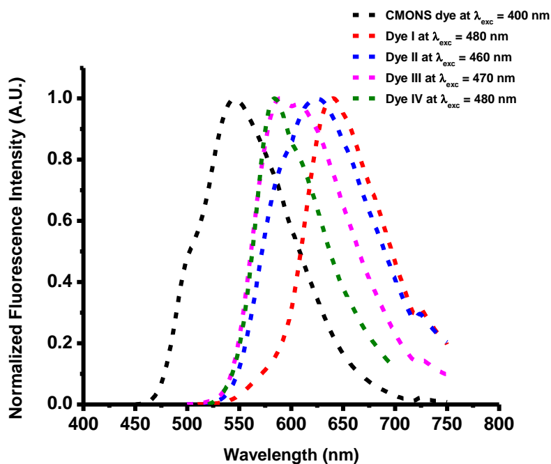
Figure 2. 23. Fluorescence spectra of organic dyes as microcrystals
