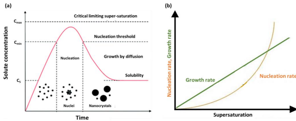
Figure 1. 12. (a) LaMer diagram for the nucleation and growth of nanocrystals. 139 (b) Dependence of nucleation and growth rate of crystallization on supersaturation 140
