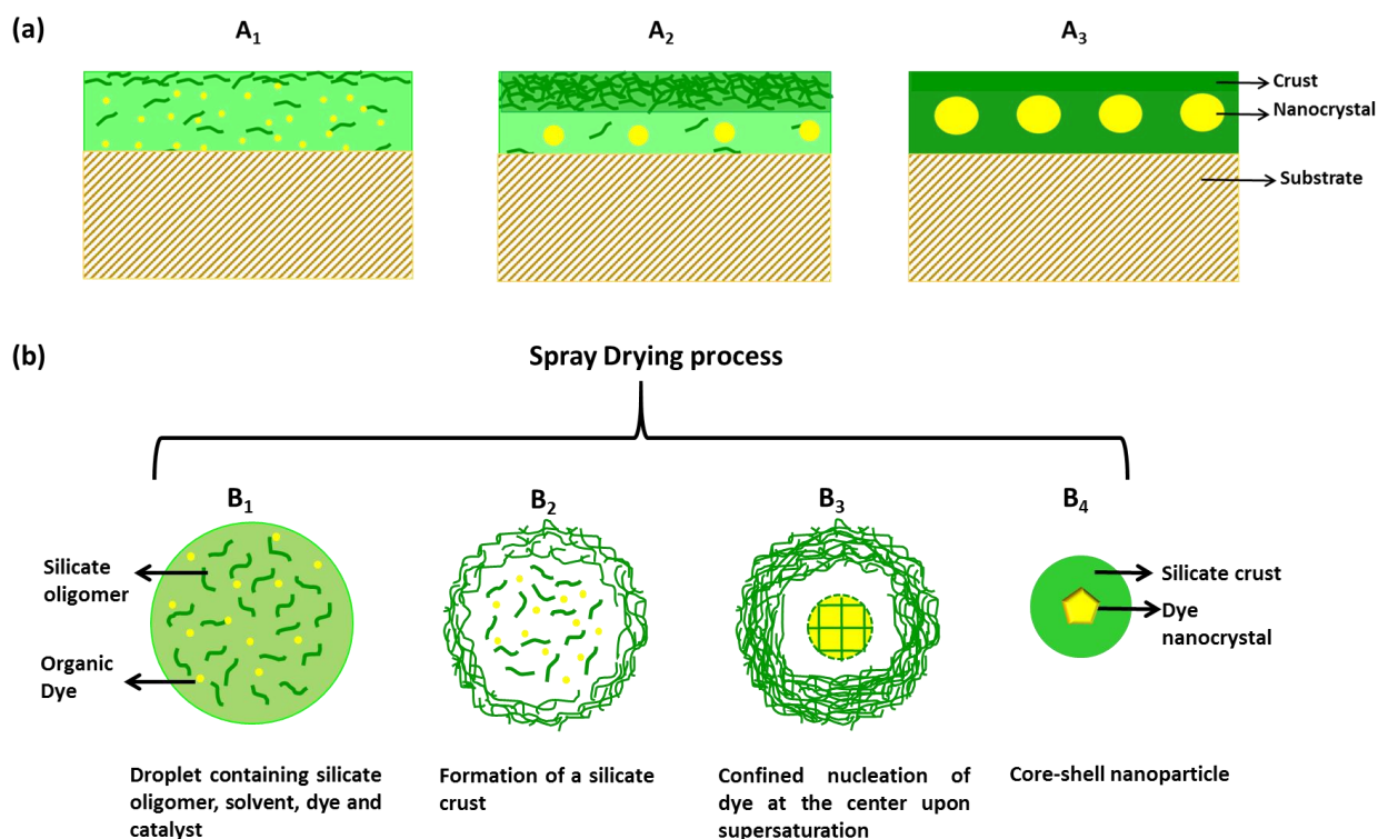
Figure 1. 13. Scheme illustrating the principle behind the formation of (a) buried nanocrystals in thin films by spin coating and (b) core-shell NPs by spray-drying
