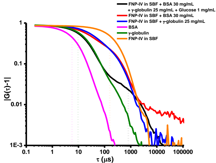
Figure 3. 32. Autocorrelation data corresponding to FNP-IV in SBF at 37 °C + BSA (30 mg/mL) + \gamma -globulin (25 mg/mL) + Glucose (1 mg/mL) at 37 °C
