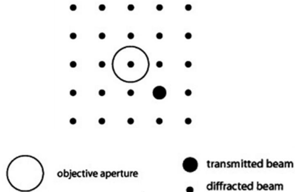
Figure A1.4. Dark-field observation method 1
