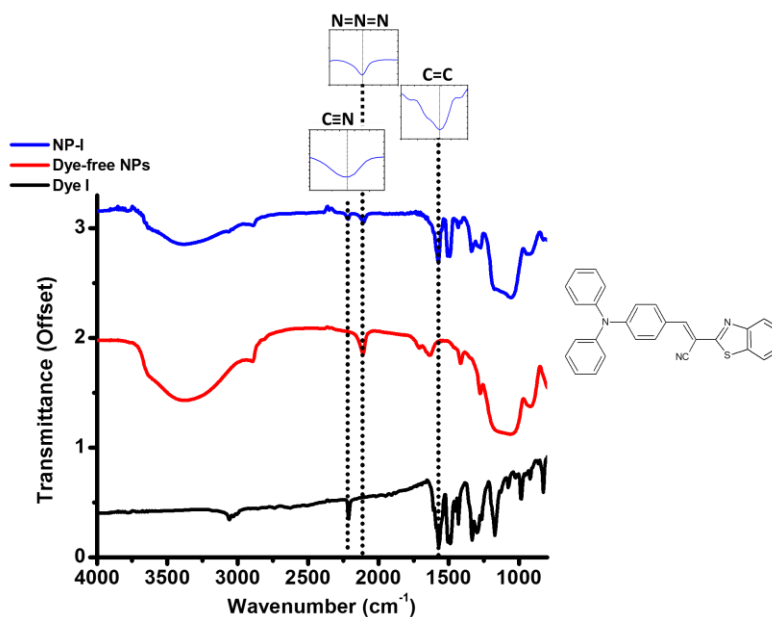
Figure 2. 13. IR spectra of NP-I (blue) compared to dye-free NPs (red) and dye I (black)
