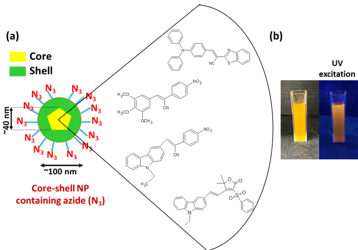
Figure 2. 1. (a) Schematic illustration of organic@silicate core-shell NPs and (b) core-shell NP suspension under UV excitation
