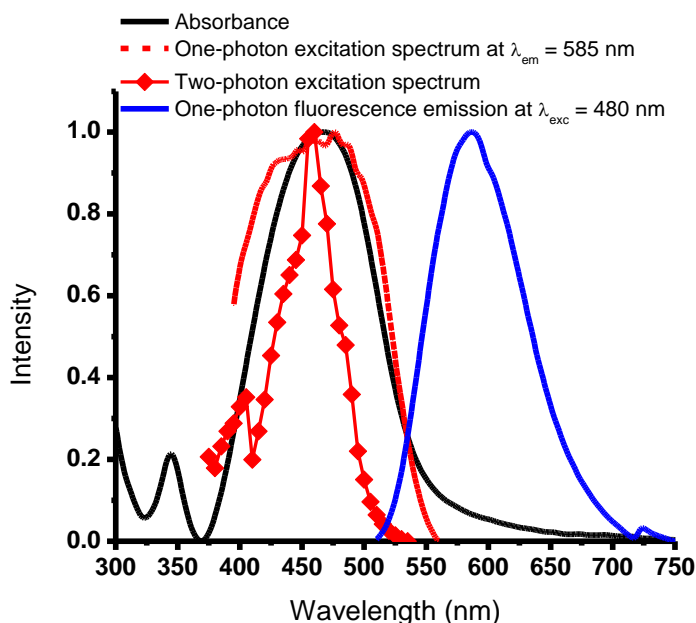
Figure 2. 29. Absorbance (black), one-photon (red) and two-photon excitation spectra (red symbol, raw data) and emission spectra (blue) of NP-IV
