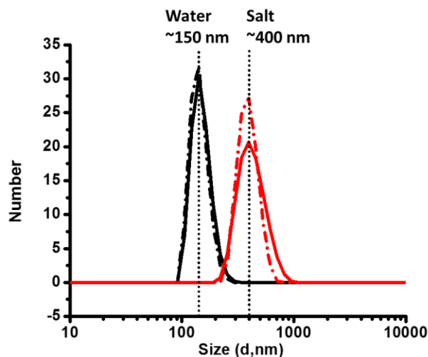
Figure 3. 10. Size distribution of NPs (NP-IV) in water (black) and 0.9 %wt salt solution (red) measured at 25 °C (solid line) and 37 °C (dotted line), pH 7.4
