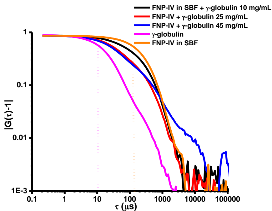
Figure 3. 29. Autocorrelation data corresponding to FNP-IV in SBF at 37 °C with different concentrations of \gamma -globulin.
