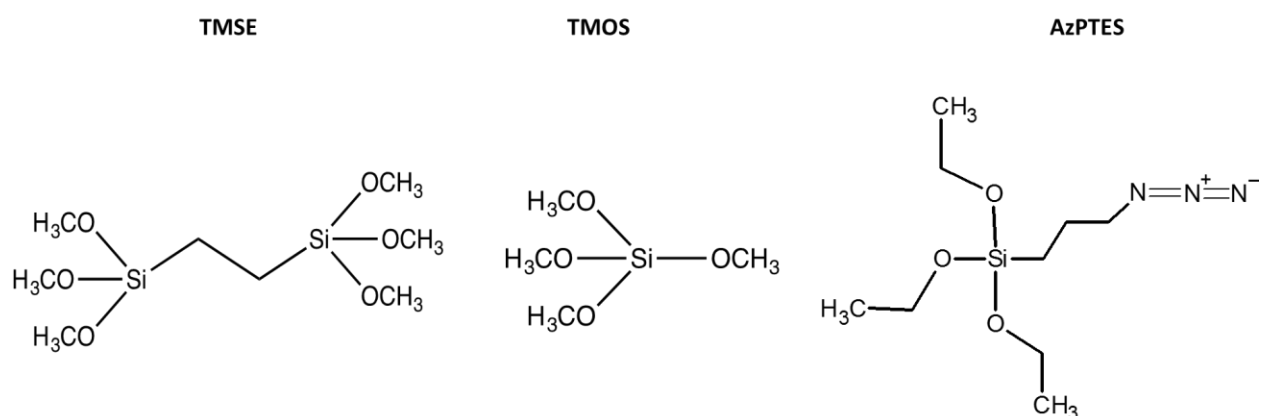
Figure 2. 2. Chemical structure of TMSE, TMOS and AzPTES.
