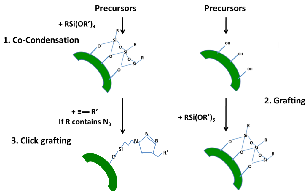
Figure 3. 11. Strategies for introduction of functional groups on the NPs
