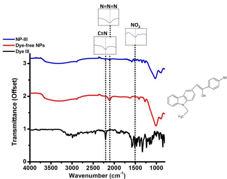
Figure 2. 15. IR spectra of NP-III (blue) compared to dye-free NPs (red) and dye III (black)
