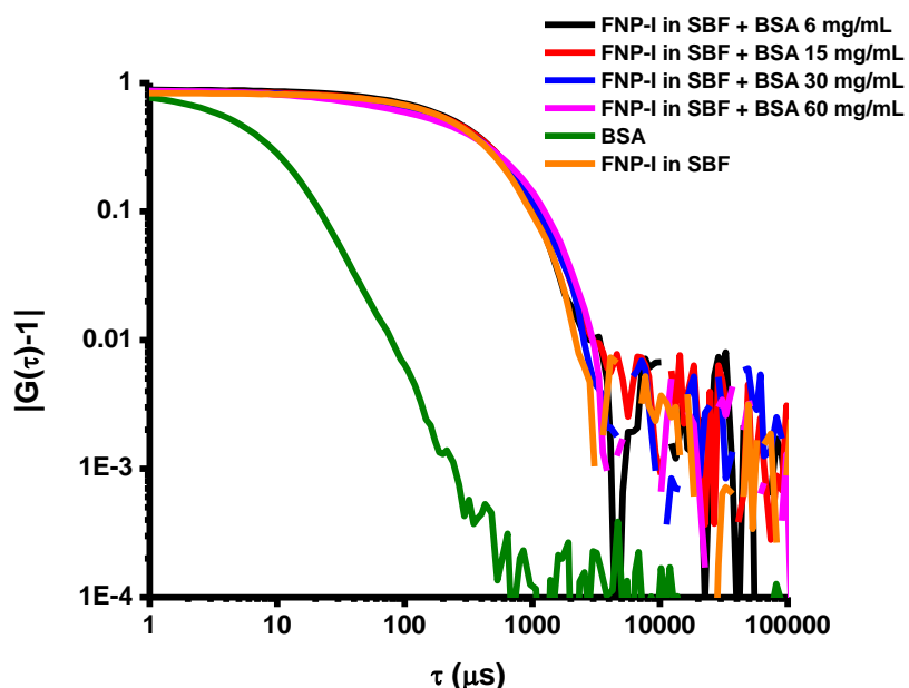
Figure 3. 25. Autocorrelation data corresponding to FNP-I in SBF with varying concentrations of BSA at 37 °C.
