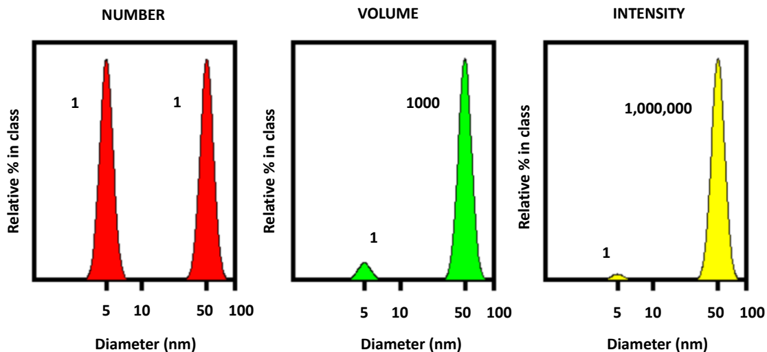
Figure A2.5. Number, volume and intensity distributions of a bimodal mixture of 10 and 100 nm particles 1
