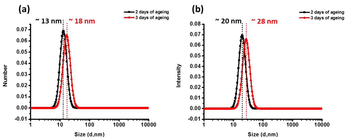
Figure 2. 8. DLS of sol prepared using protocol B (a) Number distribution and (b) Intensity distribution, at different stages of ageing, 2 days (black curve) and 3 days (red curve)
