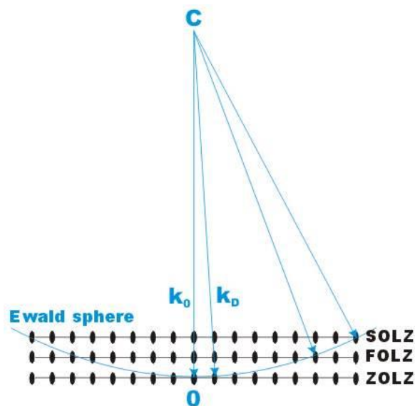
Figure A1.2. Ewald Sphere with point O is the origin of reciprocal lattice, k_0 is the wave vector of the incident wave, k_D is the wave vector of a diffracted wave, ZOLZ is Zero Order Laue Zone and FOLZ(SOLZ) is First (Second) Order Laue Zone 3
