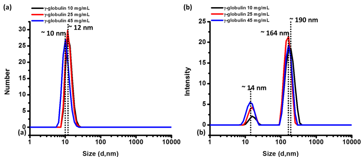
Figure 3. 27. (a) Number and (b) Intensity distribution of FNP-I in SBF at 37 °C with different concentrations of \gamma -globulin.
