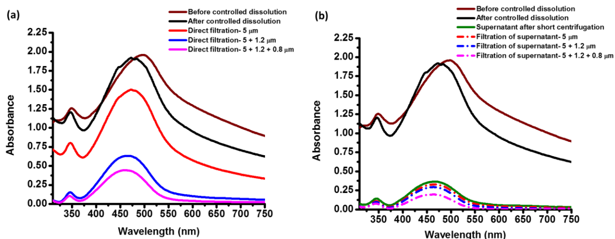
Figure 3. 8. Absorbance of the NPs (NP-IV) at each step of treatment for (a) Strategy B and (b) Strategy C
