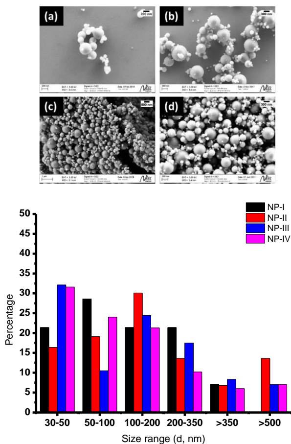
Figure 2. 11. Size distribution of core-shell NPs
