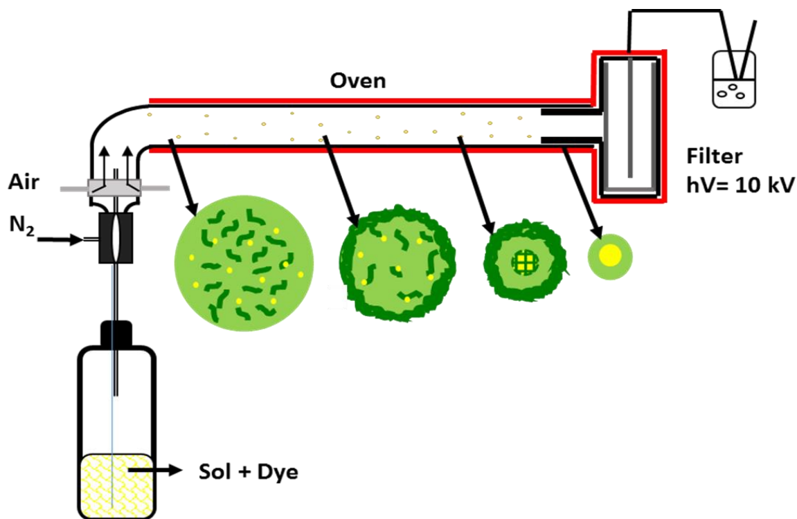
Figure 2. 3. Scheme of the home-built spray-drying reactor
