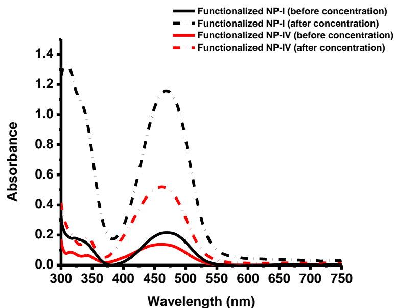
Figure 3. 18. Absorbance of functionalized NP-I (black) and NP-IV (red) before (solid) and after (dotted) concentration.
