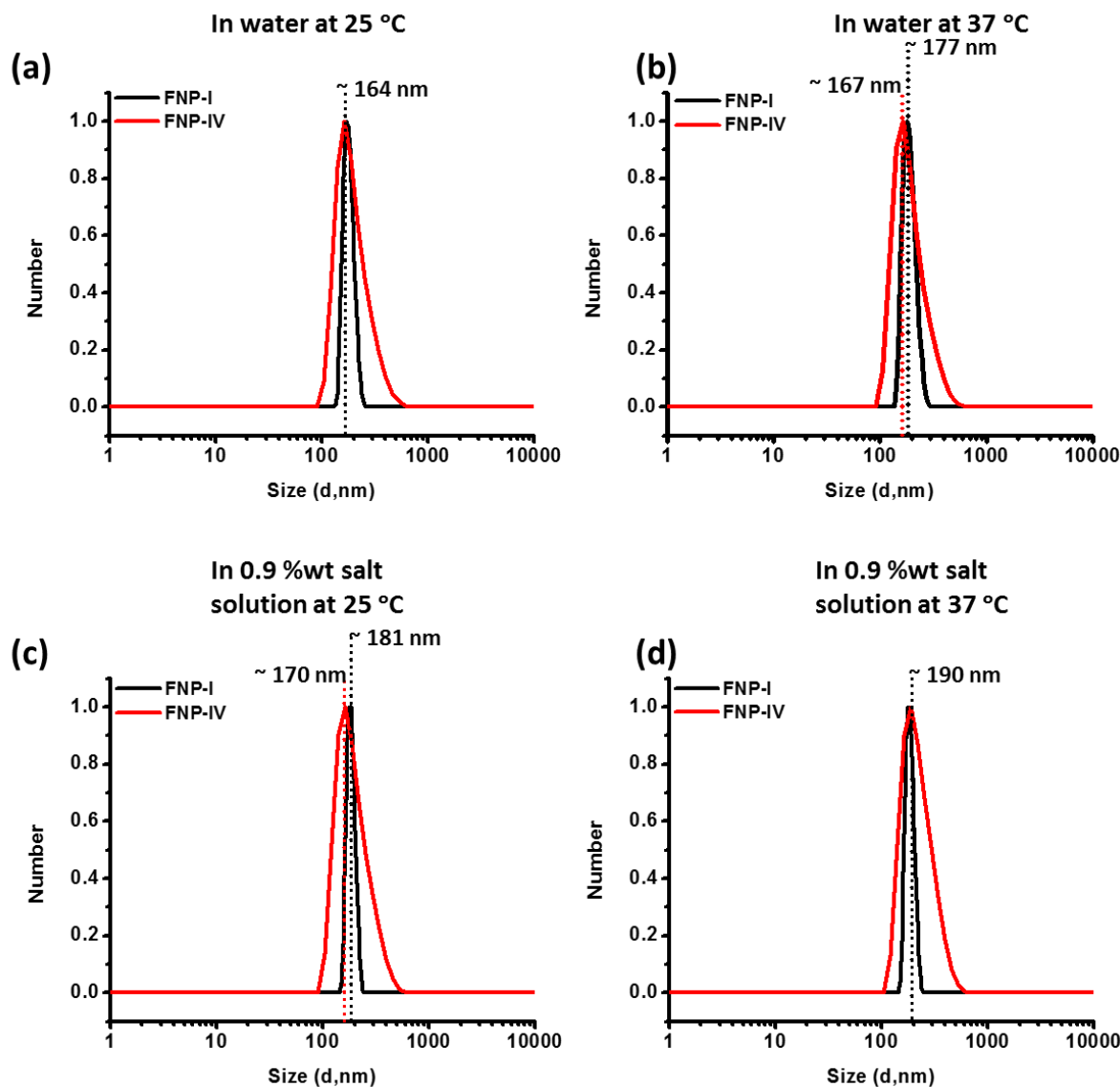
Figure 3. 19. Size distribution of LCPPEG-functionalized NP-I (Black) and NP-IV (red) in (a) water at 25 °C, (b) in water at 37 °C, (iii) in 0.9 %wt salt solution at 25 °C and (iv) in 0.9 %wt salt solution at 37 °C.
