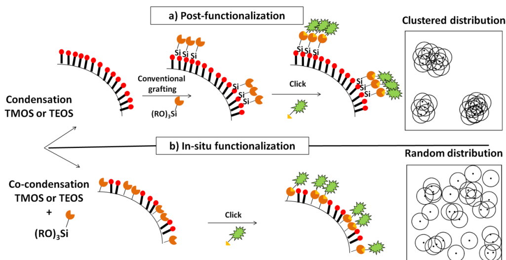
Figure 1. 20. Difference between (a) conventional grafting and (b) co-condensation methods with their corresponding graphical theoretical distribution (insets). 211
