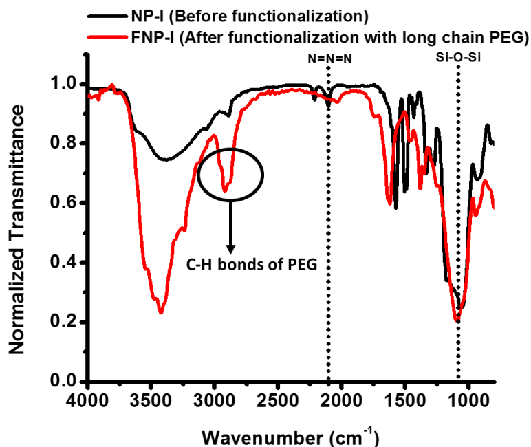
Figure 3. 15. IR spectrum of NP-I before and after functionalization with long-chain linear PEG ( M_n = 5000 )
