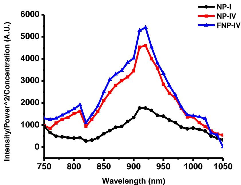
Figure 2. 27. Two-photon excitation spectra of NP-I , NP-IV and FNP-IV (raw data)
