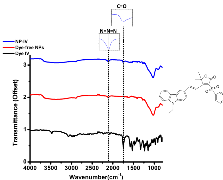
Figure 2. 16. IR spectra of NP-IV (blue) compared to dye-free NPs (red) and dye IV (black)
