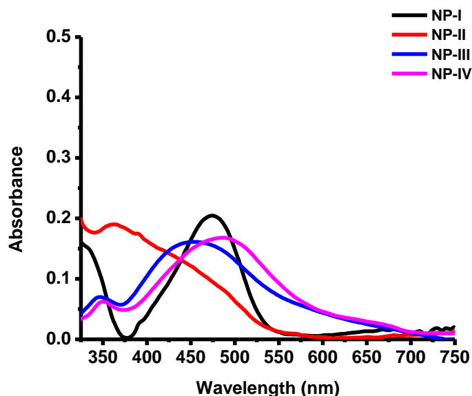
Figure 2. 21. Absorbance spectra of the core-shell NPs after basic treatment
