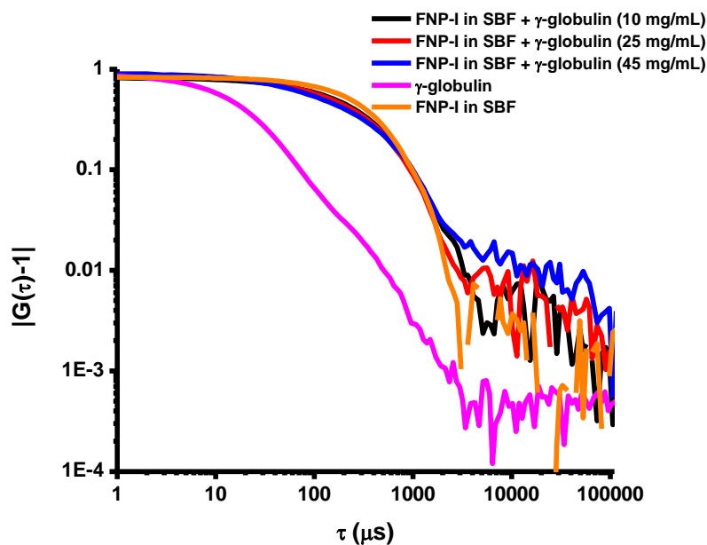
Figure 3. 28. Autocorrelation data corresponding to FNP-I in SBF at 37 °C with different concentrations of \gamma -globulin.
