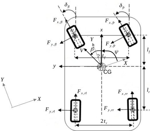
Figure 1.5 – Vehicle lateral/longitudinal model
