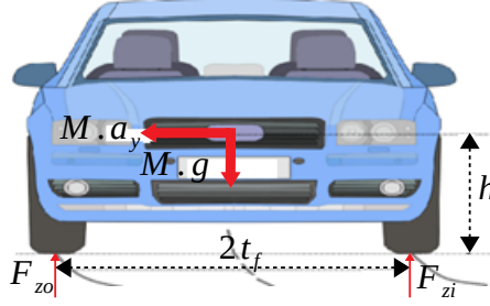
Figure 3.2 – Static rollover
