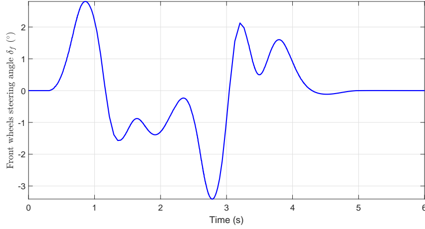
Figure 1.12 – Steering angle
