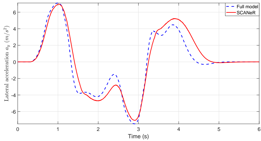
Figure 1.14 – Lateral acceleration
