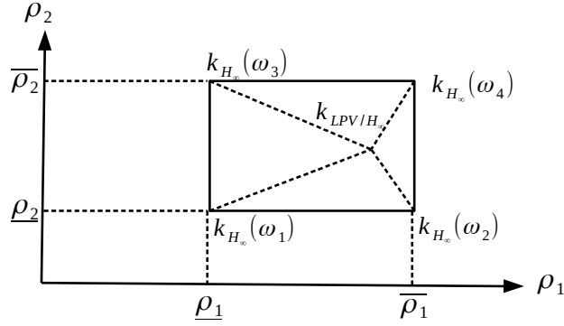
Figure 2.5 – Polytopic LPV/\mathcal{H}_{\infty} controller
