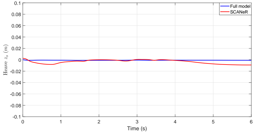
Figure 1.17 – Heave
