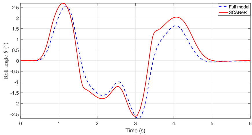
Figure 1.15 – Roll angle
