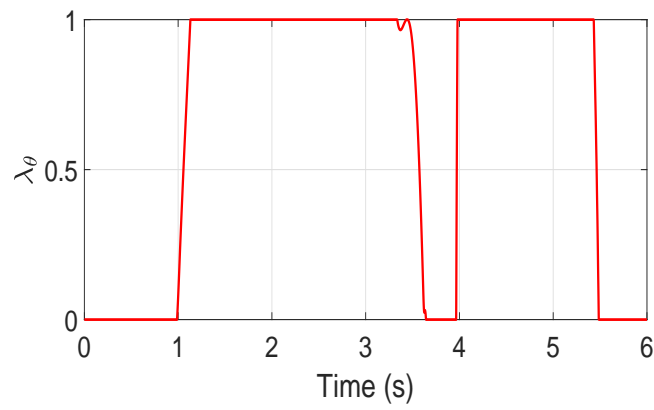
Figure 5.29 – Load transfer ratio LTR and scheduling gains (Fishhook test)
