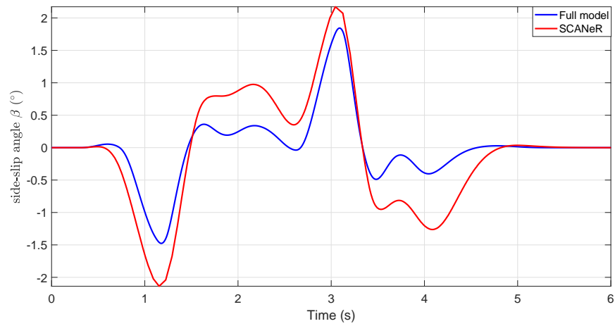
Figure 1.22 – Side-slip angle
