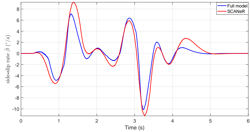
Figure 1.23 – Side-slip rate
