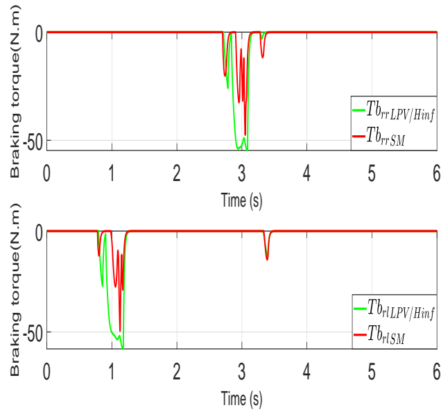
Figure 5.23 – Braking comparison (DLC test)
