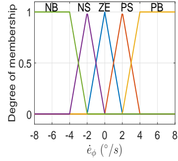
Figure 4.7 – Fuzzy sets of the input \dot{e}_\phi
