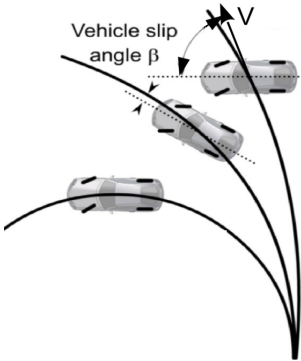
Figure 1.6 – Vehicle side-slip
