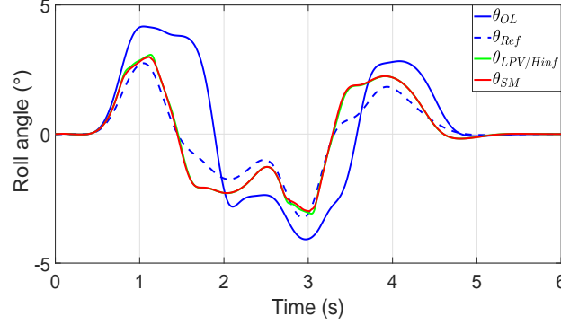
Figure 5.19 – Roll angle comparison (DLC test)
