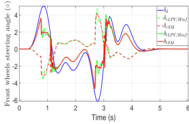
Figure 5.22 – Steering angle comparison (DLC test)
