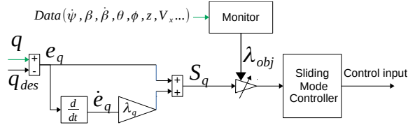
Figure 4.4 – Scheduled controller
