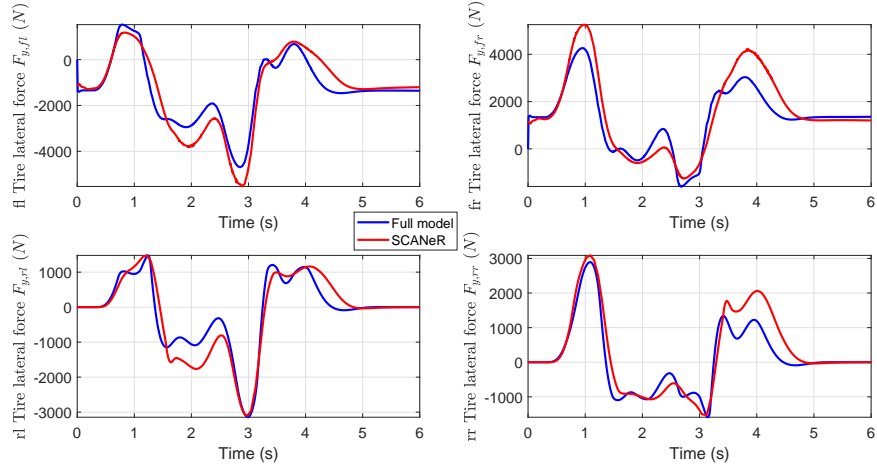
Figure 1.19 – Tire's lateral forces
