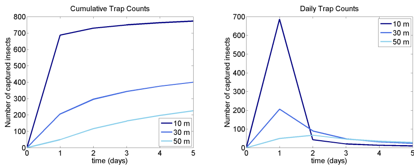
Figure 4.17: Cumulative (left) and daily (right) trap counts obtained for a release of 1000 insects at distances of 10, 30 and 50 meters from the centre of the trap, using c = c_{stat} .
