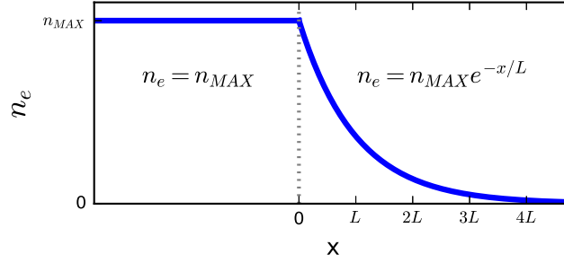
Figure 1.11: Preplasma exponential density profile given by equation 1.64
