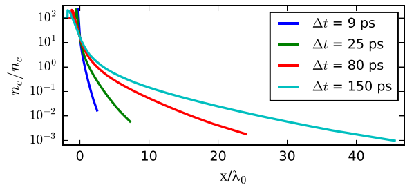
FIG. 4. Results from 1D hydrodynamic simulations. Normalized electron density n_e/n_c as a function of position x for different delays after a prepulse with a fluence of 50 \text{ J/cm}^2 ionizes a solid fused-silica target. x = 0 is the initial solid-vacuum interface position. n_c = m_e \epsilon_0 \omega_0^2 / e^2 is the critical density above which the laser cannot propagate. \epsilon_0 is the vacuum permittivity.
