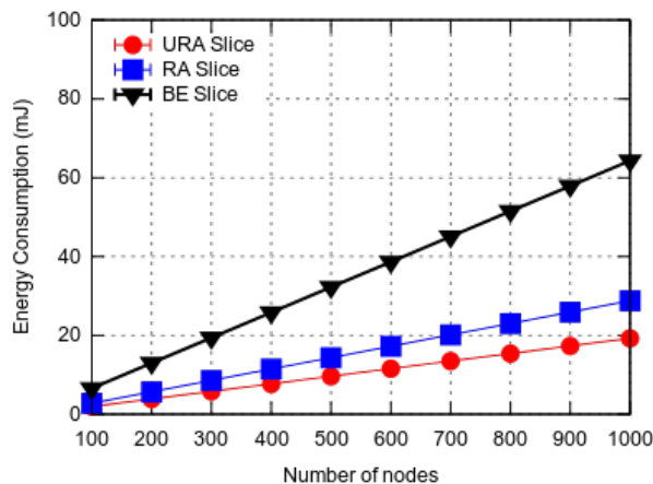
Figure. II.9: Mean energy consumption variation
