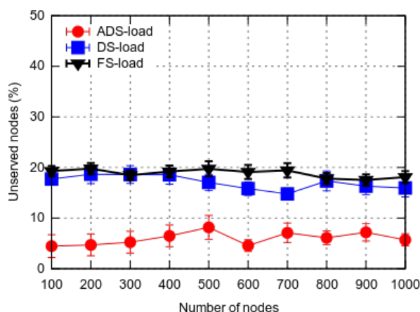
Figure. II.7: Percentage of unserved nodes
