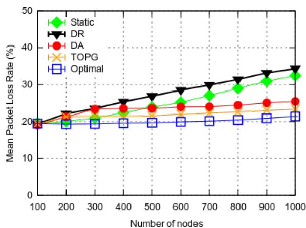
Figure. III.7: PLR variation
