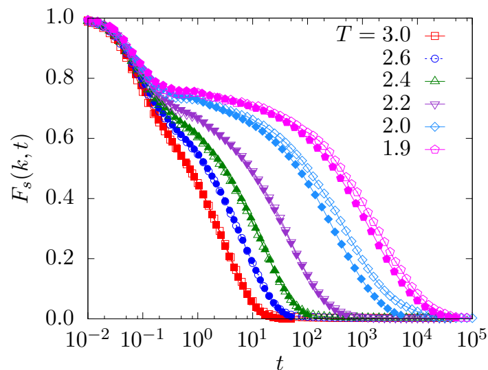
Figure 11: Self-intermediate scattering function F_s(k, t) calculated for the binary system with \Delta\sigma = 0.2 using the continuous time (open symbols) swap and hybrid (filled symbols) algorithms at different temperatures.
