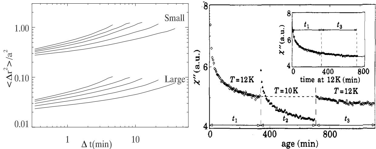
Figure 1.4 | Nonequilibrium dynamics in glassy materials. Left: Aging in the mean-squared displacement of large and small particles in a binary colloidal glass [34]. The age of the glass increases from top to bottom. Right: Aging, rejuvenation, and memory effects in the dynamic susceptibility of a disordered magnet subjected to a temperature cycle, from Ref. [35].
