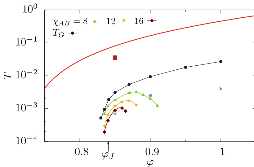
Figure 5: Ergodicity breaking versus collective dynamics. Glasses prepared at (\varphi_g, T_g) = (0.85, 0.0353) (red square), below the computer glass transition (red line), are followed in the \varphi - T phase diagram. We indicate the iso- \chi_{AB}(t_w = 10^4) lines at which the dynamical susceptibility reaches 8, 12 and 16. The dynamics is increasingly collective in the dome delineated by these lines. Ergodicity breaking, observed at the line T_G(\varphi) , may be due to collective defects (low \varphi ), or not (high \varphi ). The jamming transition \varphi_J of the glass, indicated by an arrow, takes place under the dome where dynamics is collective. We show in Fig. 6 the microscopic dynamics after bringing the glass (red square) to three state points (blue stars) at which ergodicity is lost, and the dynamics is more or less collective (labelled a, b, c from left to right).
