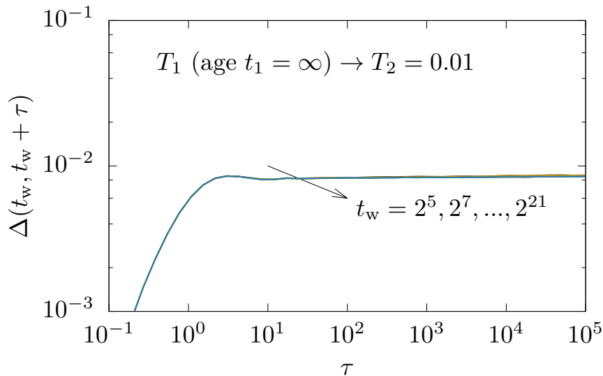
Figure 5: No rejuvenation if T_2 is too large. Here, glasses aged for t_1 = \infty at T_1 = 0.0353 are cooled down to T_2 = 0.01 .
