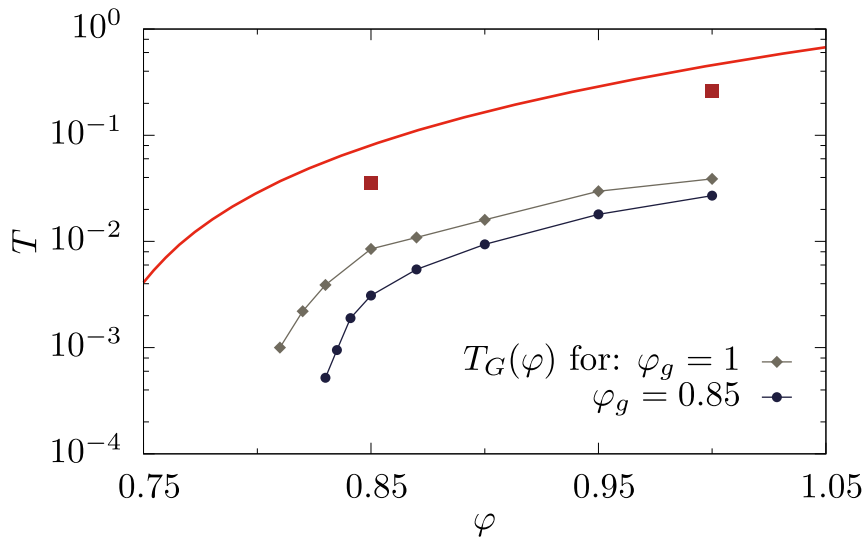
Figure 3: Loss of ergodicity for various glasses. Glasses are prepared in equilibrium conditions with the swap method at (\varphi_g, T_g) = (0.85, 0.0353) and (1, 0.26) (red squares), below the computer glass transition (red line). The glasses are rapidly brought to another state point (\varphi, T) in the phase diagram. We compare the long-time limit of the mean-squared displacement and the mean-squared distance between clones of the glass at the new state point. Both values are equal around (\varphi_g, T_g) where the glass basin is sampled ergodically. Ergodicity inside the glass is broken below T_G(\varphi) . The ergodicity breaking line T_G(\varphi) depends on glass preparation, encoded in (\varphi_g, T_g) . We find that the lines T_G(\varphi) for different glass preparations have the same qualitative behavior.
