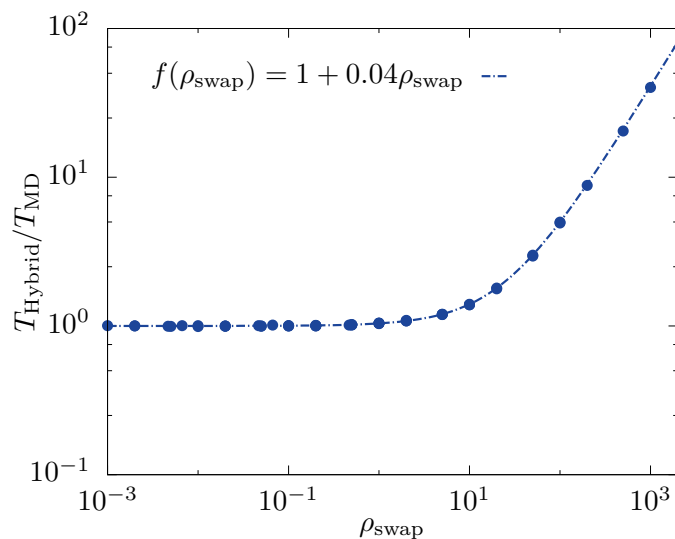
Figure 4: Ratio of the CPU time T_{\text{Hybrid}} of Hybrid simulations compared to the CPU time of standard molecular dynamics T_{\text{MD}} , both running for the same total MD length. The trivial limits of T_{\text{Hybrid}}/T_{\text{MD}} at small and large \rho_{\text{swap}} are well captured by a simple empirical fitting function shown with a dashed line.
