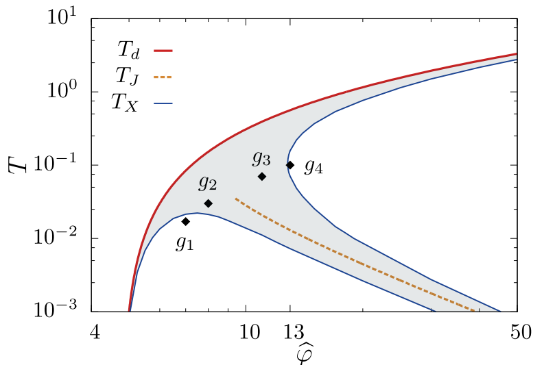
Figure 6: Equilibrium mean-field phase diagram of harmonic spheres, as in Fig. 2. We add the transition lines T_X (thin lines) which delimit the glasses that become unstable upon cooling (shaded region), such as g_2 , and g_3 , or not, as for g_1 and g_4 .
