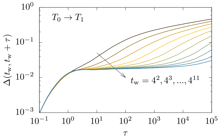
Figure 3: Aging of the mean-squared displacement after a quench from the liquid T_0 = 0.36 to the glass phase T_1 = 0.0353 . Each curve corresponds to a given waiting time t_w after the quench, and reveals a slower motion in older systems.
