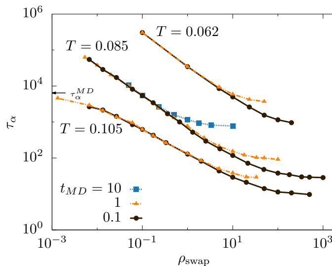
Figure 3: Relaxation time as a function of \rho_{\text{swap}} for three selected temperatures: T = 0.105, 0.085, 0.062 . At fixed temperature, each data set corresponds to a given duration of the MD blocks, t_{\text{MD}} = 0.1, 1, 10 , and each single point to one value of n_{\text{swap}} . The arrow labeled \tau_\alpha^{\text{MD}} indicates the relaxation time of the liquid at T = 0.105 for ordinary MD simulations; this time cannot be directly measured for the two lowest temperatures.
