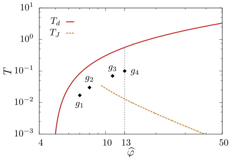
Figure 2: Equilibrium mean-field phase diagram for harmonic spheres. The dynamical transition T_d (red line) separates liquids that flow (above) from dynamically arrested ones (below). We select equilibrium glasses in the dynamically arrested region, for example g_1, \dots, g_4 , and follow each glass adiabatically in temperature and packing fraction. The corresponding state-following phase diagrams are presented Fig. 5(a-d). Glasses equilibrated above the line T_J (dashed line) are jammed once minimized to T = 0 , while glasses selected below the line are unjammed at T = 0 . The state-following phase diagrams of glasses prepared at \hat{\varphi}_g = 13 (vertical dashed line) are presented in Figs. 3-4.
