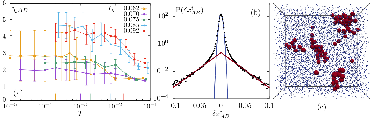
Figure 3: (a): The susceptibility \chi_{AB} for different T_g raises mildly above the floor level (dashed line) across T^* (vertical segments). The error bars are computed using the jackknife method. (b): The van-Hove function of relative displacements has a narrow Gaussian core of width given by \Delta^\infty (solid blue), and exponential tails (solid red) at T_g = 0.062 and T = 10^{-4} . (c) Corresponding snapshot with N = 12000 showing the few particles having displacements outside the Gaussian range (red spheres) among a majority of particles undergoing small amplitude Gaussian vibrations (blue dots).
