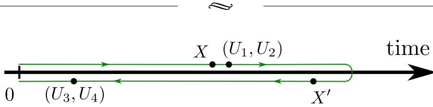
Figure 2.3: Same contribution as in Fig. 2.2 after expending the interaction Hamiltonian, and using the Keldysh point notations.
