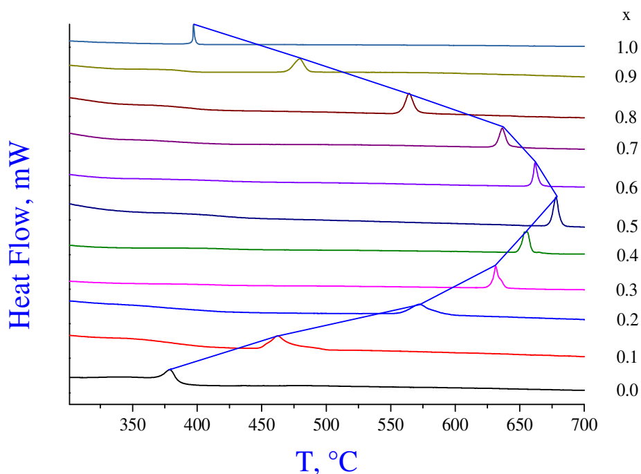
Figure IV-3: The characterization of crystalline transition temperatures by thermal analysis (DTA) of Zr_xTi_{1-x}O_2 nanoparticles with different elemental compositions 0 \leq x \leq 1 .
