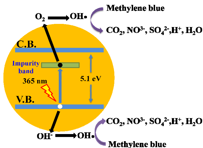
Figure I-24: The proposed mechanism of methylene blue photodegradation by ZrO 2 [125].
