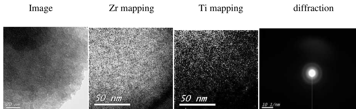
Figure annex 6: Amorphous of oxo- Zr_{0.6}Ti_{0.4}O_2 of mapping elemental and diffraction images from TEM.
