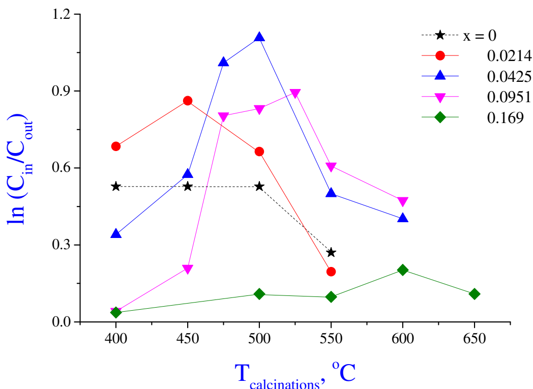
Figure V-11: Photocatalytic activity of Zr_xTi_{1-x}O_2 ( 0 \leq x \leq 0.2 ) for ethylene decomposition ( C_{in}=120 ppm). The photocatalysts were calcinated at temperatures between 400 and 650 °C according to table IV -1.
