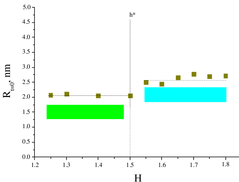
Figure III-12: Initial radius of mixed ZTOA ( R_0 ) for different hydrolysis ratios H ( C_{pr} = 0.292 M, x = 0.5 , T = 20 °C, Re \approx 6000 ).
