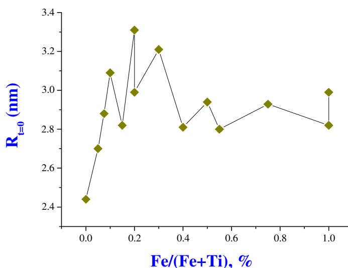
Figure I-16: Initial particle sizes of iron doped TOA nanoparticles versus doping ratios ( C_{Ti} = 0.146 \text{ mol/L} , H = 2.5 , Re = 4500 ) [101].
