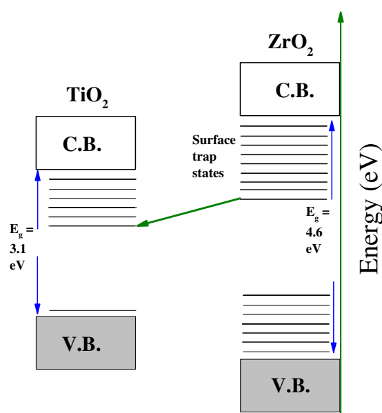
Figure I-25: The diagram of electron in surface trap states of ZrO_2 conduction band crossed section into TiO_2 conduction band [57].
