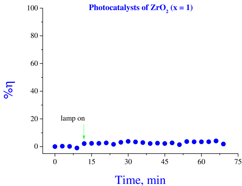
Figure annex 10: Photocatalytic activity of composite ZrO_2 : T_{calcinations} = 500 °C, C_{Ethylene} = 120 ppm, RL = 15 cm (3.78 g), \lambda = 362 \pm 11 nm, flow rate = 60:40 mL/min (air:ET).
