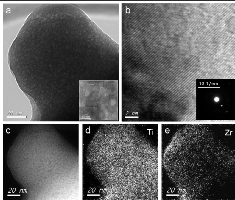
Figure IV-7: TEM image (a, b), electron absorption (c), elemental mapping of Ti (d) and Zr (e) and electron diffraction (inset b) of Zr_{0.5}Ti_{0.5}O_2 nanoparticles.
