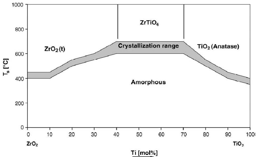
Figure I-3: Phase domains and transformation temperature of mixed ZrO_2 - TiO_2 composite as function of TiO_2 and ZrO_2 composition [37].
