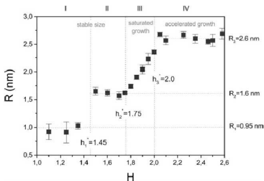
Figure I-14: Particle sizes of TOA at different hydrolysis ratios (TTIP = 0.146 mol/L, T = 20 °C) [102].
