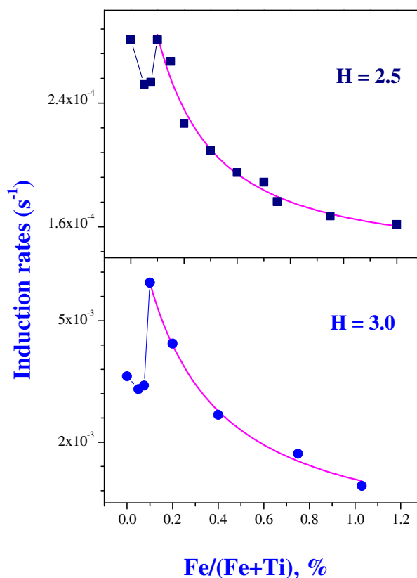
Figure I-15: Induction rate of iron doped titanium oxo-particles ( C_{\text{Ti}} = 0.146 \text{ mol/L} , T = 20 \text{ }^\circ\text{C} , H = 2 and 3 and Re = 4500 ) [104].
