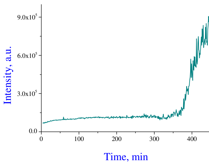
Figure III-9: The scattering intensity of TOA particles in isopropanol ( H = 1.8 , C_{\text{Ti}} = 0.292 mol/l, T = 20.0 °C, Re \approx 6000 ).
