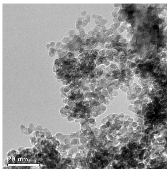
Figure I-19: TEM Image of ZOA nanoparticles obtained in the following experimental condition: C_{Zr} = 0.15 mol/L, H = 2.5 , T = 20 °C [105].
