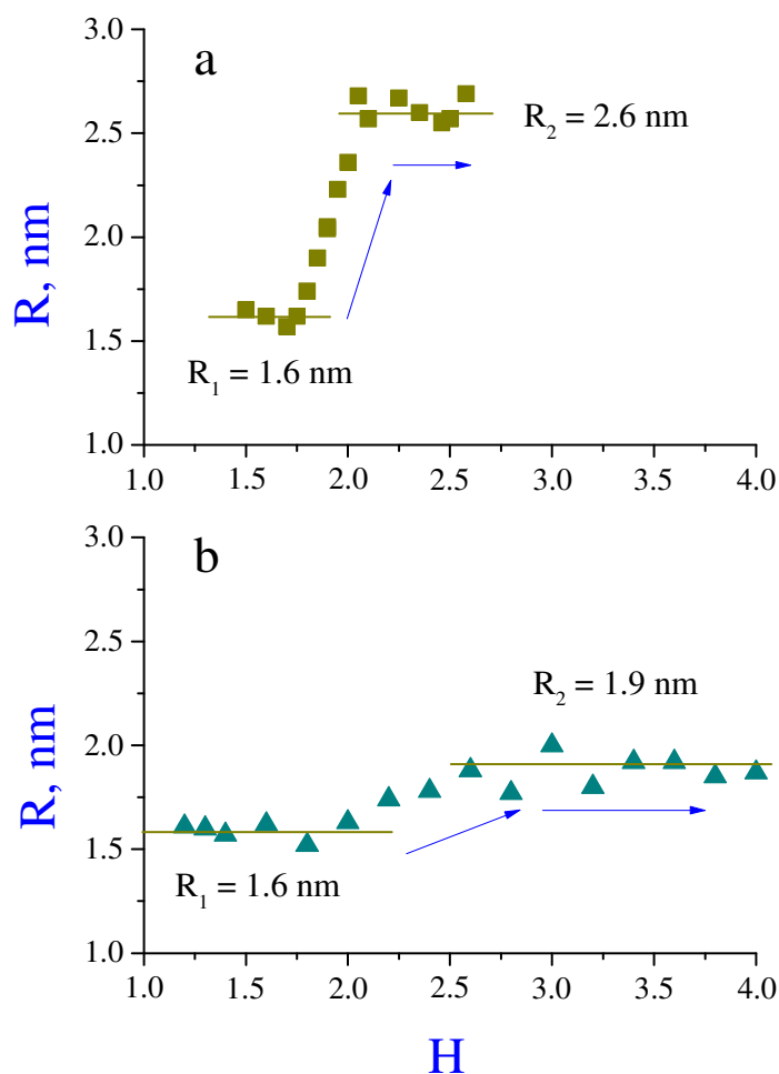
Figure III-7: Particles radius evolution with H in (a) isopropanol (b) n -propanol solvent ( C_{Ti} = 0.146 \text{ mol/l} , T = 20.0 \text{ }^\circ\text{C} , Re = 6000 ).
