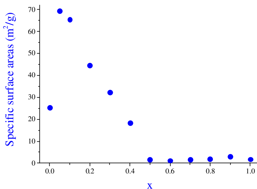
Figure IV-12: Specific surface areas (BET) of nanoparticulate Zr_xTi_{1-x}O_2 solids ( 0 \leq x \leq 1 ).
