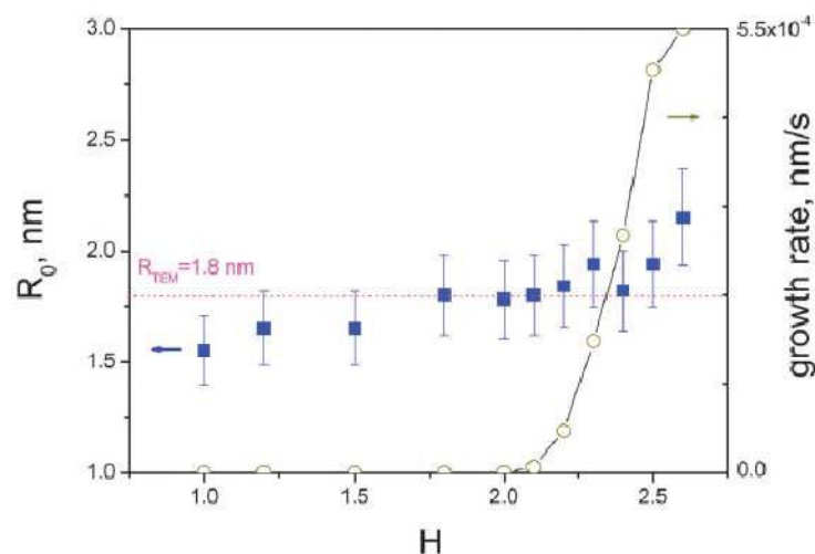
Figure I-18: Initial sizes of particle ( R_0 ) and slope of I(t) curves during the induction period of ZOA n -propanol sol-gel process for different hydrolysis ratios ( C_{Zr} = 0.15 mol/L, T = 20 °C) [105].
