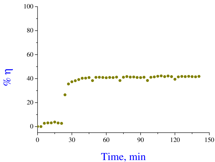
Figure annex 12: Photocatalytic activity of composite Zr_{0.04}Ti_{0.96}O_2 : T_{calcinations} = 500\text{ }^\circ\text{C} , C_{Ethylene} = 300\text{ ppm} and flow rate = 40:35 (air:ET), RL = 5\text{ cm} (1.29 g), \lambda = 362 \pm 11\text{ nm} .
