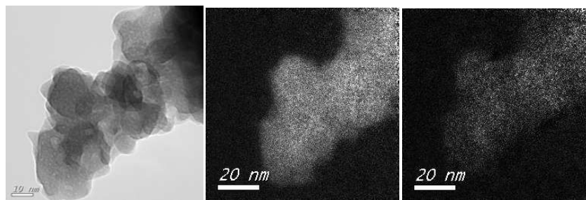
Figure annex 8: Amorphous of oxo- Zr_{0.7}Ti_{0.3}O_2 of mapping elemental images from TEM.
