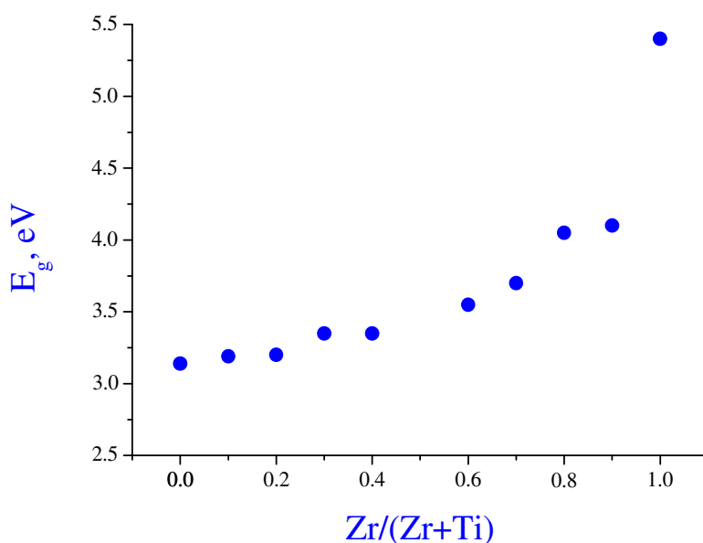
Figure IV-11: Band gaps of different compositions of composite Zr_xTi_{1-x}O_2 .
