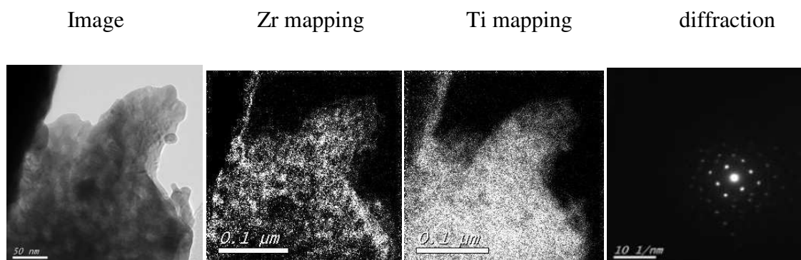
Figure annex 2: Crystalline of composite Zr_{0.3}Ti_{0.7}O_2 of mapping elemental and diffraction images from TEM.
