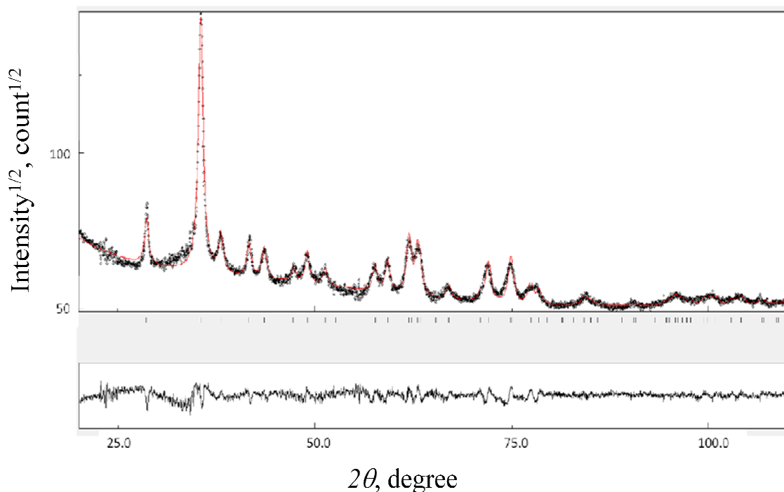
Figure IV-5: Least squares fit of XRD pattern of Zr_{0.5}Ti_{0.5}O_2 nanopowder with orthorhombic structure.
