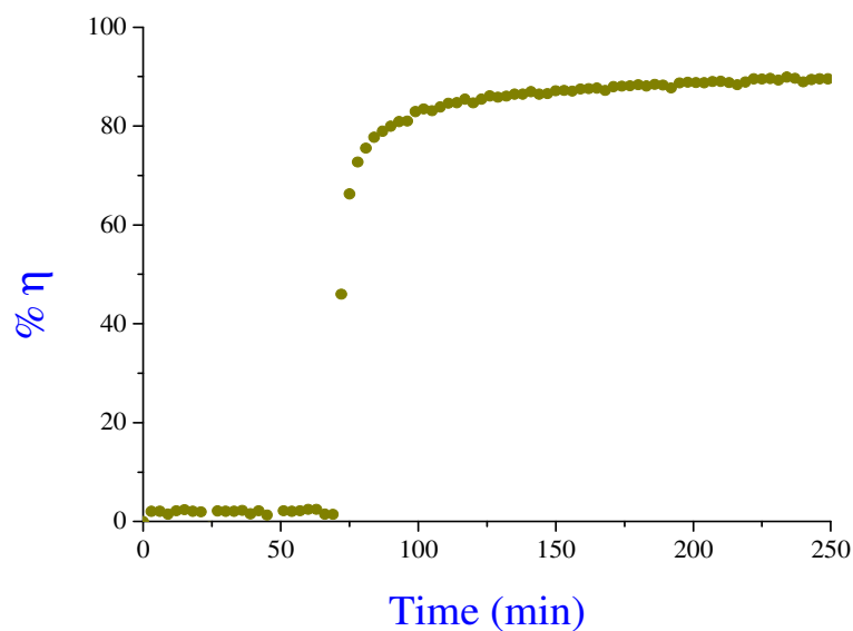
Figure annex 11: Photocatalytic activity of composite Zr_{0.04}Ti_{0.96}O_2 : T_{calcinations} = 500 °C, C_{Ethylene} = 60 ppm and flow rate = 40:35 (air:ET), RL = 5 cm (1.29 g), \lambda = 362 \pm 11 nm.
