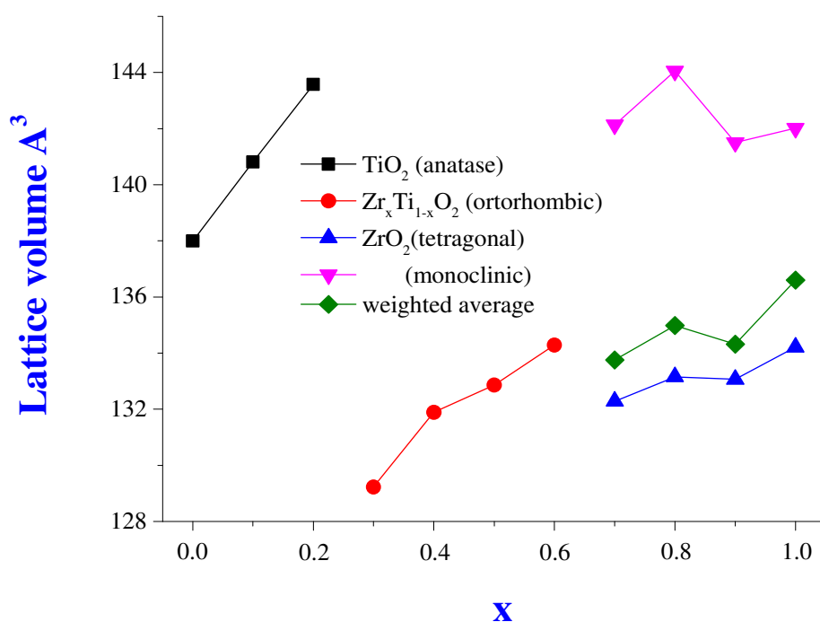
Figure IV-6: Lattice volumes ( A^3 ) in different phases and compositions of crystalline Zr_xTi_{1-x}O_2 nanoparticle. (The lattice volume of t-Zr_xTi_{1-x}O_2 were multiplied by 2 due to this compound containing two metal elements).
