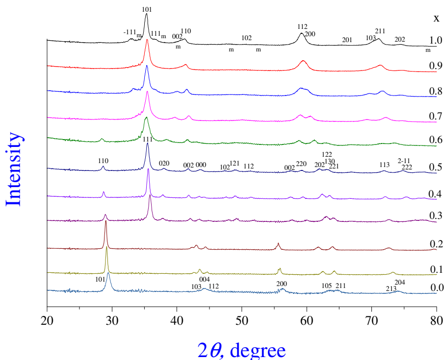
Figure IV-4: XRD patterns of Zr_xTi_{1-x}O_2 nanopowders with different elemental compositions 0 \leq x \leq 1 , heat treated at temperatures T_h(x) of the exothermic peaks in DTA curves. The peaks of anatase, orthorhombic and tetragonal / monoclinic phases are respectively indexed in diffractograms x=0 , x=0.5 and x=1 (peaks of monoclinic phase are complimentary labeled with m ; the very weak peaks are only labeled).
