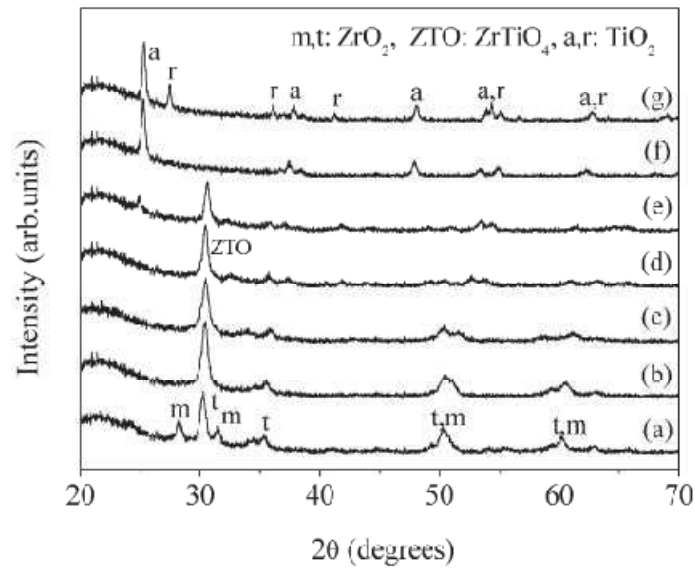
Figure I-4: X-ray patterns of mixed film samples after calcinations at 700 °C (a) ZrO_2 , (b) ZrTi91 , (c) ZrTi73 , (d) ZrTi55 , (e) ZrTi37 , (f) ZrTi19 and (g) TiO_2 [48].
