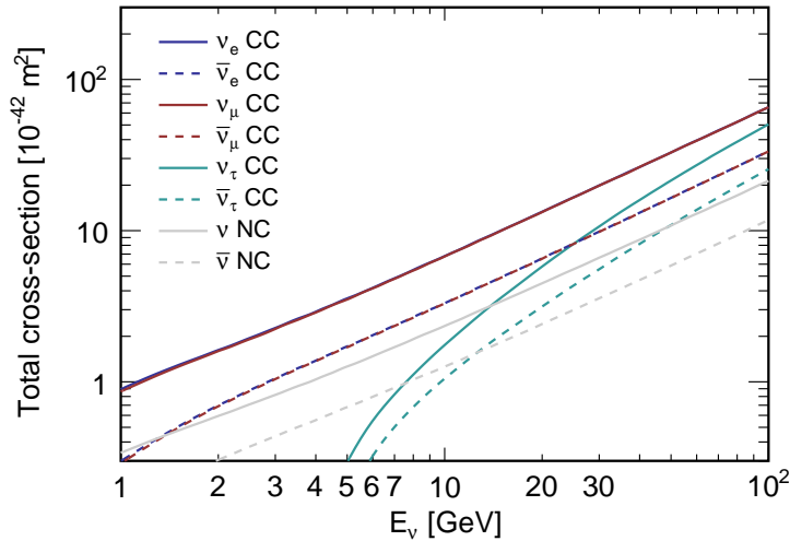
Figure 2.5: Inclusive cross-section per nucleon for the interaction of neutrinos with a water target, as predicted by the GENIE Monte Carlo generator [97, 98] (see Chap. 4 for details).
