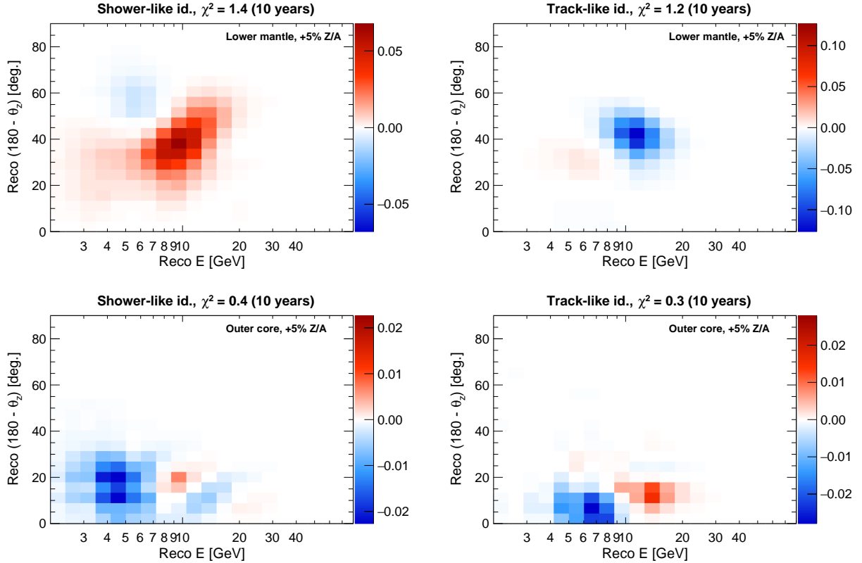
Figure 9.6: Expected signal in the final track-like and cascade-like samples, shown as maps of the \chi_s^2 indicator. Mind that the energy range shown here is extended with respect to Fig. 9.5. The Z/A factor is varied by +5% separately in each layer (lower mantle in top panel, outer core in bottom panel). 10 years of exposure with a full detector, true NH and reference oscillation parameters are assumed, and the detector response is applied using the uncorrelated smearing method.
