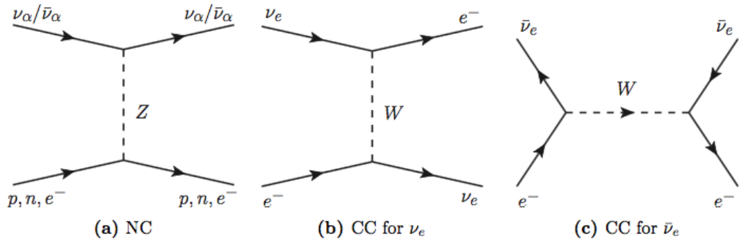
Figure 1.12: Elastic scattering processes between anti(neutrinos) and ordinary matter ( n, p, e^- ).
