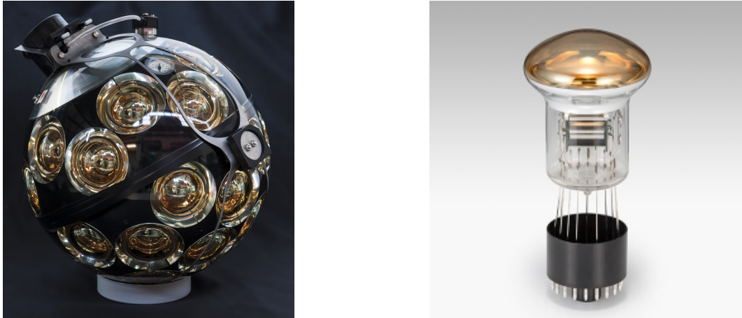
Figure 3.2: Photographs of a KM3NeT DOM (left) and Hamamatsu R12199-02 photomultiplier tube (right). In the DOM, the visible part of the individual PMTs comprise the photocathode areas, circled by the silver-coloured reflector rings.
