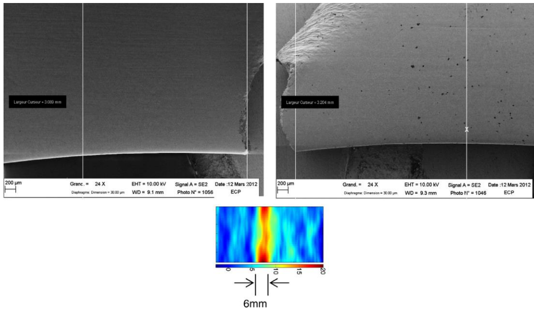
Figure 1.34 Correlation between intrinsic dissipation and PSB formation on armco iron specimen.
