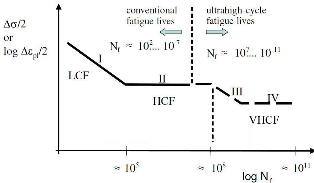
Figure 1 Schematic figure of S-N curve.(Mughrabi, 2006)
