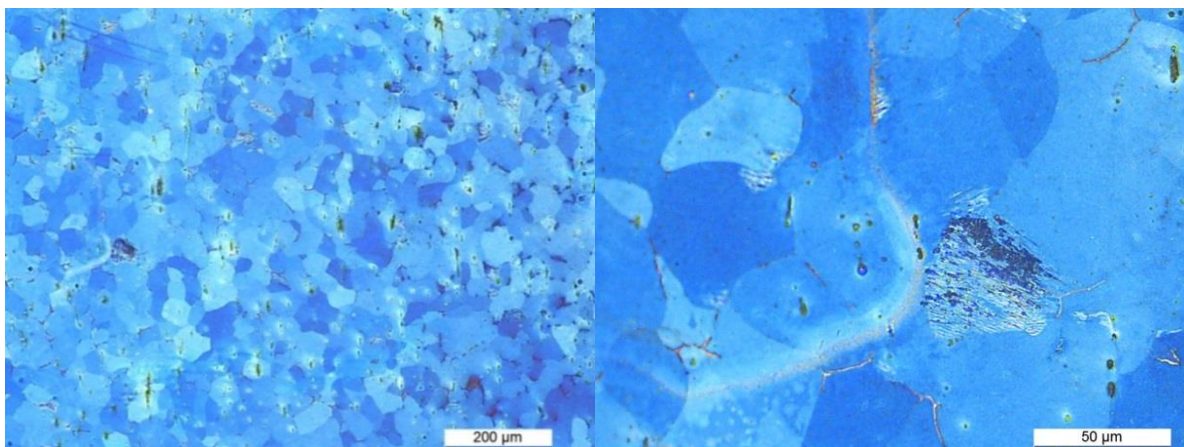
Figure 4.10 Surface of C12 steel at 194 MPa after 3 \times 10^9 cycles, observed by desk type optical microscope.
