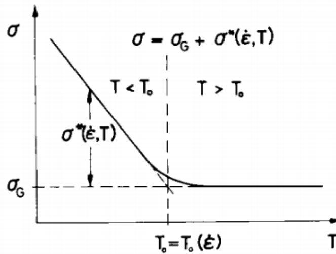
Figure 3.20 Schematic diagram of flow stress in BCC metals versus temperature. (Mughrabi, 2009)
