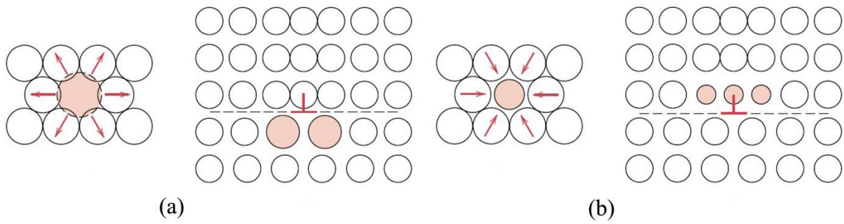
Figure 1.8 Representation of strains imposed on host atoms by (a) a larger substitutional atoms and the corresponding possible locations of foreign atoms beside an edge dislocation such that there is partial cancellation of lattice strains; (b) the case of a smaller substitutional atom. (Callister, 2015)
