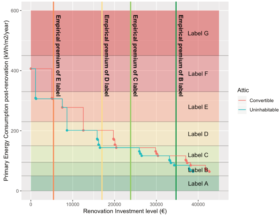
Figure 2.41: Renovation of a typical house built before 1974
