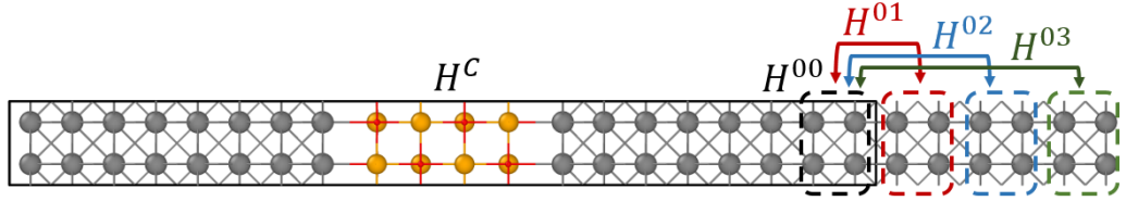
Figure 3.8: Example of tunneling junction composed by 4 silver cubic cells electrodes and 2 cubic cells of magnesium oxide in the middle. The Hamiltonian blocks used for transport calculations are schematized: H^C is the Hamiltonian of the central region and the blocks H^{0i} define the semi-infinite periodic Ag electrodes.
