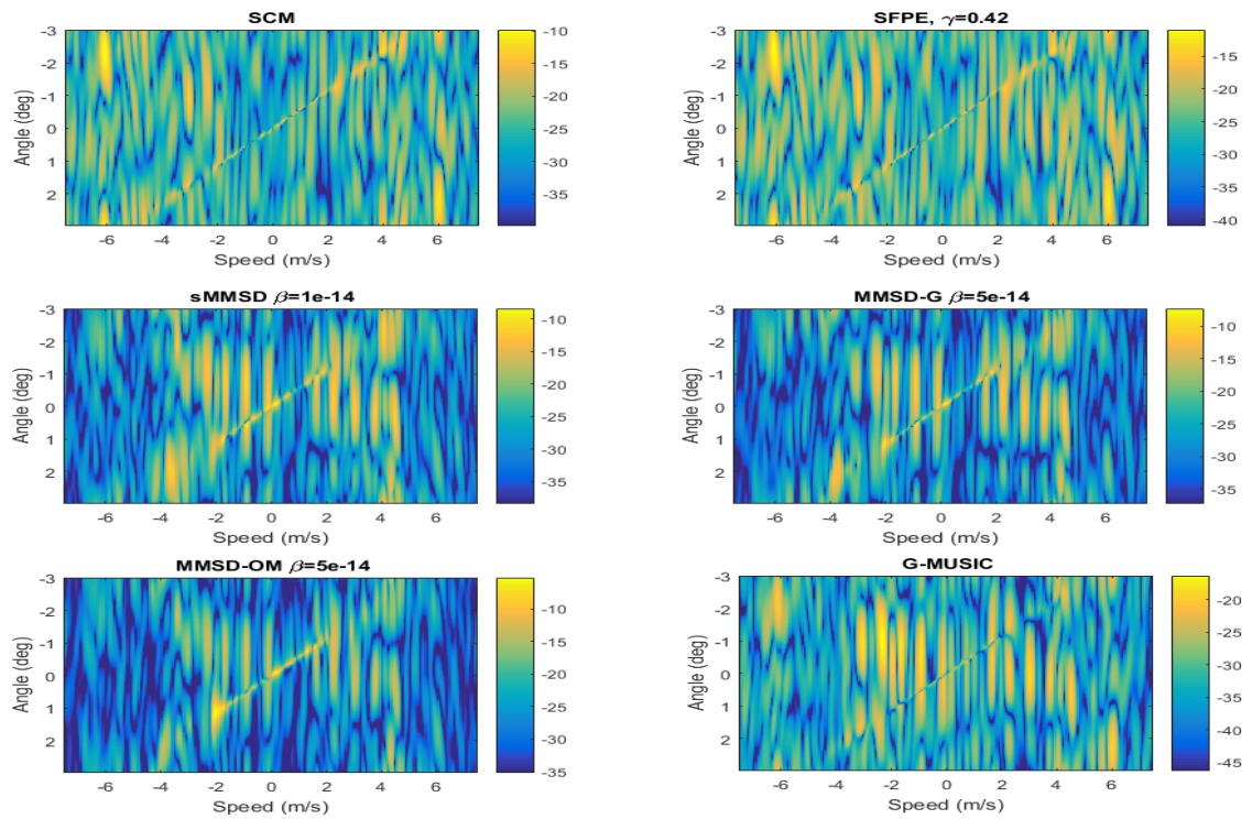
Figure 4.11: The output of detectors in presence of outlier, K = 2R with K \ll N , R = 46 , N = 256
