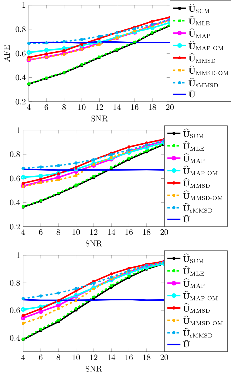
Figure 4.2: AFE w.r.t. SNR for R=5 , N = 20 , \nu = 0.5 , \mathbf{U} \sim \text{CGB}(\{\kappa_0 \phi_r \bar{\mathbf{U}} \bar{\mathbf{U}}^H\}) , \kappa_0 = 300 from top to bottom: K = 3R , K = 4R and K = 6R
