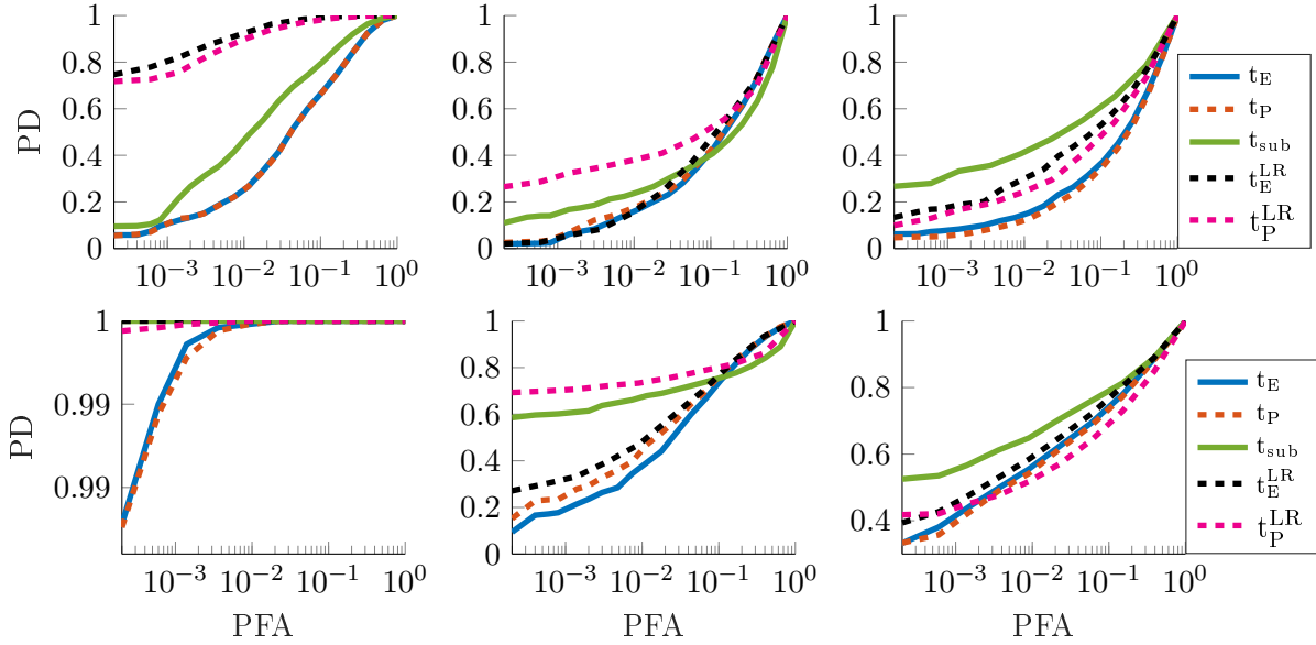
Figure 3.1: ROC curves for Scenario 1 to 3 (from left to right column) where SNR = 0dB (top) and SNR = 5dB (bottom).
