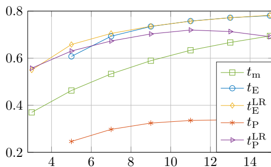
Figure 3.5: PD versus spatial window size \sqrt{K} for fixed PFA = 5% of the different detectors on the UAVSAR dataset.
