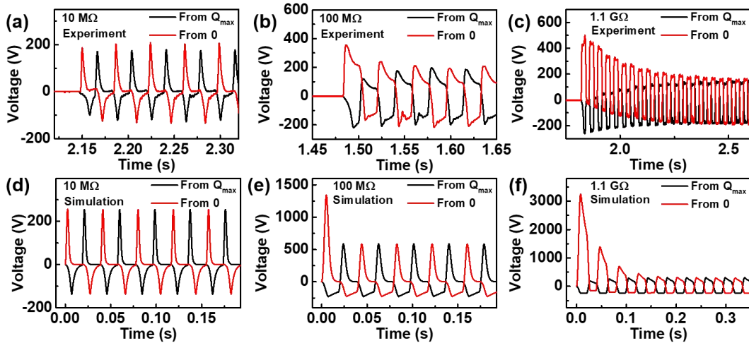
Figure 3-22 (a), (b), and (c) Measured output voltage of the TE-KEH with load resistances of 10 MΩ, 100 MΩ, and 1.1 GΩ respectively. (d), (e), and (f) Simulated output voltage of the TE-KEH with load resistances of 10 MΩ, 100 MΩ, and 1.1 GΩ respectively.
