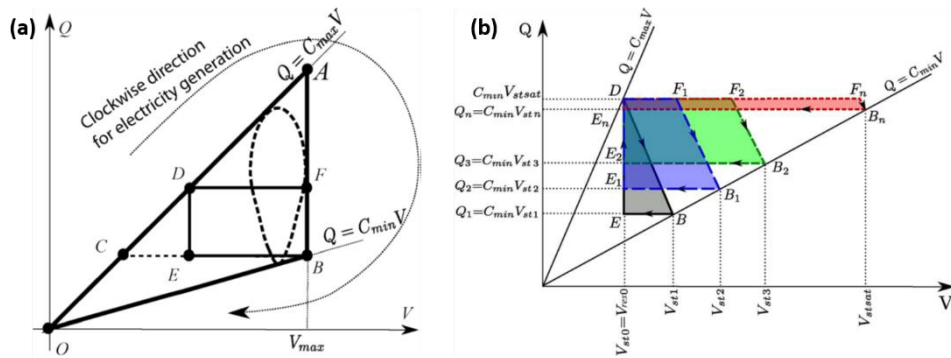
Figure 1-5 (a) Common shapes of the QV cycle of ES-KEHs. (b) Illustration of successive QV cycles from an ES-KEH with an idealized pre-charged charge pump circuit. [27]
