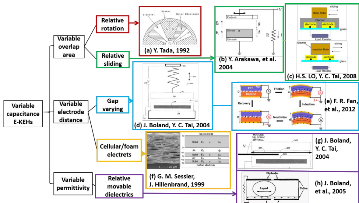
Figure 2-10 Different types of variable capacitance E-KEHs with representative material and structure designs. (a) Relative rotation design from [64]. (b) Relative sliding design from [67]. (c) Relative sliding design from [68]. (d) Gap-varying design from [69]. (e) Gap-varying design from [70]. (f) Cellular electret design from [71]. (g) The design with movable solid dielectrics from [69]. (h) The design with movable liquid dielectrics from [72].
