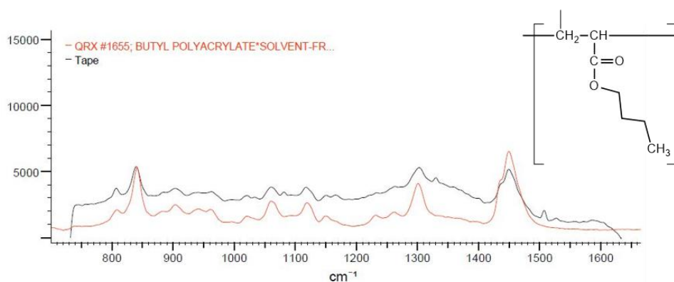
Figure 5-5 The Raman spectrum of the adhesive measured from the tape we used (black line), and the Raman spectrum of the butyl polyacrylate in the database provided by the Bio-Rad Laboratories, Inc (red line). Inset is the chemical constitution of the butyl polyacrylate.
