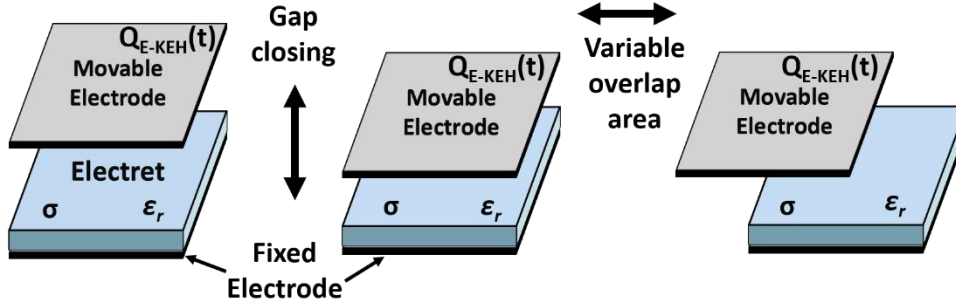
Figure 2-16 Parallel-plate configurations of E-KEHs.
