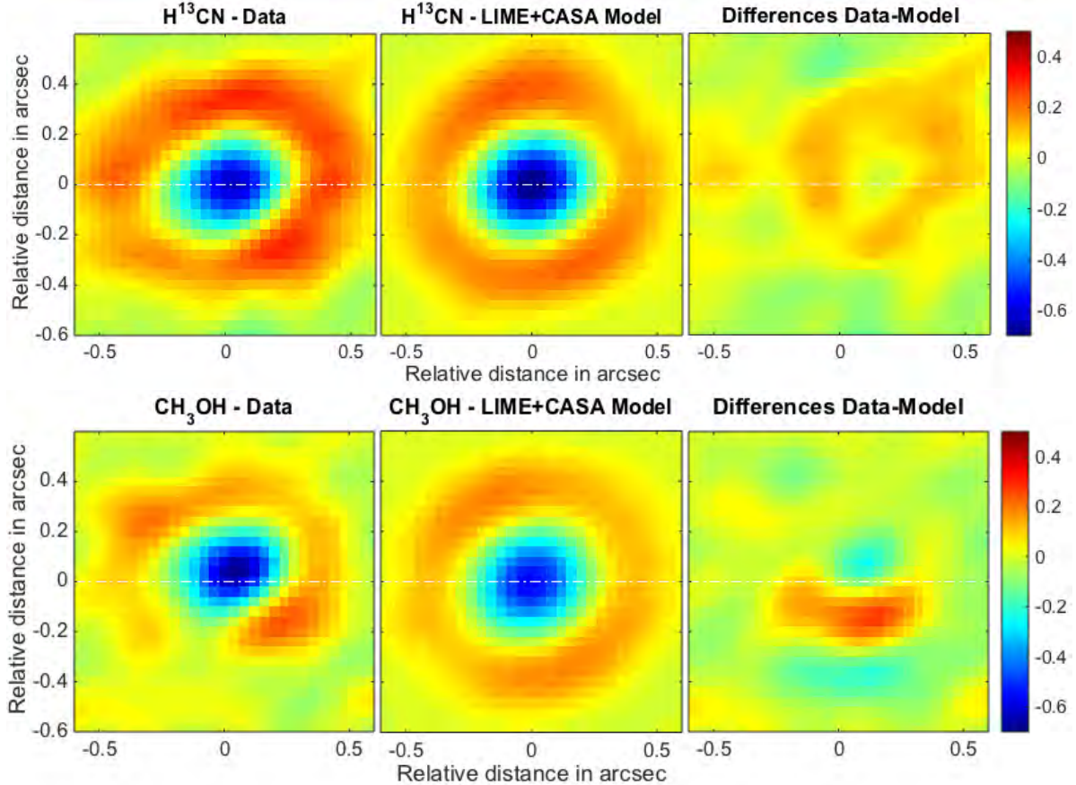
Figure 2. Molecular map of H 13 CN (top) and CH 3 OH (bottom). The left column shows the observed maps, the central column shows the model, and the right column shows the residual between the model and the observed maps.
