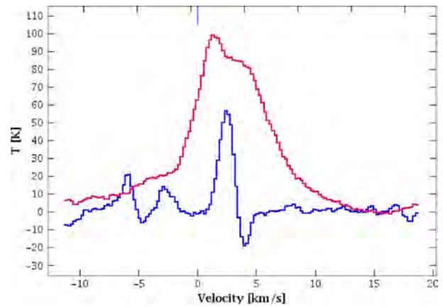
Figure 1. HNC O 15 0,15 –14 0,14 line emission as observed towards IRAS16293 in the PILS survey towards source A (red line) and source B (blue line).
