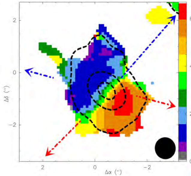
Figure 1.23. Moment 1 map (velocity field) of the C^{34}S (7–6) transition observed with the SMA towards source A. The color bar at the right indicate the scale in \text{km s}^{-1} . The black dashed contours show the continuum emission at 878 \mu\text{m} , while the red and blue dashed arrows indicate the direction of the outflows. The synthesized beam is located at the bottom right. Figure taken from Girart et al. (2014).
