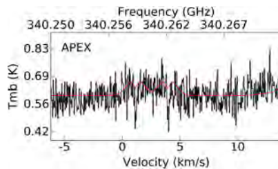
Figure B3. CN 3 – 2 transitions.
