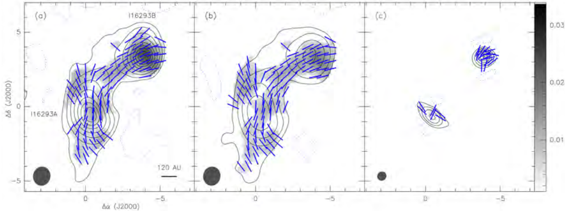
Figure 1.27. Contour maps of the dust continuum emission at 878 \mu\text{m} overlaid with the grayscale images of the polarized dust intensity and the magnetic fields on the plane of the sky (blue segments) as derived from polarized data. (a) Maps using both extended and compact configurations of the SMA. (b) Maps only for the envelope contribution. (c) Maps obtained by using only the baselines between 80 and 220 k\lambda . Figure taken from Rao et al. (2014).
