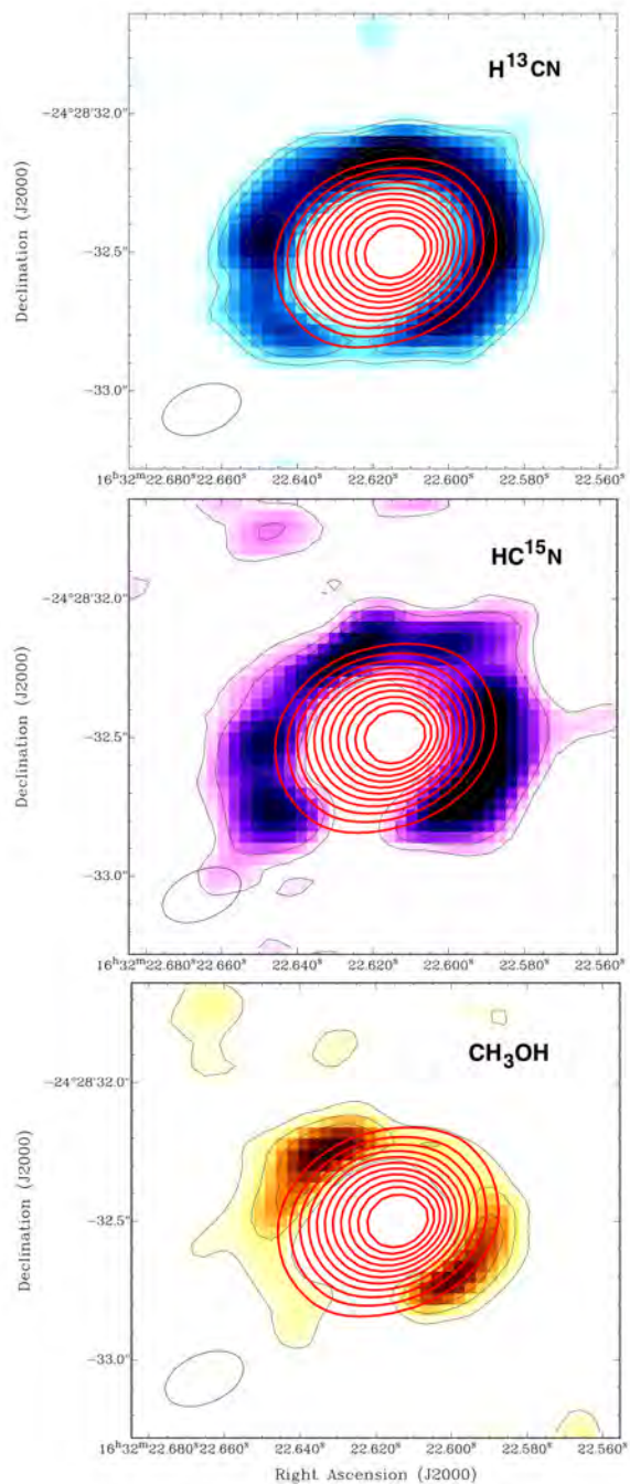
Figure 1.25. ALMA color scale integrated intensity maps of the \text{H}^{13}\text{CN} (8–7), \text{HC}^{15}\text{N} (8–7) and \text{CH}_3\text{OH} ( 9_{3,6} - 8_{2,7} ) molecules on source B overlaid with the continuum emission at 0.45 mm (red contours). Figure taken from Zapata et al. (2013).
