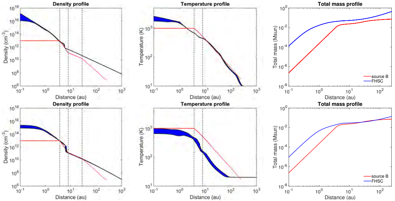
Figure 3. Density, temperature and total mass profiles for run 023 (top panels) and run 119 (bottom panels) obtained by Vaytet & Haugbølle (2017) are shown in blue, while the predicted profiles from our model are shown in red. The width of the blue renderings of the model reflects their time evolution.
