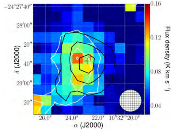
Figure 5. Moment 0 (integrated intensity) map of the J = 1 - 0 transition of ^{13}\text{CN} at 108.780 GHz. The white contours correspond to the emission of the same transition in steps of 0.03 \text{ K km s}^{-1} , while the black contours correspond to the emission of the ^{12}\text{CN} J = 1 - 0 transition at 113.144 GHz in steps of 0.2 \text{ K km s}^{-1} . The beam is shown at the bottom right of the figure. The red crosses indicate the position of A and B sources.
