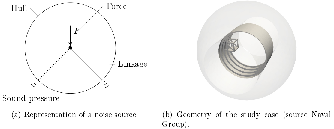
Figure 4: Study case: a keelson attached to a section of a hull submerged in water. An oscillating force is applied to the keelson and its energy is transmitted to the water through the hull.
