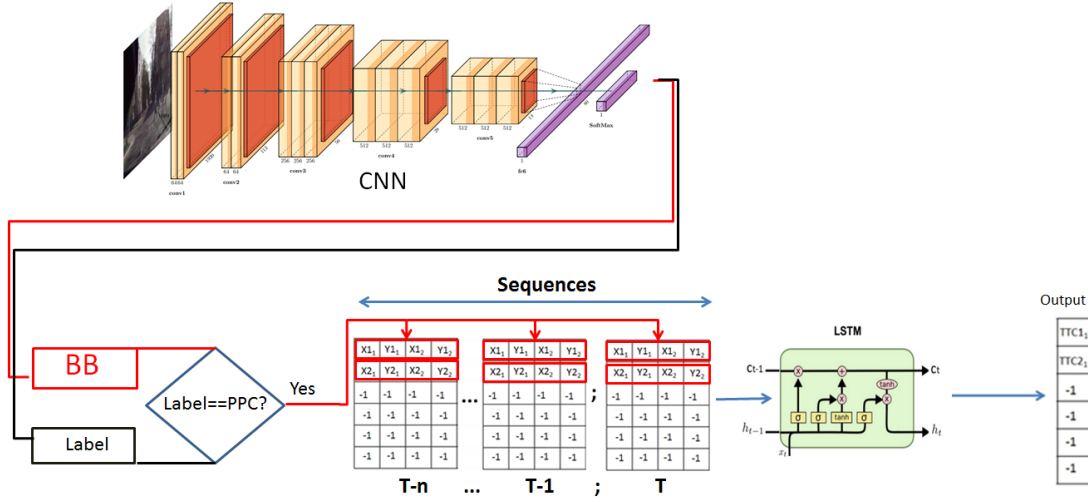
Figure 3.8 – Our time to cross the street estimation method using only BB coordinates in order to estimate the time to cross the street. BB= Bounding Box coordinates, Label= Pedestrian action tag, PPC= Pedestrian Preparing to cross the street; TTC= time to cross; -1= no pedestrian.
