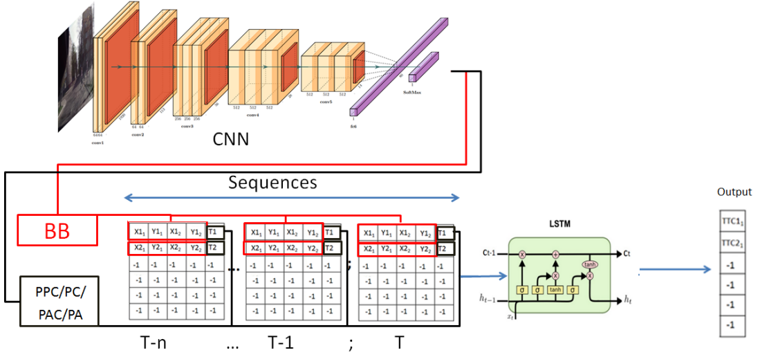
Figure 3.9 – Our time to cross the street estimation method using the BB coordinates and pedestrian action labels in order to estimate the time to cross the street. BB= Bonding Box coordinates, PPC= Pedestrian is Preparing to Cross the street; PC= Pedestrian is crossing the street; PAC= Pedestrian is About to Cross the street; PA= Pedestrian's intention is Ambiguous; P1,P2= Detected pedestrians; T1,T2= Pedestrian Action Tags; TTC= time to cross; -1= no pedestrian.
