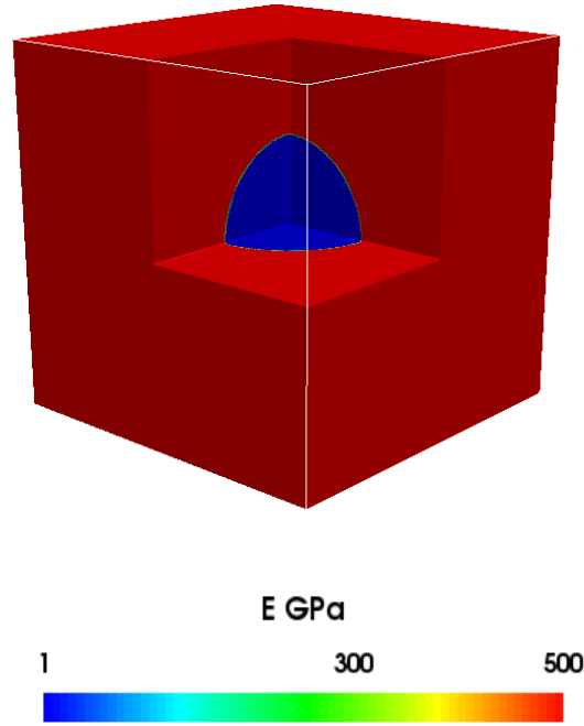
Figure 4.3: Young modulus of inclusion and matrix
