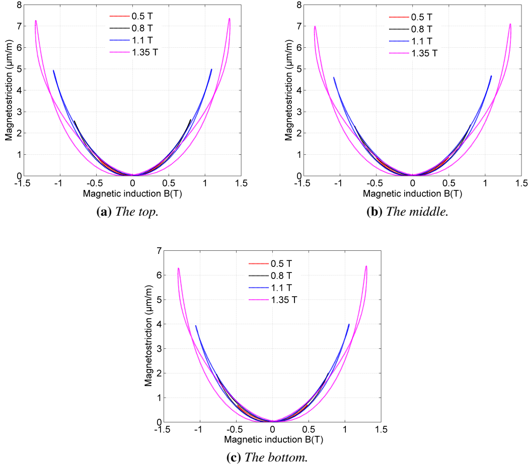
Figure 3.4.11: Magnetostriction measurements by laser vibrometer at three locations along the lamination surface ( f = 50Hz ).
