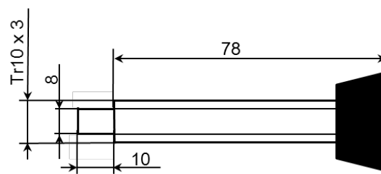
(c) Clamping screw with trapezoidal thread
