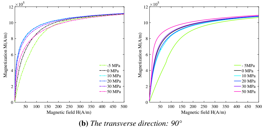
Figure 2.6.3: Anhyseretic M(H) behavior of the NO steel along different direction of magnetization and under uniaxial stress \theta = (80^\circ, 90^\circ) : Experimental results (left), modeling results (right).
