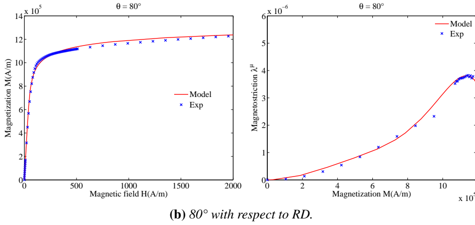
Figure 2.5.8: Comparison between measurements and modeling results: M(H) on the left, \lambda^\mu(M) on the right.
