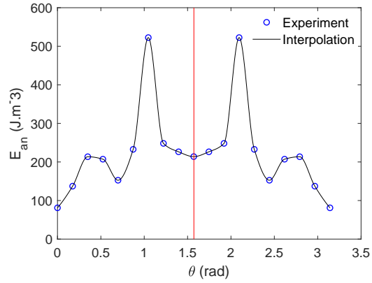
(b) Anisotropy energy for a magnetization M = 0.6 M_s .
