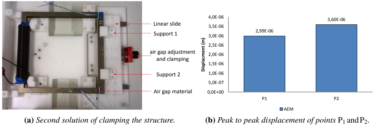
Figure 3.5.12: Displacement at two measuring points of the U-I structure (linear slide).
