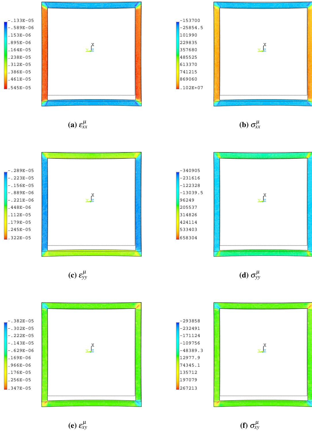
Figure 3.4.30: Induced magnetostrictive strain and stress in the structure at peak of current ( t = \frac{T}{4} ).
