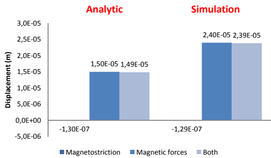
(e) 1mm air gap: E = 13\text{MPa} (AEM).
