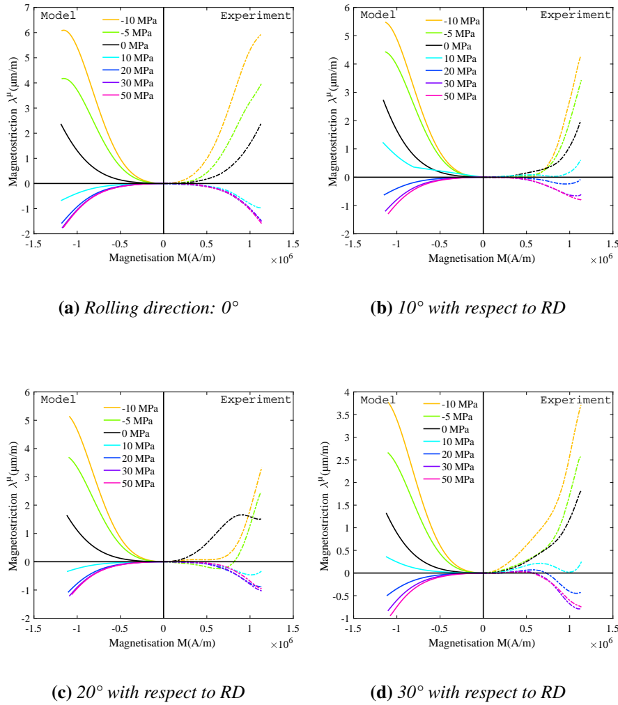
Figure 2.6.4: Anhyseretic magnetostrictive behavior \lambda^\mu(M) of NO steel different directions of magnetization and under uniaxial stress: Modeling and experimental results \theta = (0^\circ \dots 30^\circ) .
