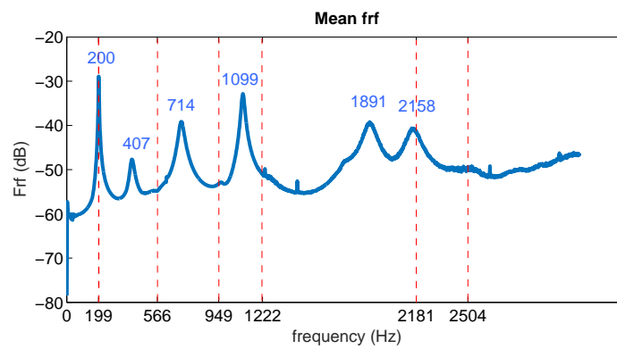
Figure 4.4.9: Experimental mean FRF for out-of-plane modes: vertical lines correspond to simulated frequencies (laminated model).
