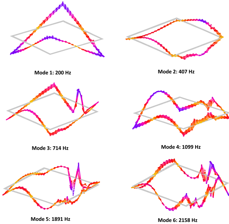
Figure 4.4.10: Out-of-plane modes shapes (measured).
