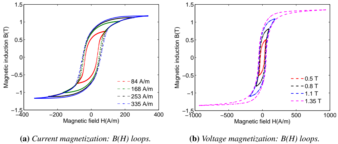
Figure 3.4.5: Hysteretic behavior: B(H) loops at point B.
