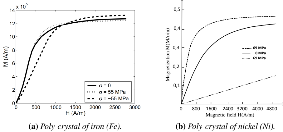
Figure 1.5.1: Stress effect on magnetization [22].
