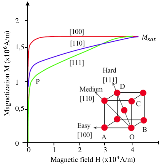
Figure 1.2.3: Magneto-crystalline anisotropy: Cubic crystal lattice of iron showing the easy magnetization directions ( < 100 > ), the medium ( < 101 > ) and the hard magnetization directions ( < 111 > ) [61].
