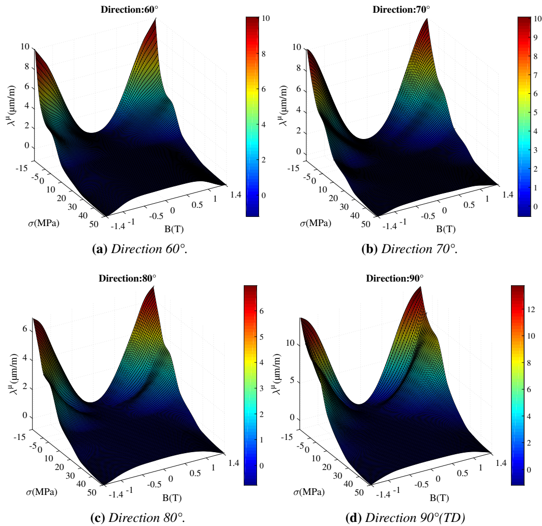
Figure 2.4.5: Anhyseretic magnetostrictive behavior under stress in different direction with respect to the rolling direction (1.4 T, 6Hz): \theta = (60^\circ \dots 90^\circ) .
