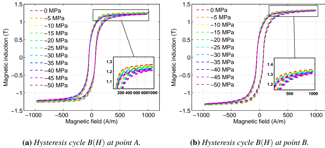
Figure 3.4.15: Voltage magnetization: hysteresis cycles under compressive stress at H_{max} = 1000 A/m.
