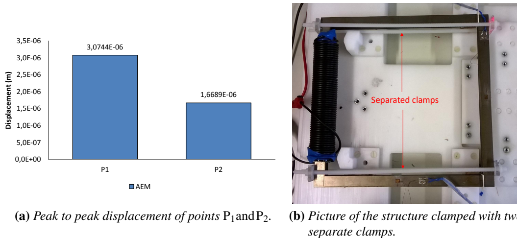
Figure 3.5.11: Displacement at two measuring points of the U-I structure (clamps).
