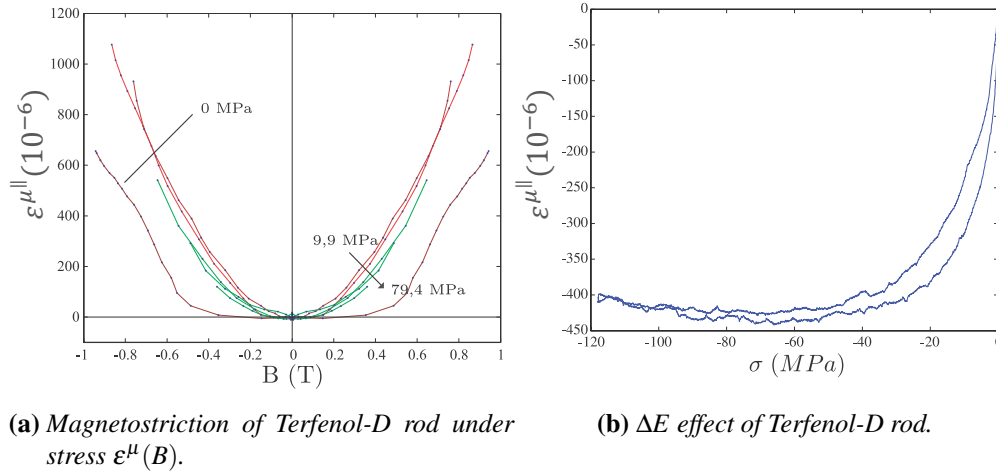
Figure 1.9.4: Magnetostrictive deformation measurements: (a) Anisotropic magnetostriction of a Terfenol-D rod as a function of induction at different compression stresses, (b) magnetostriction (at zero field) due to compression of a Terfenol-D sample [39].
