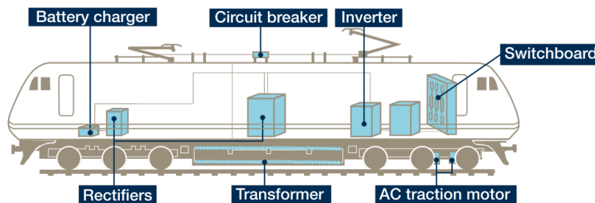
Figure 0.0.1: Transformer in train locomotive (VonRoll website).
