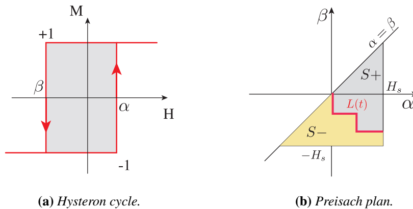
Figure 1.9.2: Preisach Hysteron [74].
