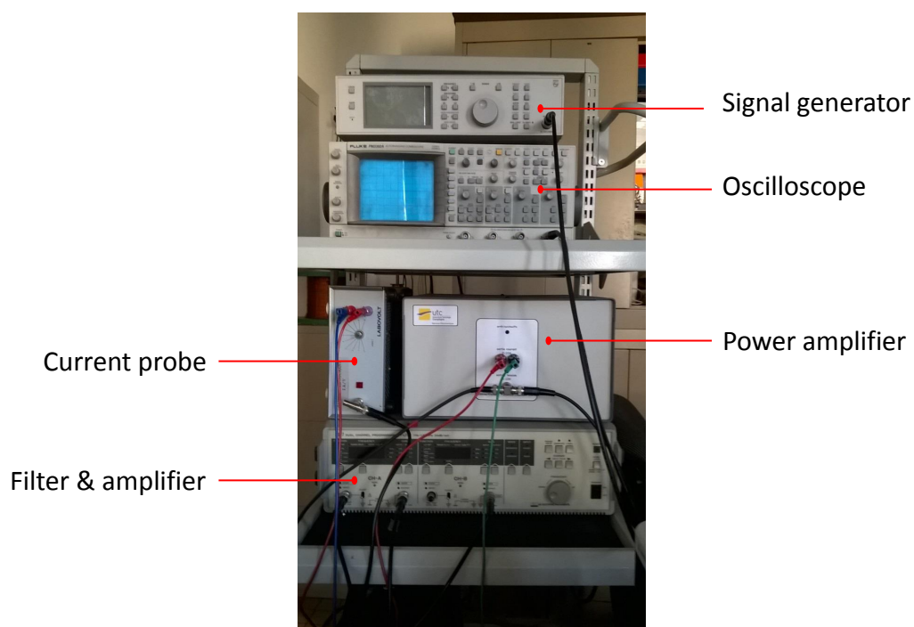
Figure 3.3.7: Current magnetization set-up.
