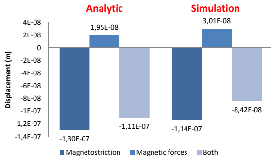
(a) 1mm air gap: E = 10\text{GPa} (Glass mat).
