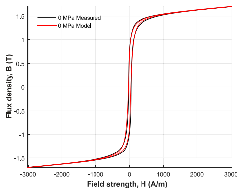
(a) B(H) loop at \sigma = 0 MPa.
