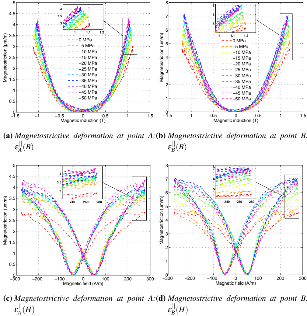
Figure 3.4.18: Current magnetization: magnetostriction deformation under compressive stress at H_{max} = 275 \text{ A/m} .
