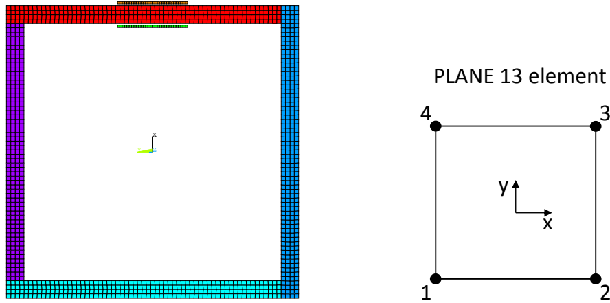
Figure 3.4.22: Model mesh: PLANE13 element.
