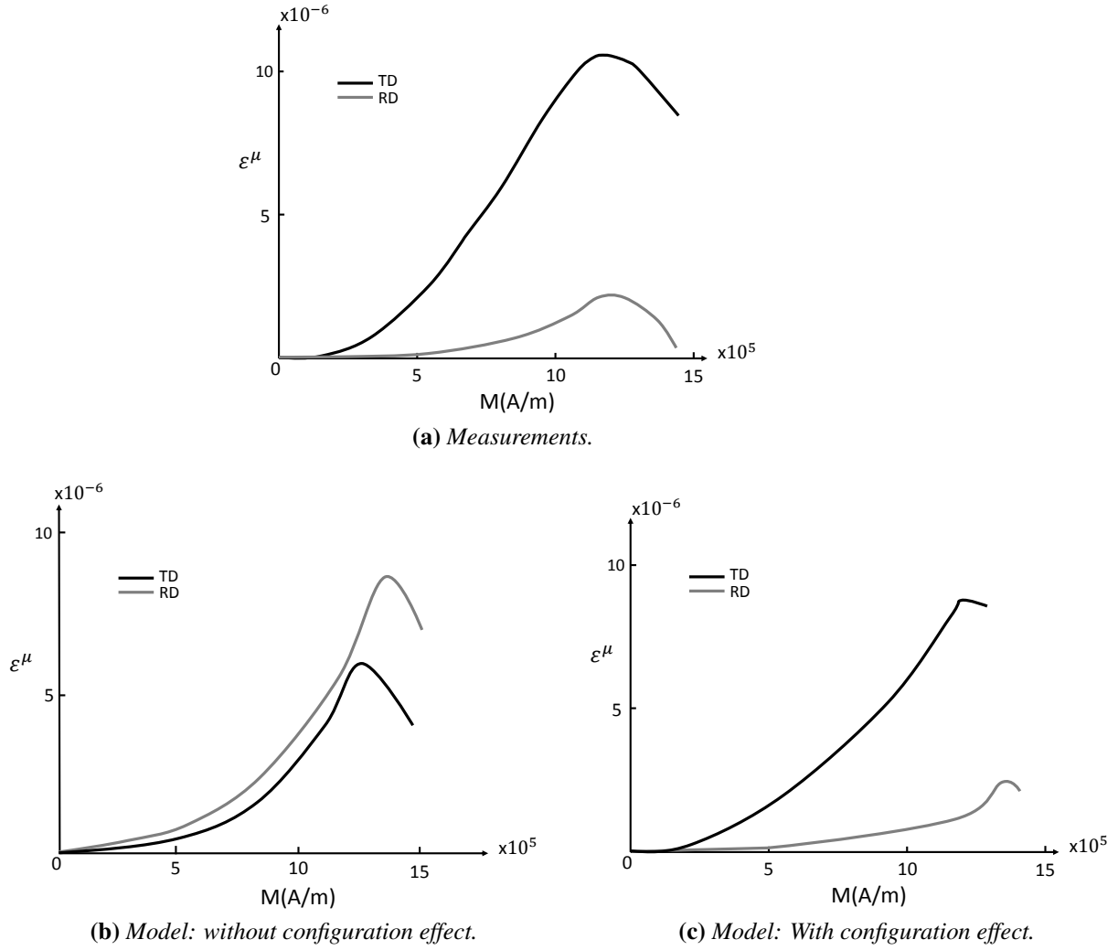
Figure 1.9.7: Magnetostriction strain of NO 3%Si-Fe: Comparison between measurement and modeling results, with and without the consideration of the configuration effect [48].
