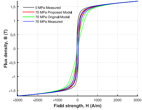
(b) B(H) loop at \sigma = 70 MPa.
