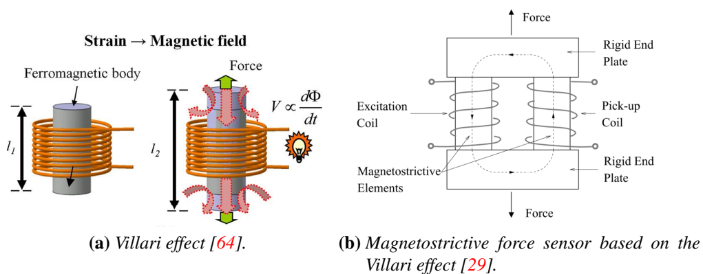
Figure 1.5.2: Villari effect : (a) principal, (b) application.
