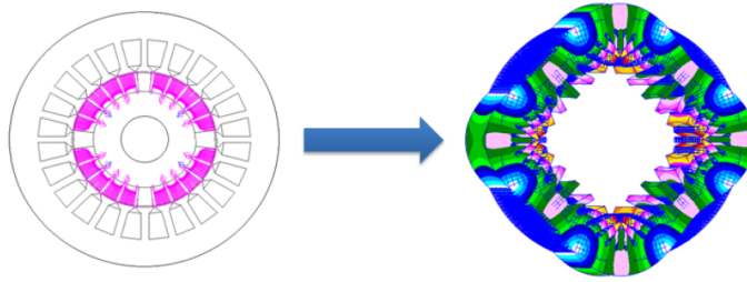
Figure 4.3.2: Magnetic pressure due to Maxwell forces (left) and generated deformation of stator (right) [44].
