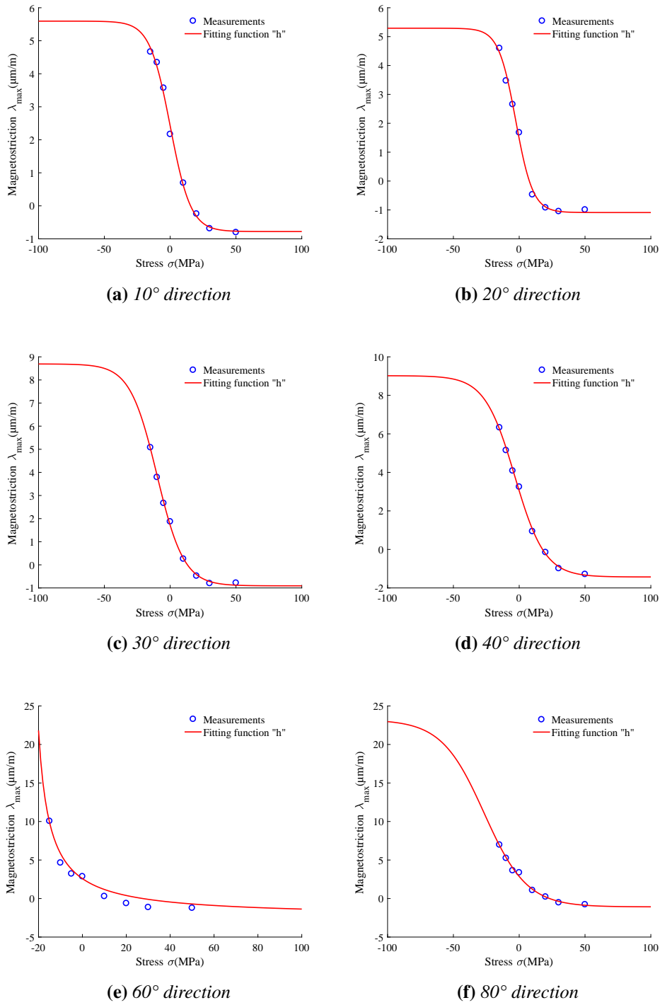
Figure B.1: Comparison between fitted and measured magnetostriction deformation for direction of cut: 10°, 20°, 30°, 40°, 60°, 80°
