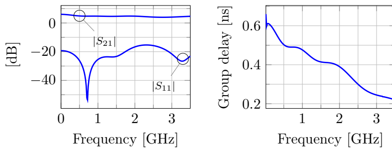
Figure 5.17 – Frequency response and group delay of the balanced distributed amplifier based transversal filter of Fig. 5.16a (SPICE simulation).
