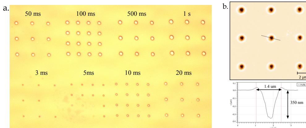
Fig. IV.25 a) Reflection image after development process (60 s using MF-319 diluted 1 : 3 with deionized water) of the holes created with 0.95 NA objective. b) Topographic AFM image of the matrix exposed in 10 ms after development.
