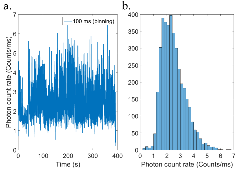
Fig. III.6 a) Total photons count rate as a function of time of the same nanocrystal shown in Figure III.3. The nanocrystal was excited with an optical power of 850 \text{ W/cm}^2 in pulsed mode. We have displayed the graph with a binning time of 100 ms. b) Histogram of the photo-events shown in a) with a binning of 0.2 counts/ms.
