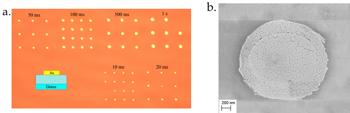
Fig. IV.26 a) Reflection image of nano-disks over glass substrate fabricated with 0.95 NA objective b) Scanning electron micrograph of one Au nano-disk of 1.80 \mu\text{m} in diameter corresponding to the 3 \times 3 matrix 1 s.
