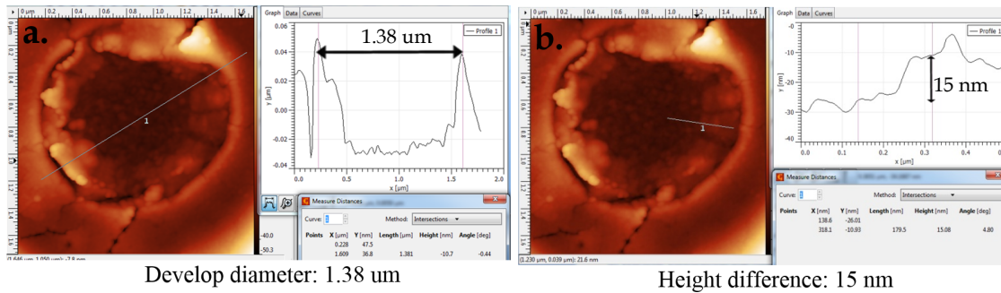
Fig. A.5 AFM image showing the center of the hole. a) Trace line indicating the develop diameter around 1,38 \mu\text{m} . b) Trace line showing the differential in height from the center hole to the layer which comprise the radial pattern.
