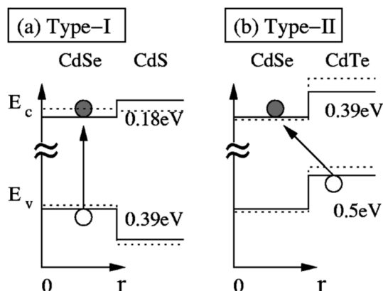
Fig. II.2 Classification of core/shell heterostructure. a) Type-I heterostructure. b) Type-II heterostructure. In type-I, the hole remains confined inside the CdSe-core while the electron is delocalized in the whole structure. In type-II, the hole wave function is localized within the CdTe-shell and the electron wave function is confined in the CdSe-core. The solid lines represent the natural conduction and valence bands of CdSe/CdS (for type-I heterostructure) and CdSe/CdTe (for type-II heterostructure). In both classifications, the conduction bands are nearly aligned, whereas the valence bands are not aligned. The dash lines represent the theoretical electronic bands reported on [42]. In such calculations, the difference between natural and theoretical electronic bands are explained by strain effects (tensile and compressive strain). Figure adapted from [42].
