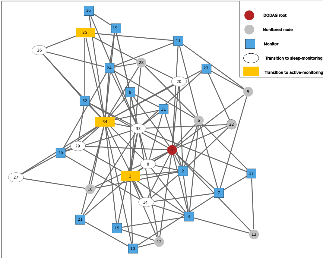
FIGURE 6.3: Optimal solution in a given period for the KARATE [6] network topology with 34 Vertices and 114 edges. reservedBattery_i = 1641.6 \text{ mJ} (0.05 % of total power).
