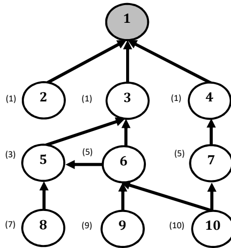
FIGURE 5.1: Logical routing topology (DODAG) built RPL, node 1 is the root, nodes' ranks are between brackets.
