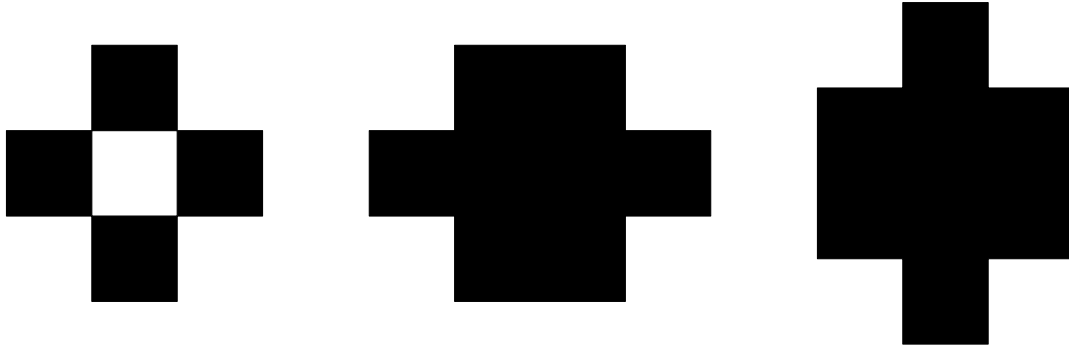
Figure 2.13: The shapes associated to the total domination. The big ones are the two different unions of two copies of the small one. Tiling the plane with the small one boils down to tiling the planes with the two big ones.
