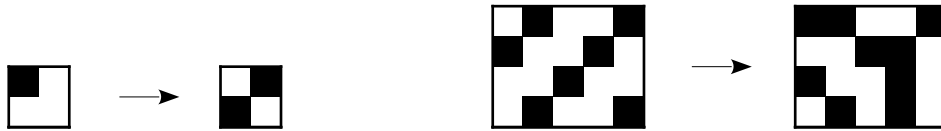
Figure 2.10: The two rules used to convert a restriction of an optimal 2-dominating set of \mathbb{Z}^2 into optimal 2-dominating set of a rectangle. For each corner, if one of the two patterns before the arrows appear, we replace them by the version on the right of the arrow.
