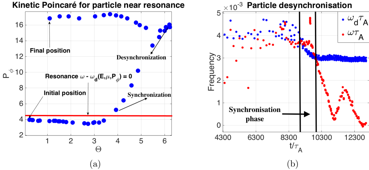
Figure 6.12: (a) Kinetic Poincaré plot of a particle launched near the precessional resonance at P_\varphi = 4.5 . The particle does not have time to circle in the virtual island that it is immediately transported at larger P_\varphi . (b) Compared time evolutions of the mode frequency and precessional frequency of a particle. The precessional frequency decreases slightly in amplitude when the mode is chirping, synchronizing with it over t/\tau_A \in [9.10^3, 10^4] . Afterwards, the particle desynchronizes with the mode. This synchronization phase corresponds on (a) to the de-trapping of the resonant particle.
