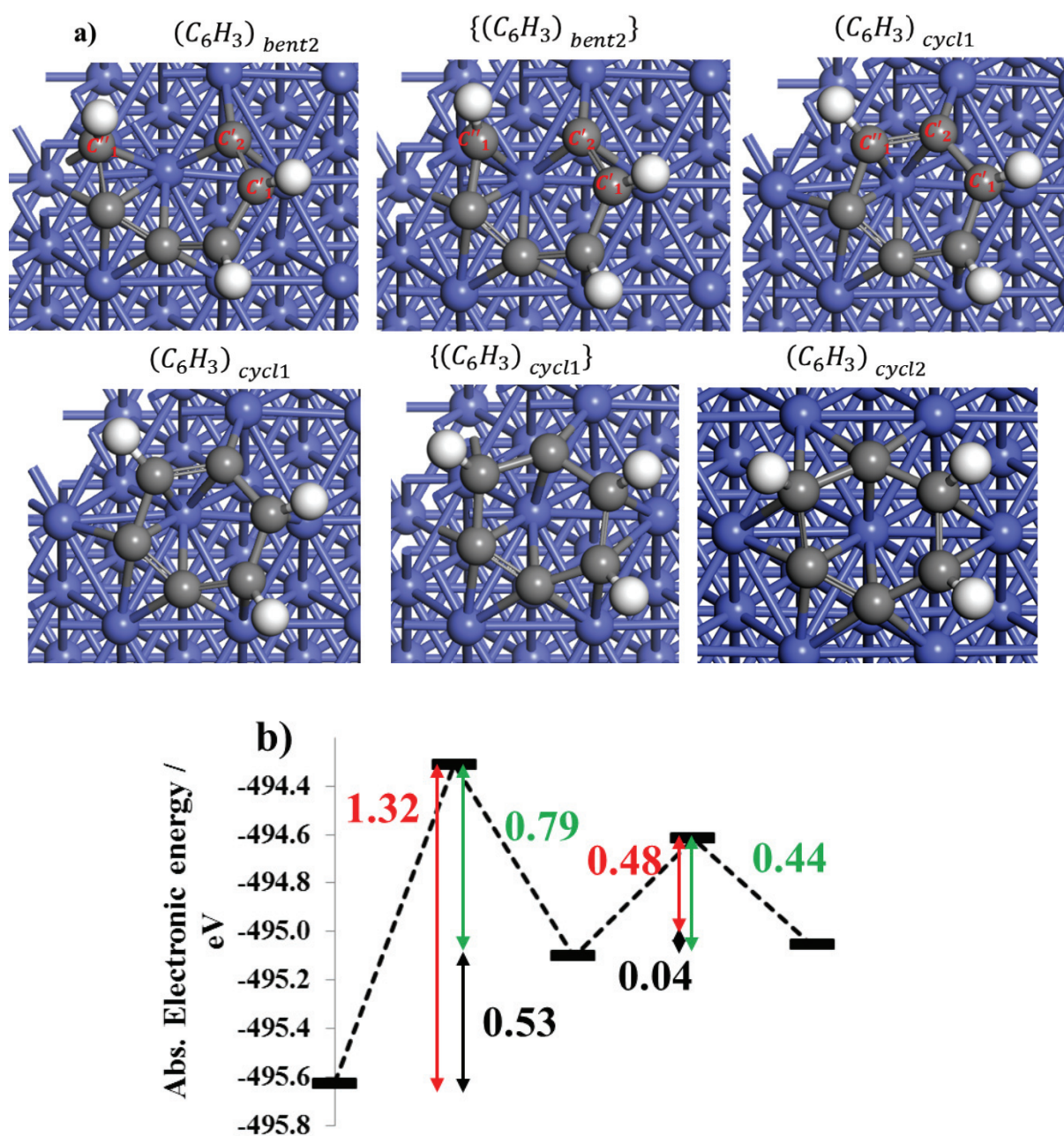
Figure 61. a) Structural and b) energetic properties of cyclization of polymeric carbon species and a cycle relaxation reaction.
