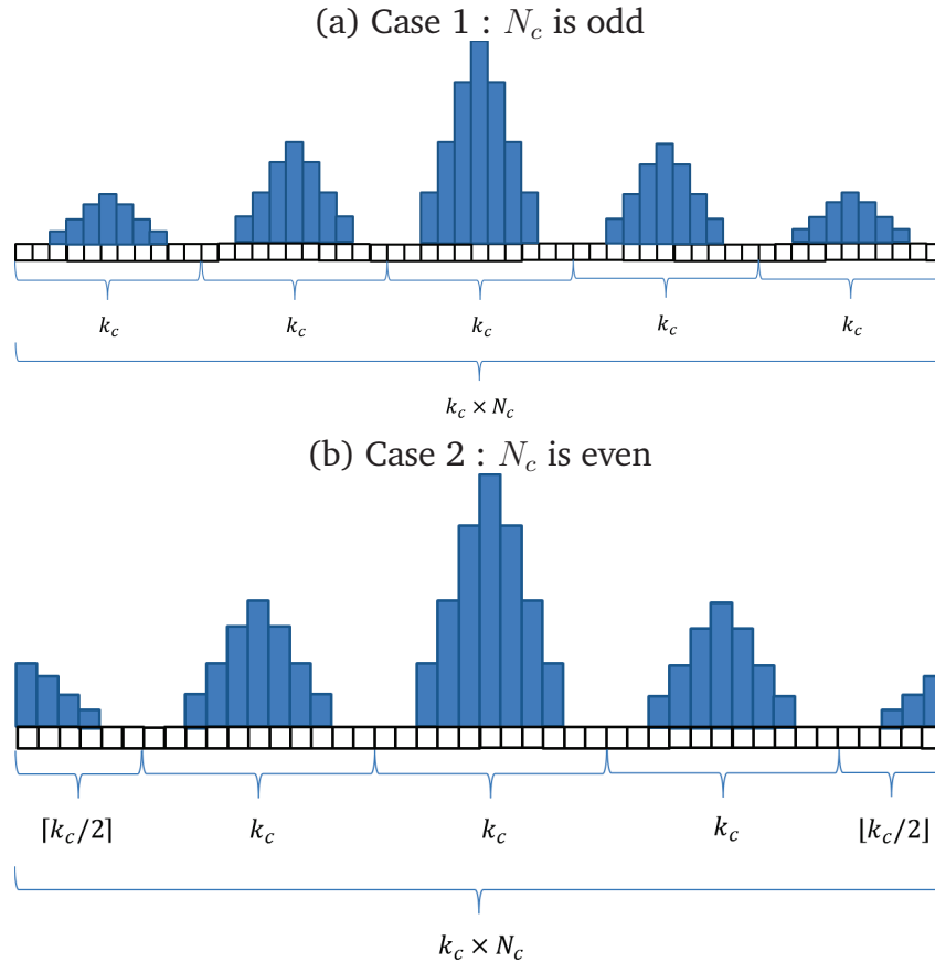
Figure 4.1: DFT of a discrete modulated signal, with indices ranging in I_N (see Remark 15 for the meaning of I_N ). Note that when N_c is even, one modulation pattern is cut in the middle.
