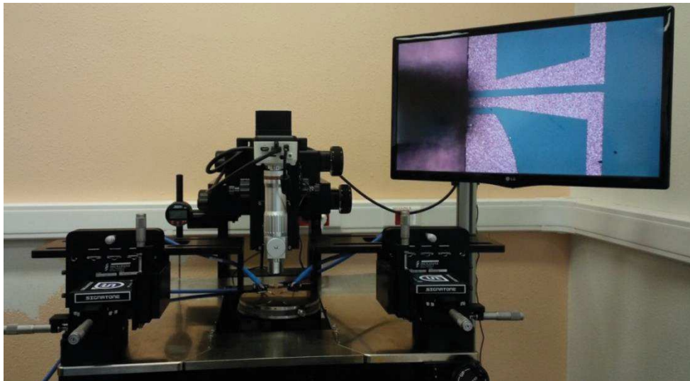
Figure 2-28: Station sous-pointe à l'IMT-Atlantique
