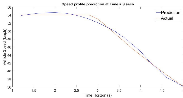
Figure 4.15 – Use Case 1: Vehicle Speed Profile prediction at time = 9 secs
