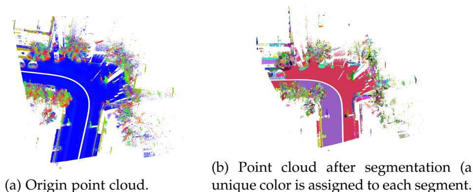
Figure A.6: Results of a segmentation by a region growing algorithm.
