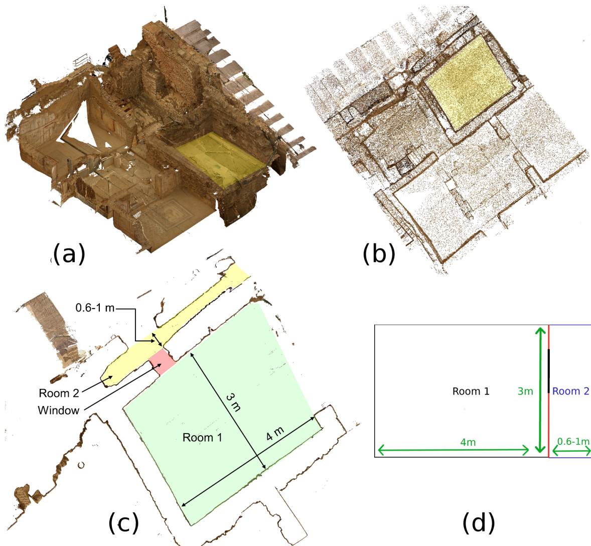
Figure 14.11: Descriptions of the watermill for the application case 2.1.2 (a) Point cloud with watermill (room illustrated in yellow); (b) Floor plot of the watermill; (c) Schematic geometric descriptions; (d) Schematic knowledge representation.
