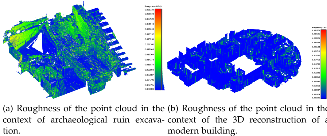
Figure 4.5: Comparison of the roughness of two point clouds acquiring by a laser scanner.
