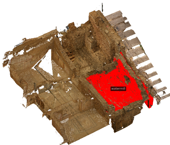
Figure 14.12: Results of watermill recognition (in red) on the application case 2.1.2.
