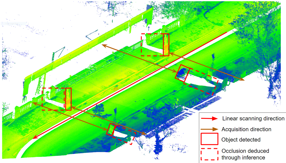
Figure 10.3: Illustration of occlusions inference.
