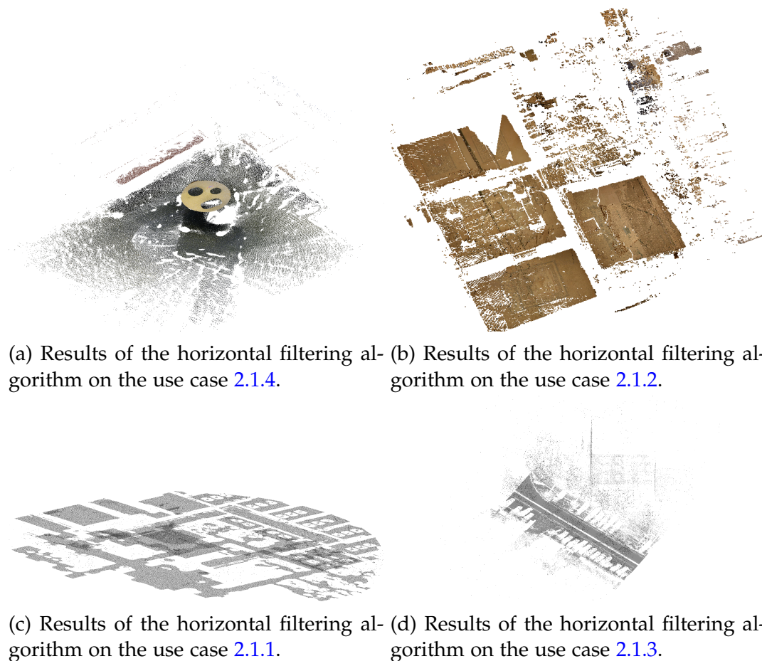
Figure 14.3: Results of the "Normal Filtering" algorithm for the floor detection in application cases studied.
