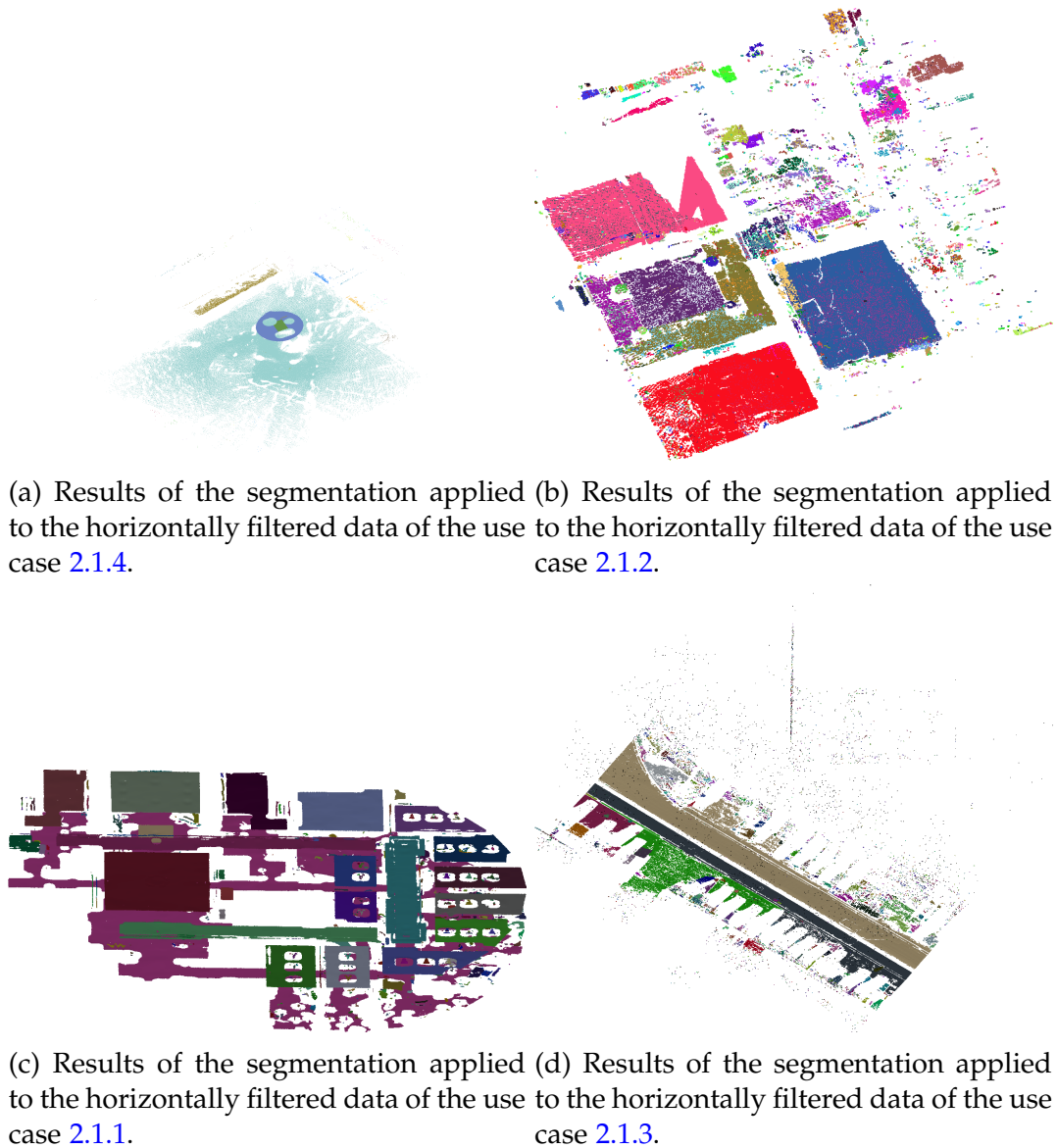
Figure 14.4: Results of the "Normal Region Growing" algorithm for the floor detection in the application cases studied. A single color is assigned to each segment.
