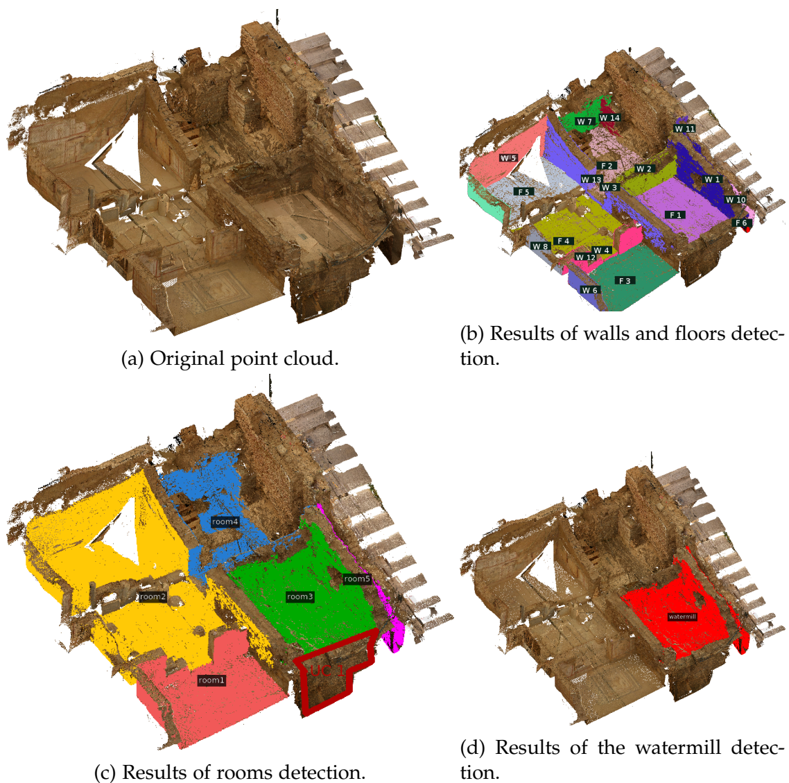
Figure 15.3: Results of objects detection on the application case 2.1.2.
