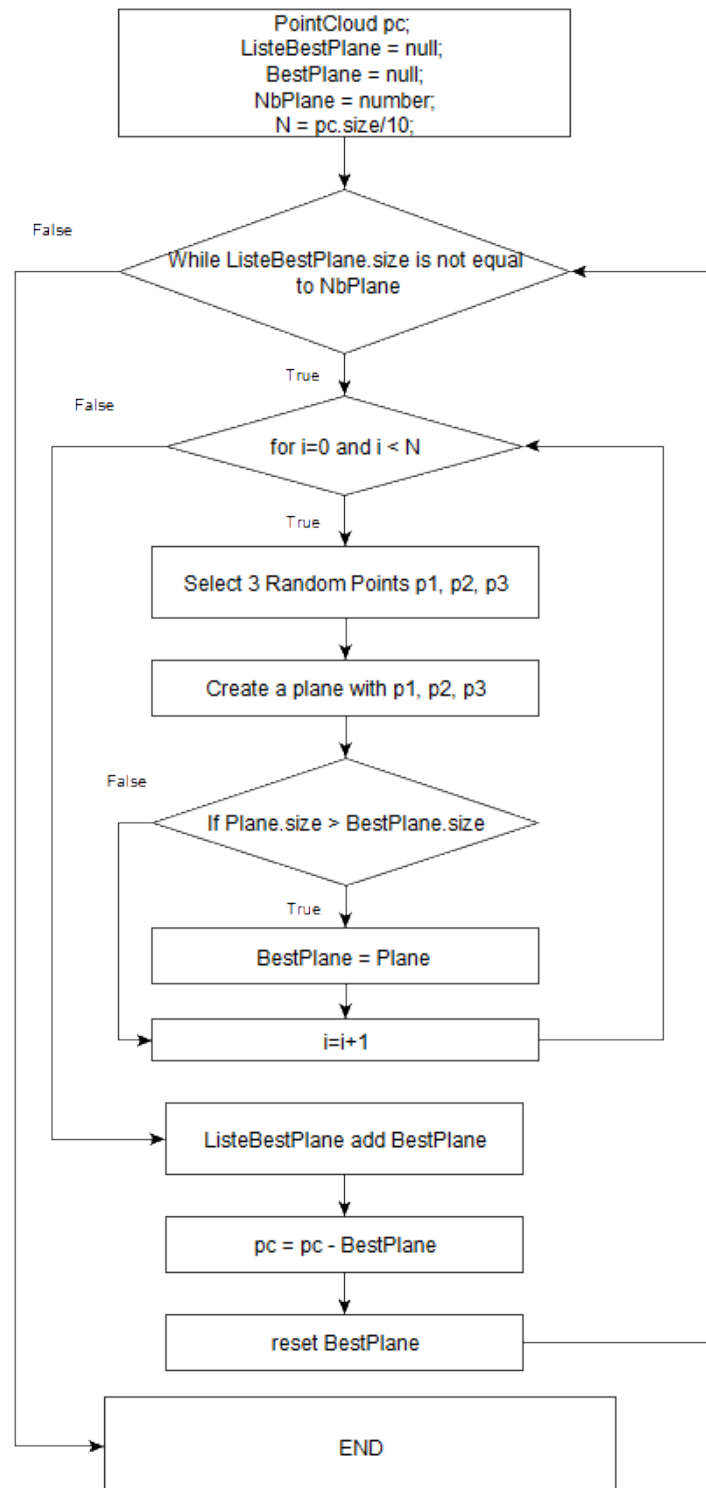
Figure A.7: Organizational chart of the RANSAC algorithm.
