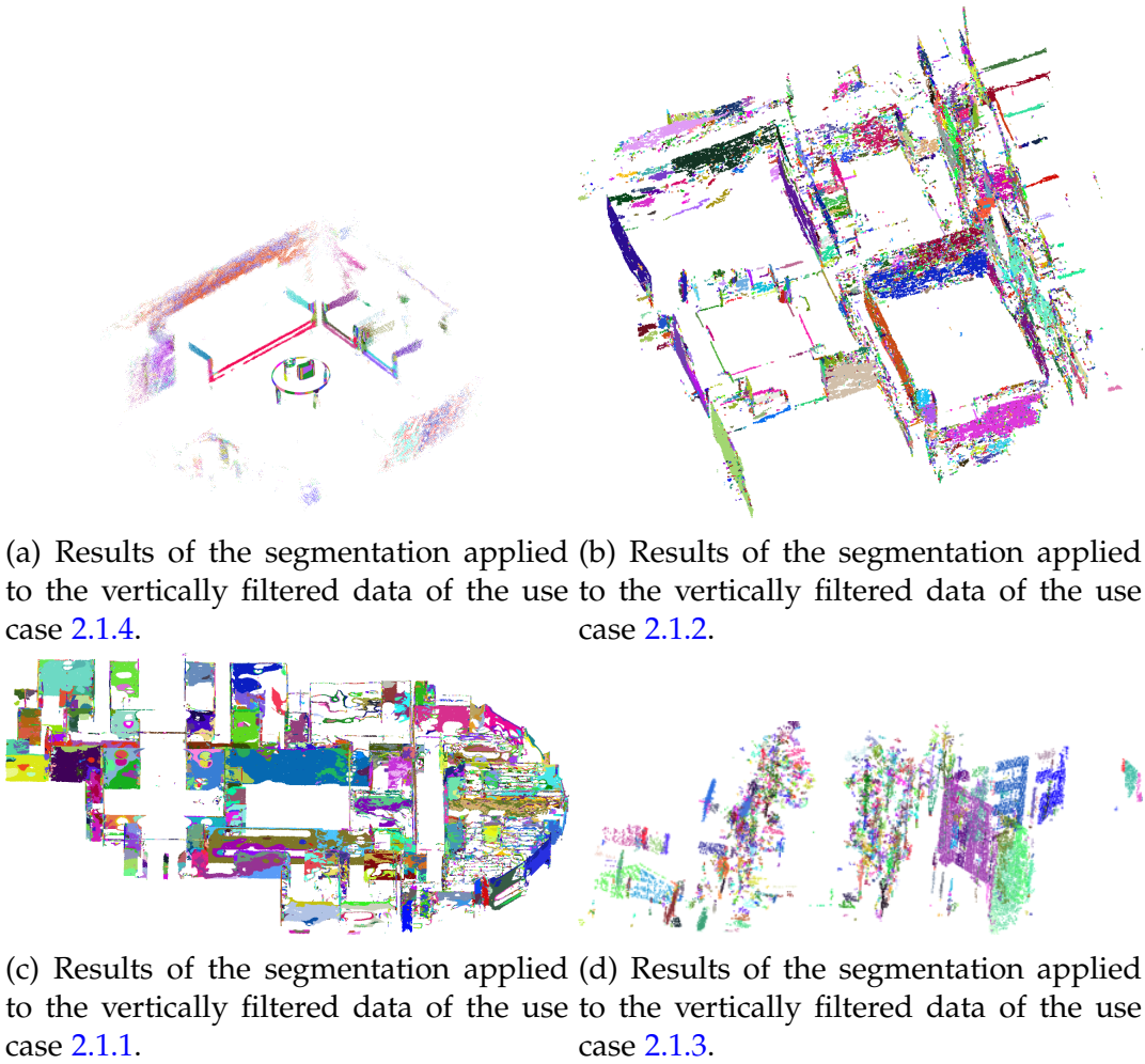
Figure 14.7: Results of the "Normal Region Growing" algorithm for walls detection in the application cases studied. A single color is assigned to each segment.
