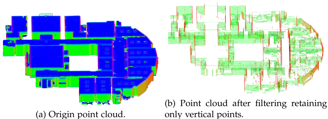
Figure A.5: Illustration of the filtering of a point cloud.
