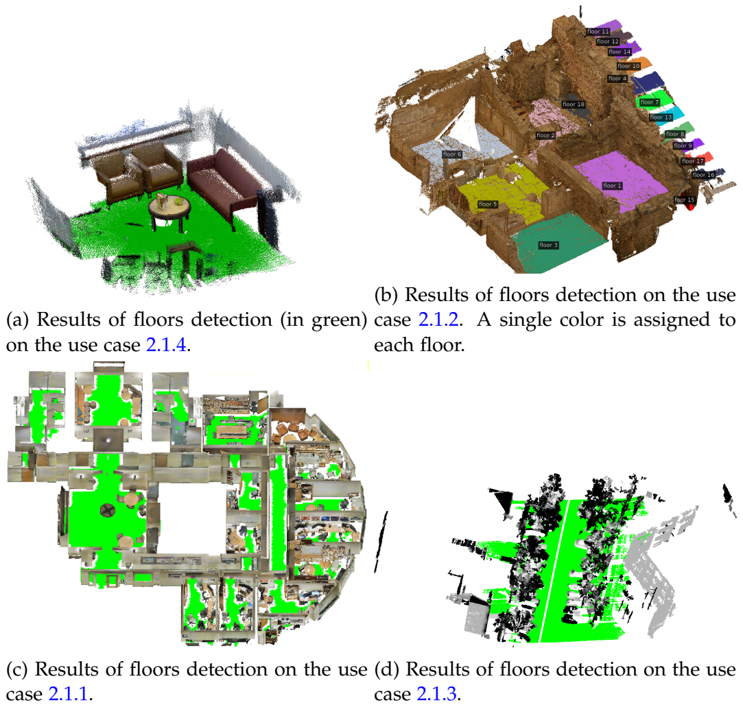
Figure 14.5: Results of floors detection on application cases studied.
