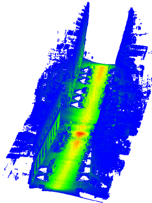
Figure 13.3: Density computation results based on the knowledge of the sensing process: high density in red and yellow, medium density in green, and low density in blue.
