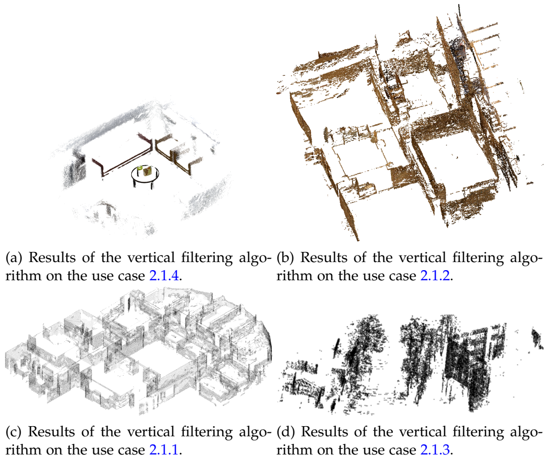
Figure 14.6: Results of the "Normal Filtering" algorithm for walls detection in application cases studied.
