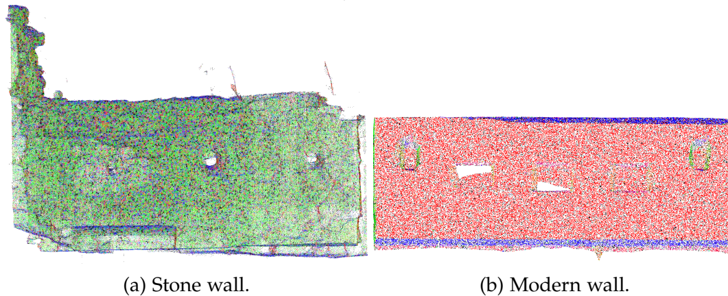
Figure 11.2: Illustration of the normal estimation. The value of the normal is converted in RGB format for the visualisation.
