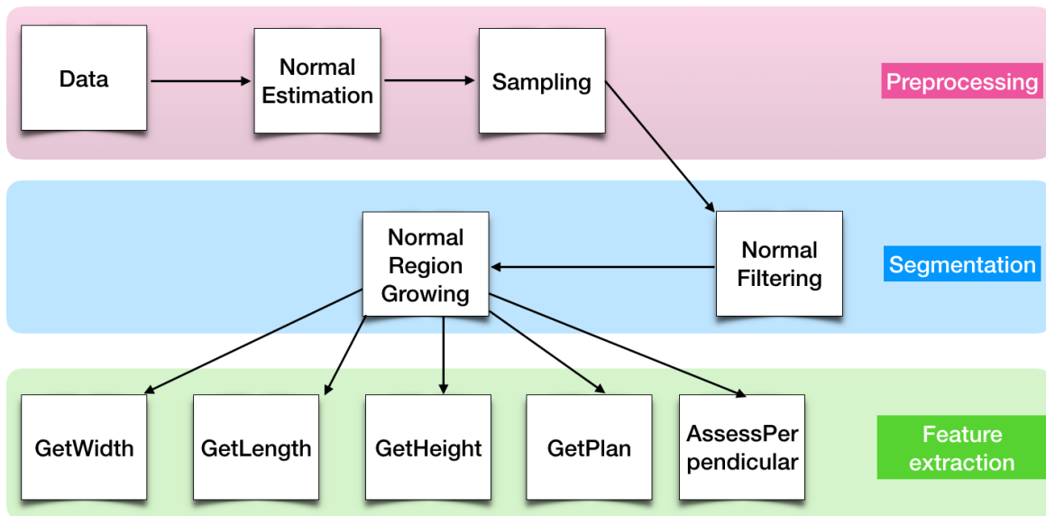
Figure 14.1: Algorithms graph for the floor detection.
