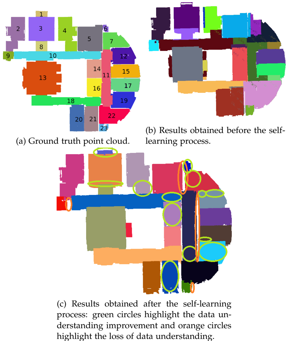
Figure 15.9: Results of detection on Stanford dataset.
