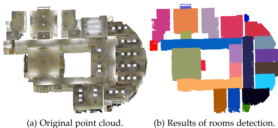
Figure 15.4: Results on the application case 2.1.1.
