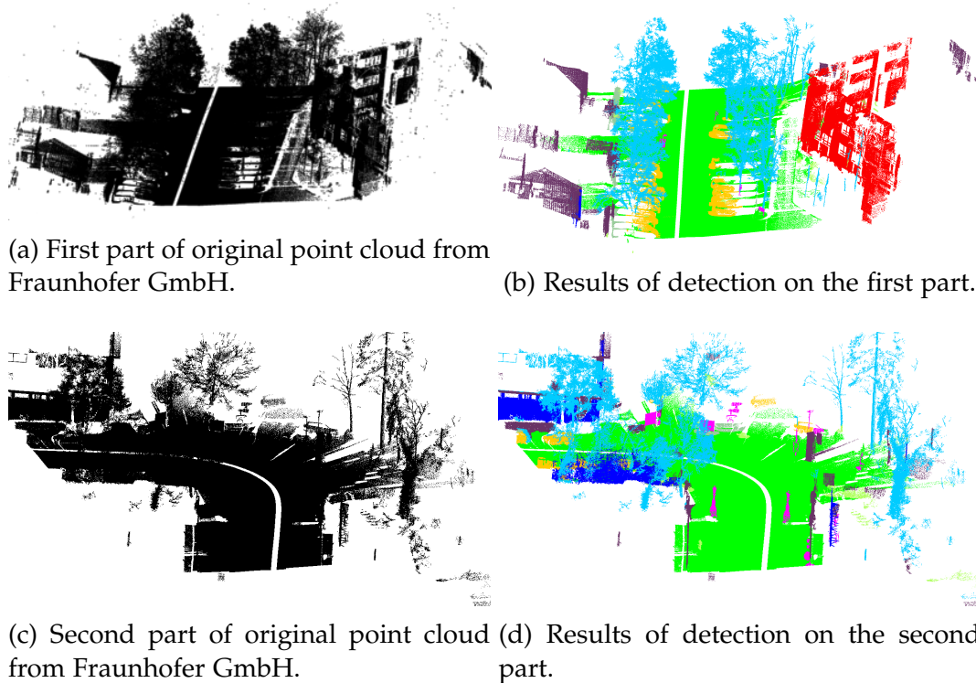
Figure 15.7: Results on the application case 2.1.3: facades in red, walls in dark blue, building elements in purple, the floor in bright green, cars in yellow, traffic signs in magenta, and trees in bright blue.
