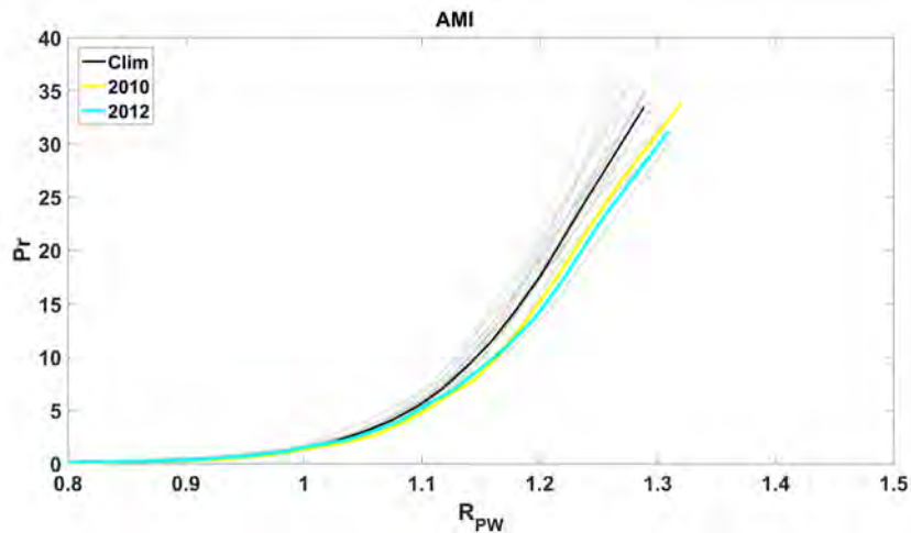
FIGURE 4.25: Conditionally average rain rate (Pr ; \text{mm.day}^{-1} ) by bins of the R_{PW} in the AMI box during MJJA. The climatology, 2010 and 2012 are represented by black, yellow and blue lines, respectively. Gray lines represent the Pr- R_{PW} relationship for each year of the reference period (1998-2014). Bins of R_{PW} were defined by quantiles of 2%.
