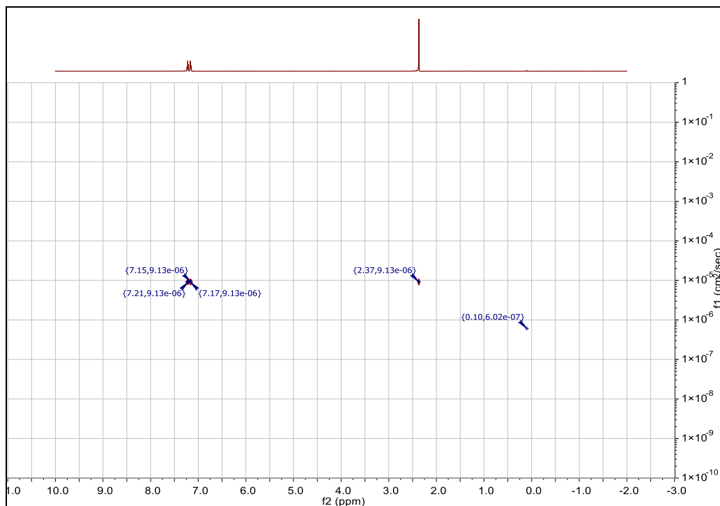
Figure SI 1.1.27 ^1\text{H} DOSY NMR spectrum of 1.2b ( c \approx 20 mM). The spectrum is recorded in deuterated chloroform at 600 MHz at 25°C. Obtained signals: D=9.13 \text{ e}^{-10} \text{ m}^2/\text{s} , V=365 \text{ \AA}^3 .
