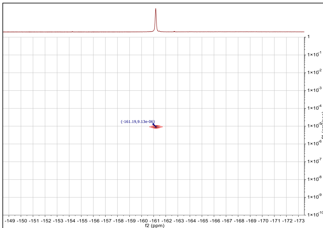
Figure SI 1.1.25 ^{19}\text{F} DOSY NMR spectrum of 1.1 ( c \approx 100 mM). The spectrum is recorded in deuterated chloroform at 565 MHz at 25°C. Obtained signals: D = 9.13 \text{ e}^{-10} \text{ m}^2/\text{s} , V = 365 \text{ \AA}^3 .
