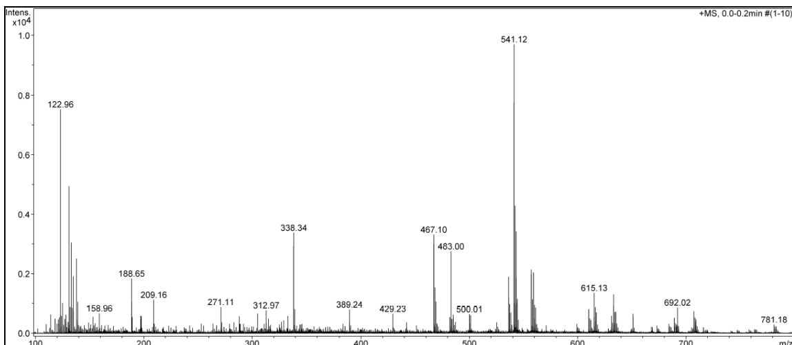
Figure SI 1.1.47b. Mass spectra of the Lewis pair 1.3f ((\text{PhF}_5)_3\text{B}-\text{P}(\text{PhF}_5)_3) recorded in positive charge mode - zoomed. Molecular masses: 1.1 ((\text{PhF}_5)_3\text{B}) = 511.99 ; 1.2f (\text{P}(\text{PhF}_5)_3) = 531.95 .
