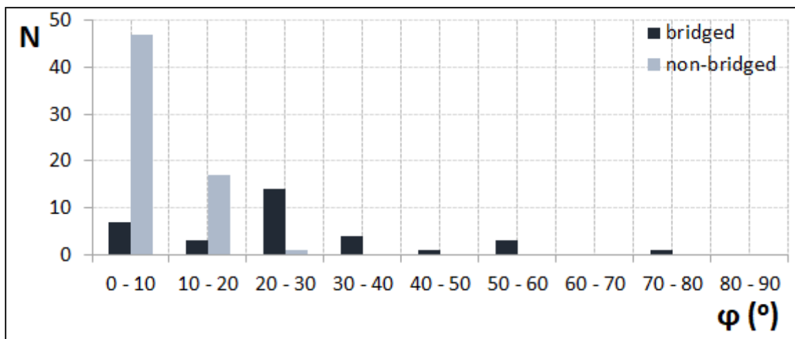
Figure 1.2.10 The distribution of the dihedral angle \varphi (Figure 1.2.1) of the interacting molecules in the B(X_1X_2X_3) - P(Y_1Y_2Y_3) set.
