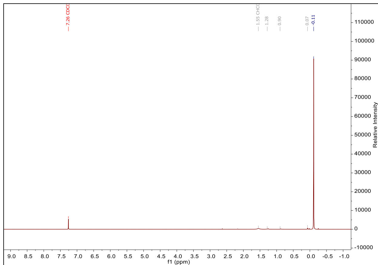
Figure SI 2.10 ^1\text{H} NMR spectrum of the synthesized complex 2.1 by modified literature procedure 285 (for the details of the synthesis, see Experimental section, page 163). The spectrum is recorded in deuterated chloroform at 400 MHz.
