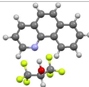
[5.3h] \Delta H_s = -12.3 kcal/mol; \Delta G_s = -0.6 kcal/mol; \Delta S_s = -39.2 kcal/mol
