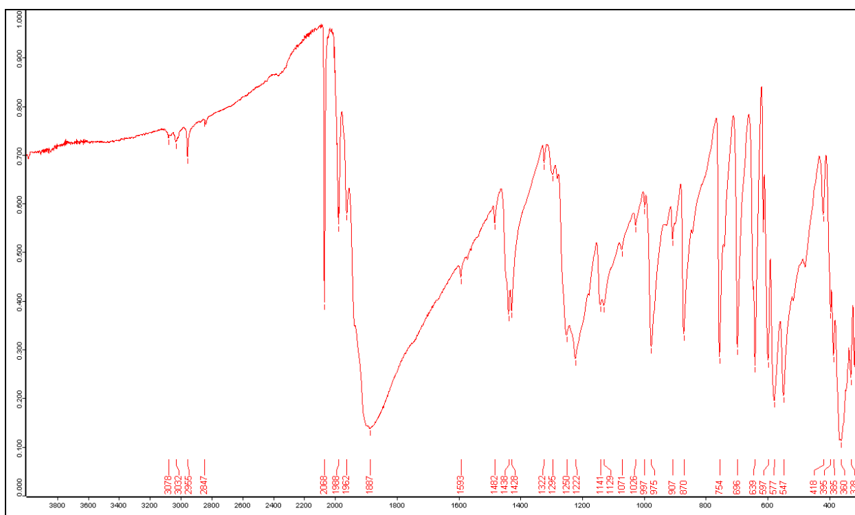
Figure SI 3.21 IR solid state (powder) spectrum of the Fischer carbene 3.2b .
