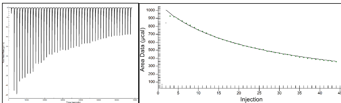
Figure SI 5.7. left side – ITC thermogram of the dissociation of the complex 5.1/5.2g (syringe, c=129.14 mM) in chlorobenzene. The titration was performed at 25^{\circ}\text{C} through 44 sequential additions (of 2.06 \mu\text{L} each). Time between two consecutive injections was 1500 s. Heat released is expressed in \mu\text{J/s} versus time in s. right side – ITC integrated heat peaks of the thermogram shown on the left side. Integrated heats are expressed in \mu\text{cal} versus number of injections and fitted by dimer dissociation model implemented in NanoAnalyze software.
