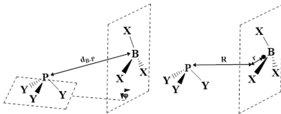
Figure M4 The geometrical parameters describing phosphine-borane interactions: a) d_{B-P} distance and angle \varphi , b) normal distance R and offset distance r . The X and Y are substituents on boron and phosphorus atoms, respectively. The dihedral angle \varphi is an angle between the planes formed by atoms directly bound to phosphorus and boron atoms.
