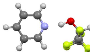
[5.3f] \Delta H_s = -12.7 kcal/mol; \Delta G_s = -2.1 kcal/mol; \Delta S_s = -35.3 kcal/mol
