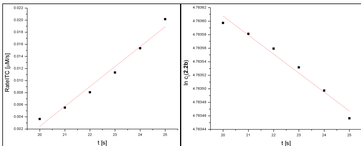
Figure 2.6 left side - Linear fit of the plot of the ITC Rate as a function of time for the reaction of 2.1 (sample cell, c=101.43 mM) with 2.2b (syringe, c=16.93 mM) carried out in ITC calorimeter. ITC Rate is expressed in \mu\text{M/s} and time in s. Obtained k = 3.3 \cdot 10^{-3} \pm 3 \cdot 10^{-4} , as the result of the fitting. right side - Linear fit of the plot of logarithm of 2.2b concentration as a function of time for the same reaction. Obtained k_{obs} = 2.8 \cdot 10^{-5} \pm 2 \cdot 10^{-6} as the result of the fitting.
