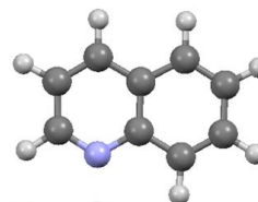
[5.3f] \Delta H_s = -12.7 kcal/mol; \Delta G_s = -2.1 kcal/mol; \Delta S_s = -35.3 kcal/mol
