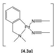
Scheme A1. Schematic representation of the studied reaction systems during the Thesis.
