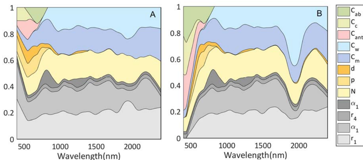
Figure 15 Normalized total sensitivity indices for differences in (A) reflectance and (B) transmittance between two faces of leaf as simulated by the FASPECT model. The area with different colors represents the normalized total sensitivity index of each input variable.
