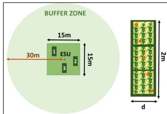
Figure 34 Spatial Sampling within an ESU. On the left, the circle represents the buffer zone with 30m radius centered on the ESU. The 15m x 15 m ESU includes three sub-samples where measurements are taken as illustrated on the right. The orange circles represent the position of the DHP camera for GAI estimates.
