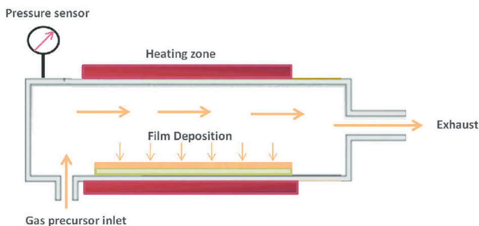
Figure 1.6. Schematic of chemical vapor deposition (CVD) reactor. Films are deposited on samples or substrates after high-temperature interaction and/or reactions of gaseous precursors
