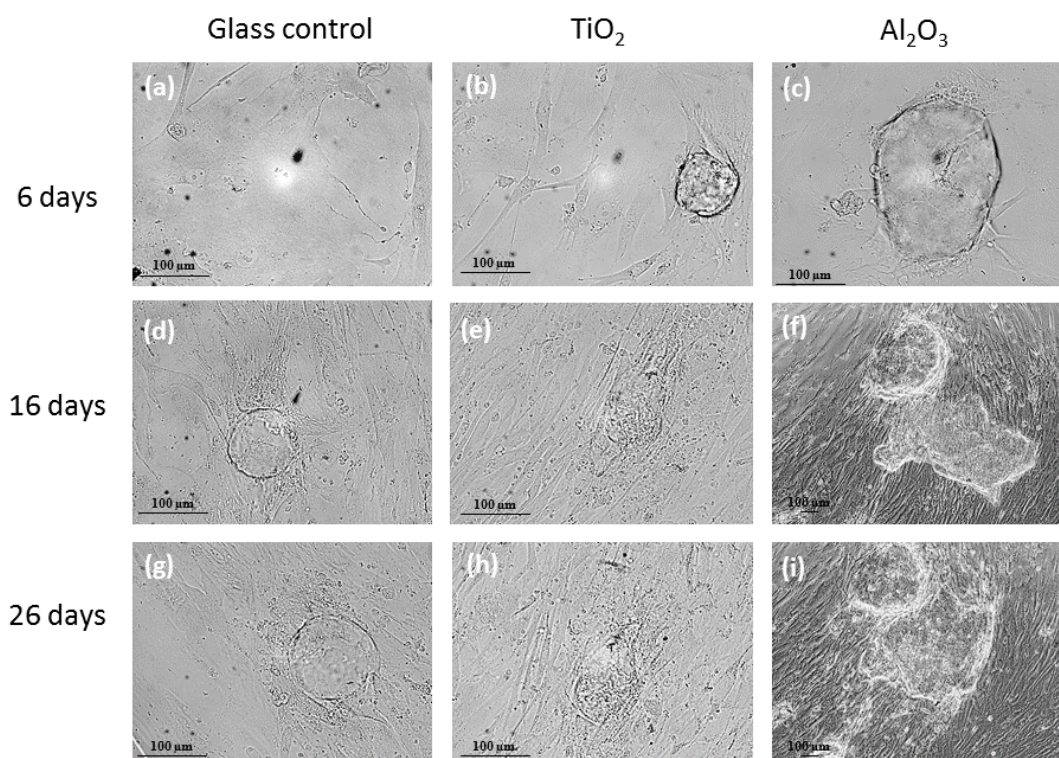
Figure 3.13. Phase contrast optical microscopy images of BMMSCs on glass control (a, d, g) , TiO 2 and Al 2 O 3 thin films (b, e, h and c, f, i, respectively) after 6, 16 and 26 days of cell culture.
