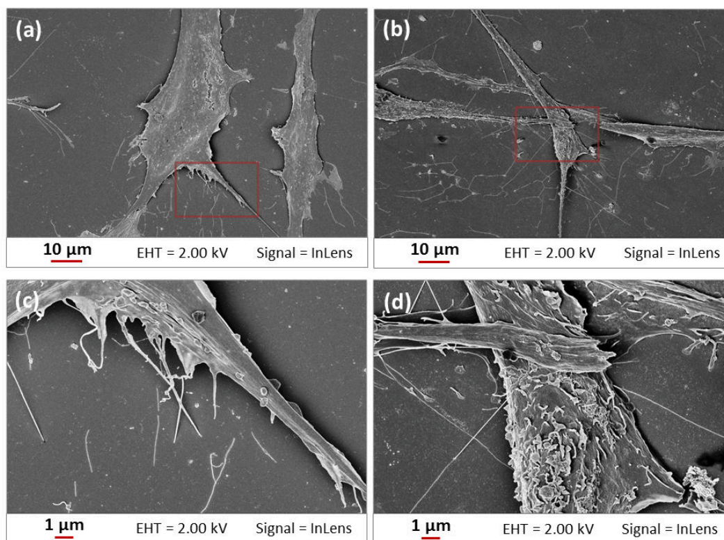
Figure 3.21. SEM images of glass control (a,c) and VO x -coated (b, d) substrates after 7 days of cell culture with magnification of ×1000 (top) and ×5000 (bottom).
