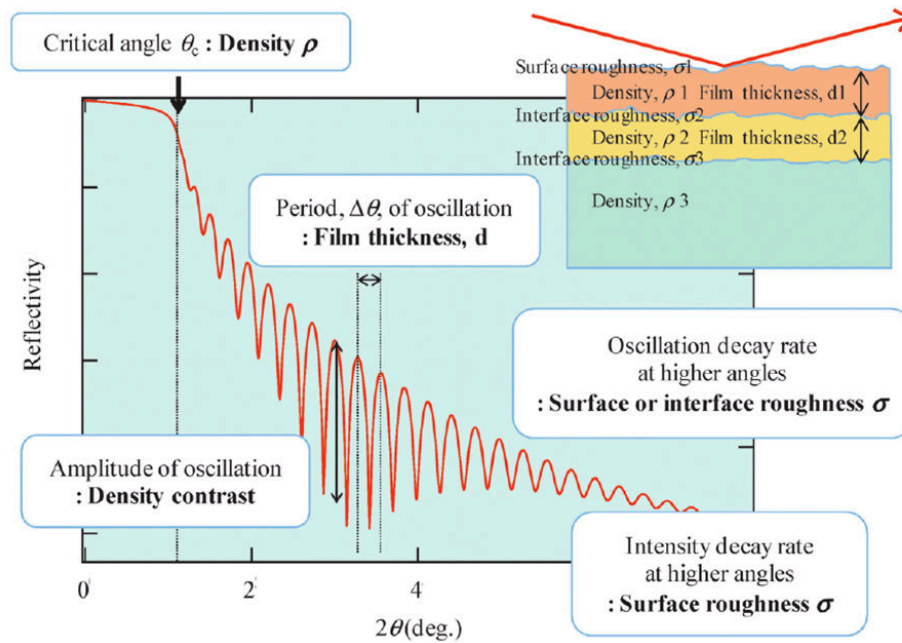
Figure 2.1. Information provided by X-ray reflectivity profile [2].
