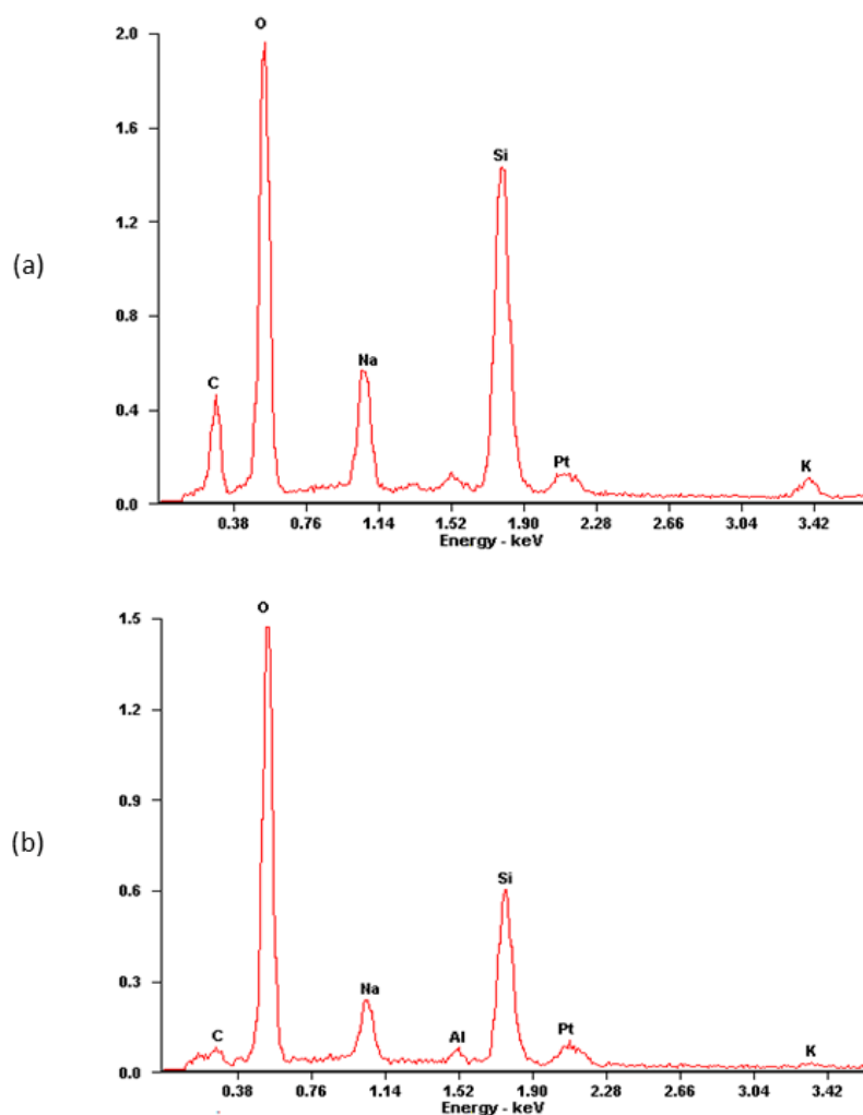
Figure 3.5. EDS pattern of TiO 2 (a) and Al 2 O 3 (b) thin films deposited at 300 and 200°C, respectively.
