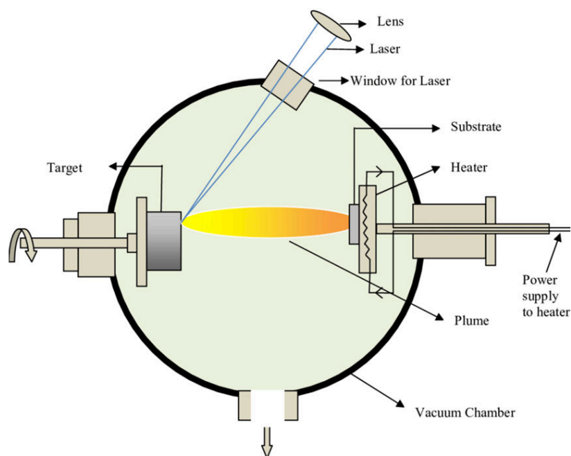
Figure 1.8. Schematic of PLD system. In this process films are grown as a result of thermal evaporation of the target material by laser ablation [112].
