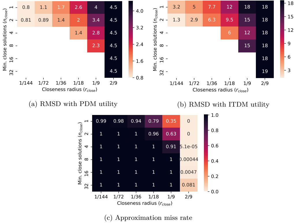
Figure 5.10 – Miss rate and root-mean-square deviation (RMSD) for the Average Distance (AD) approximation method using 100 known profiles.
