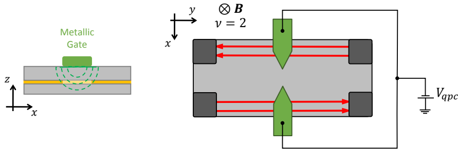
Figure 4.4: A quantum point contact nanostructure formed by two metallic finger placed on the surface of the GaAs heterostructure, which is only capacitively coupled to the 2DEG creating an electrostatic barrier for the electrons.
