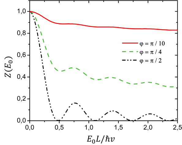
Figure 4.16: Elastic scattering probability Z(E_0) for a single electronic excitation, injected at a well defined energy E_0 above the Fermi Sea of an edge channel in the integer quantum Hall regime at filling factor \nu = 2 , after a propagation length L calculated by C. Grenier et al. [116, 115]. The calculations were performed at different coupling regimes given by the mixing angle \varphi .
