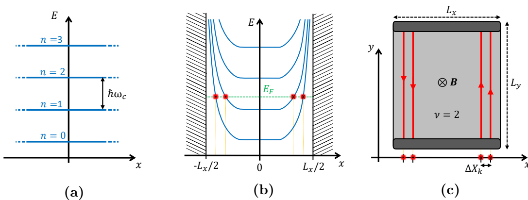
Figure 3.9: Formation of edge states for a 2DEG of spinless particles due to confinement imposed by the finite size of the system. (a) Flat Landau levels of an infinite 2DEG under a uniform magnetic field \mathbf{B} . (b) Landau level of a system with finite size L_x along the \hat{x} direction. The electric field \mathcal{E}_b created at the boundaries bends up the Landau levels. (c) Each time a Landau level crosses the Fermi level E_F it develops a chiral edge state on the sample located at the position of the crossing. The number of edge states is given by the filling factor \nu = 2 which indicates the number of filled Landau level at the bulk of the system. The center of motion of different edge states are spatially separated by \Delta X_k which depends on the sharpness of the confinement potential U .
