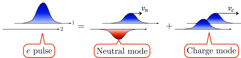
Figure 4.15: A wave packet injected in one edge channel fractionalizes into two modes: the slow neutral mode that propagates at a speed v_n and fast charge mode that propagates at a speed v_c . Picture adapted from Ref. [114].
