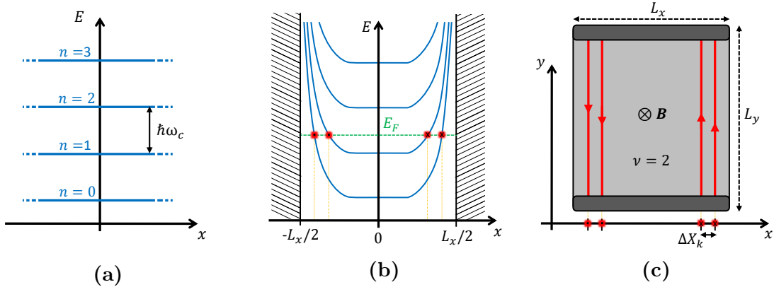
Figure 2.1: (a) Flat Landau levels E_n = \hbar \omega_c (n + 1/2) formed in an infinite 2DEG under a uniform magnetic field \mathbf{B} . (b) Landau level formed in a system with finite size L_x along the \hat{x} direction. The confinement potential created at the boundaries (here represented as hard walls) bends up the Landau levels. (c) Each time a Landau level crosses the Fermi level E_F in b, a chiral edge state develops on the sample located at the position of the crossing. The number of edge states is given the number of filled Landau level at the bulk of the system.
