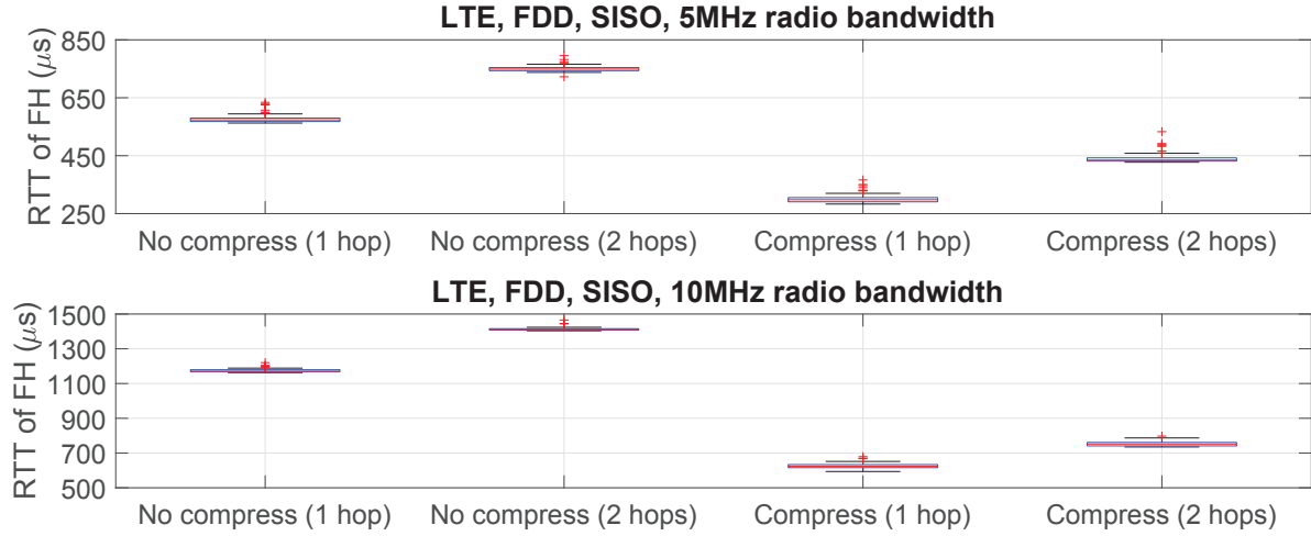
(a) RTT of FH for 5 MHz and 10 MHz radio bandwidth
