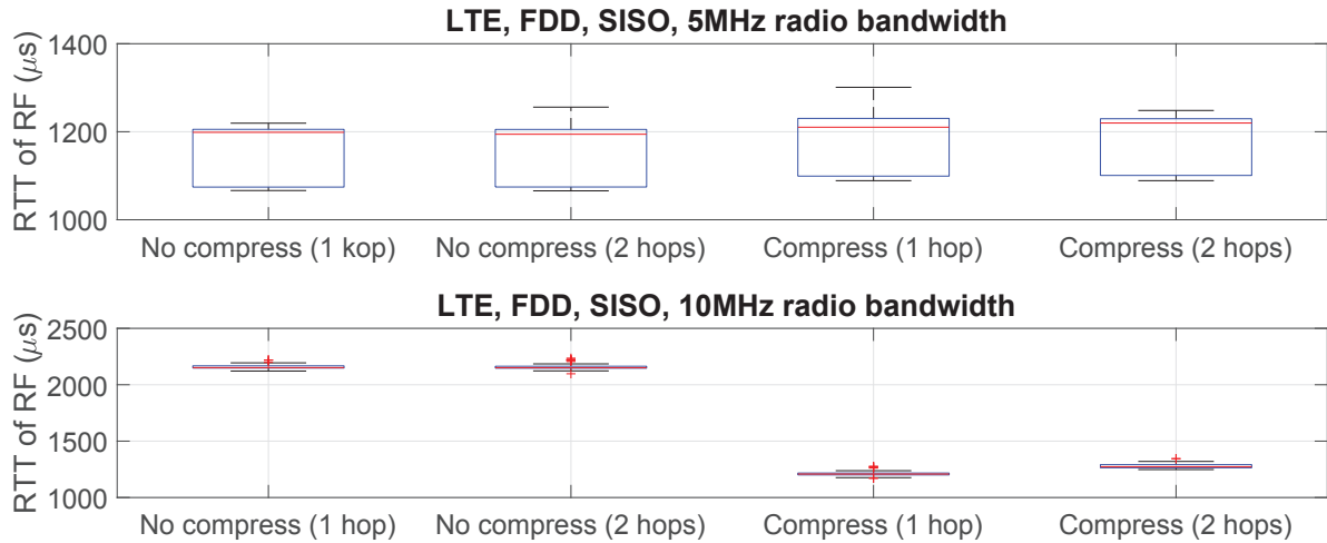
(b) RTT of RF front-end for 5 MHz and 10 MHz radio bandwidth
