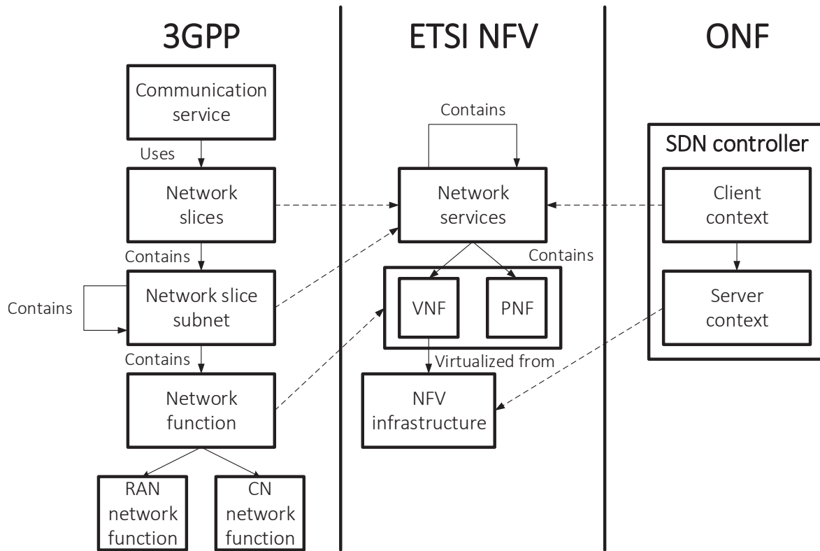
Figure 6.1: Mapping between the slicing information models of 3GPP, ETSI and ONF
