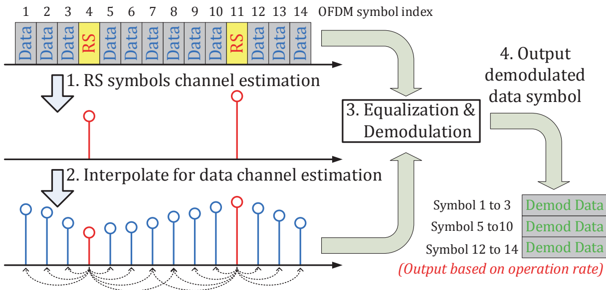
Figure 2.6: Channel estimation and demodulation processing
