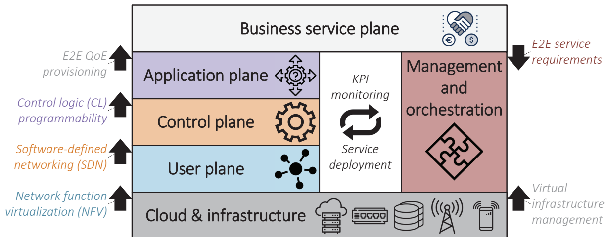
Figure 1.2: Overview of 5G architecture
