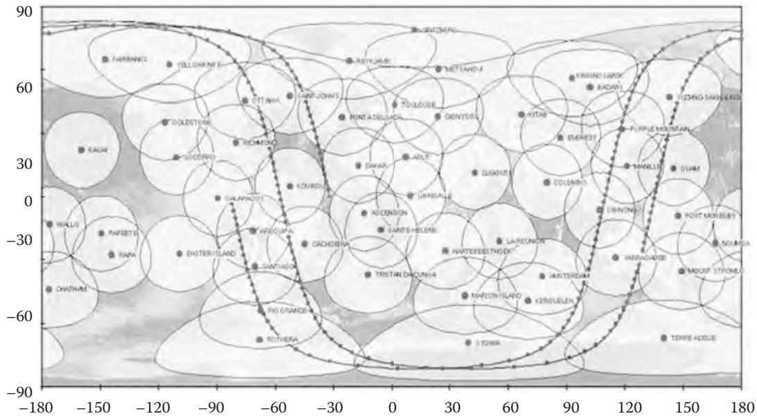
FIGURE 1.21 Envisat satellite ground track superimposed to DORIS station network visibility areas at ENVISAT altitude and 12° minimal elevation. (From Aviso website: https://www.aviso.altimetry.fr/en/my-aviso.html ).
