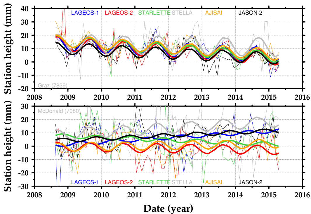
FIGURE 7.7: SLRF2014 height residual time series at Graz, 7839 (top), and McDonald, 7080 (bottom), between 2008.6 and 2015.3. LAGEOS-1, LAGEOS-2, Starlette, Stella, Ajisai, Jason-2 observations are plotted in blue, red, green, grey, orange, black, respectively. The solid curves are the results of the least squares fit to the time series of a bias, drift and annual periods.
