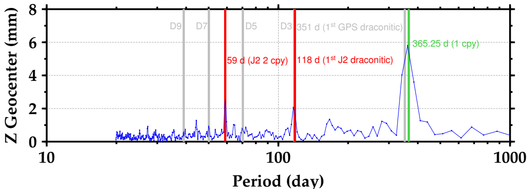
FIGURE 5.6: Amplitude spectra of the Z geocenter coordinate obtained using the Lomb-Scargle method for the 10 day estimates of GPS-derived geocenter motion from Jason-2 POE-F dynamic orbit series (July 2008 to January 2017; Cycles 1–315). The vertical lines mark the annual frequency, the first draconitic frequencies of Jason-2 and GPS, as well as their integer multiples.
