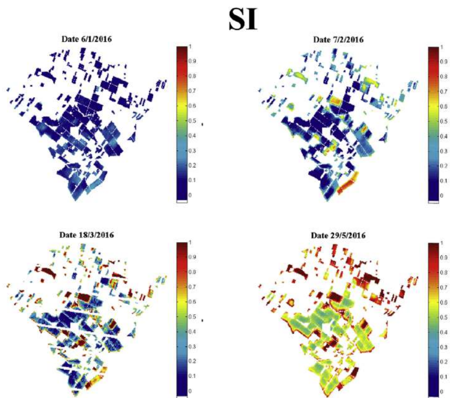
Fig. 9 – Time series of stress index (SI) maps estimated using Landsat data over R3 area.
