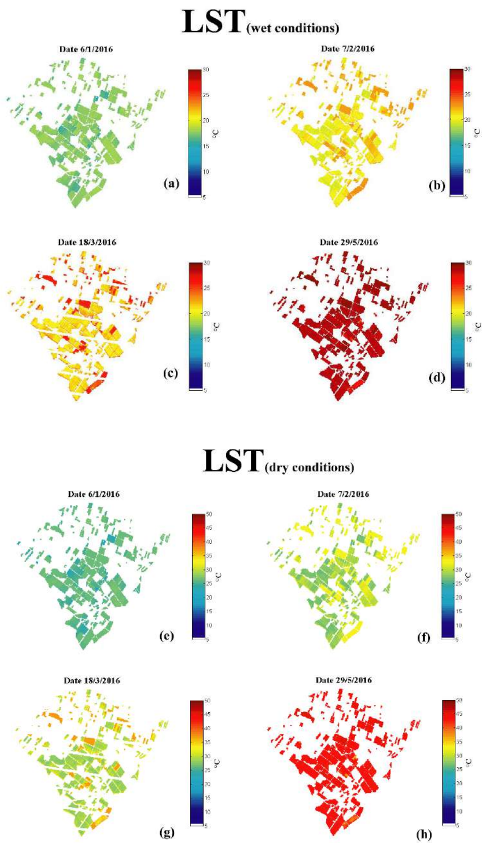
Figure IV.6: Time series of Land Surface Temperature (LST) maps in wet (a, b, c, d) and dry (e, f, g, h) conditions over R3 site on dates corresponding to different growing stages of wheat.
