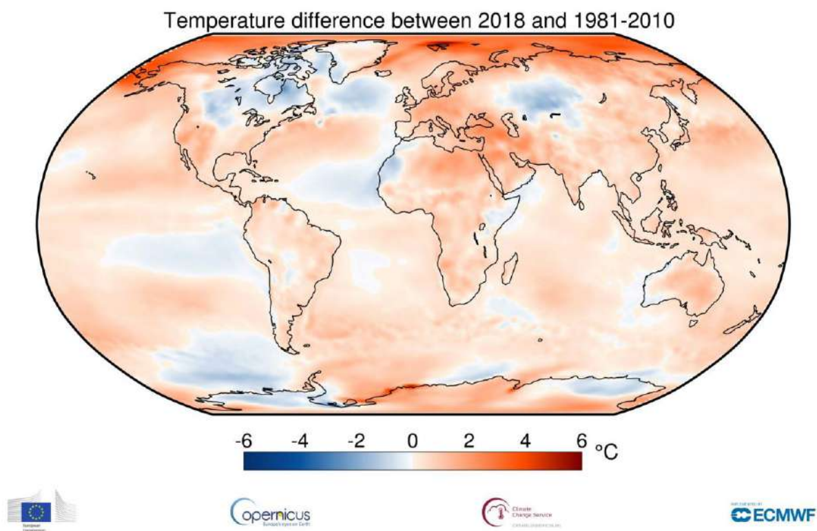
Figure 1: Temperatures anomaly between 2018 and the average 1981-2010. Source: ERA-Interim. 09-01-2019, (Credit: Copernicus Climate Change Service / ECMWF)
