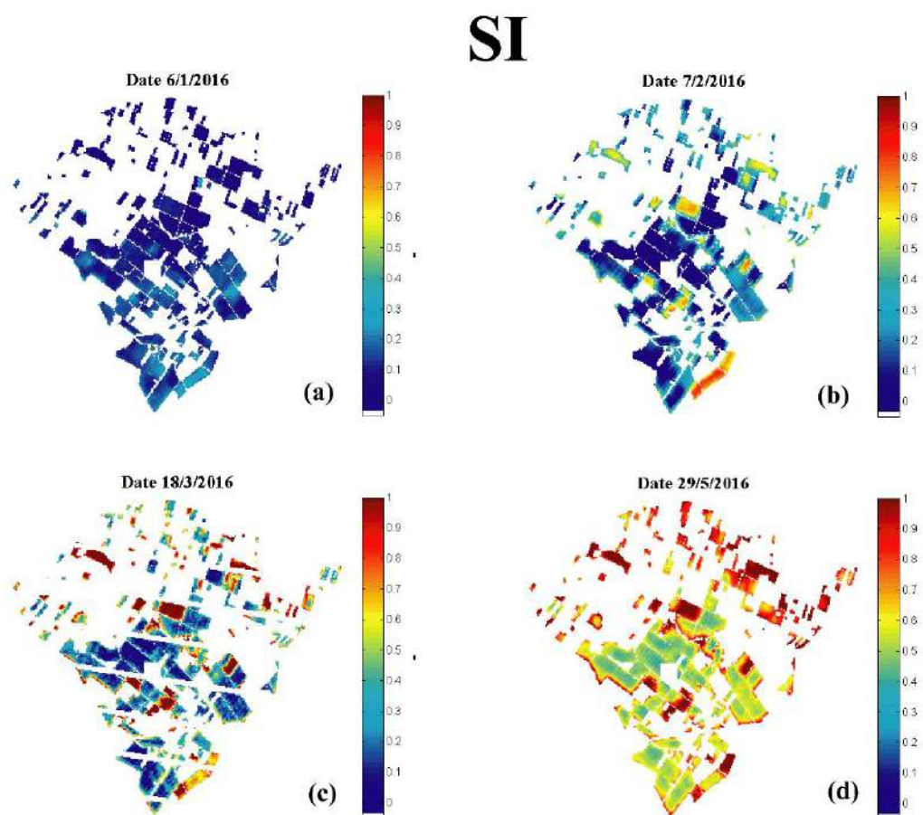
Figure IV.7: Time series of stress index (SI) maps estimated using Landsat data over R3 site.
