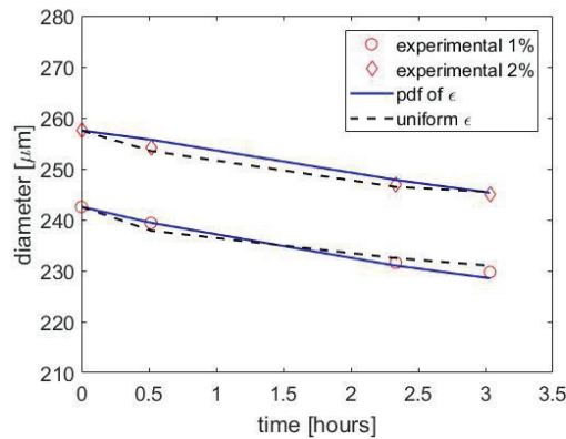
Figure 4.10: Parameters identification on oil in water experiments at 1% (circles) and 2% (rhombus) of Isane hold-up employing the pdf (blue) or assuming a uniform value (black) of \epsilon .
