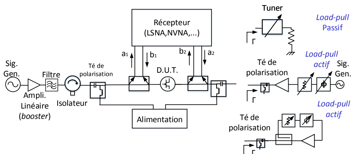
FIGURE 2.2 – Banc load-pull
