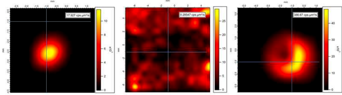
Figure 4.30: Field emission pattern at V_{tip} = 250 V in the case of no laser illumination (on the left) and increasing the laser peak intensity ( in center I_{laser} = 1.02 \cdot 10^3 GW/cm^2 and on the right I_{laser} = 2.04 \cdot 10^3 GW/cm^2 ).
