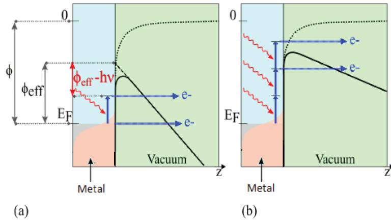
Figure 2.21: Laser assisted electron emission processes: (a) photo-assisted field emission; (b) multi-photon field emission.
