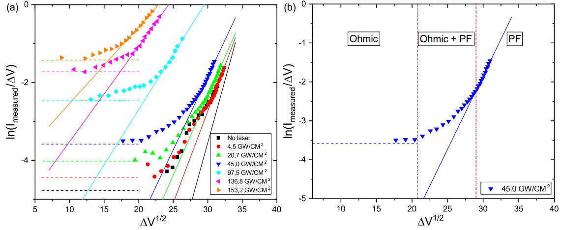
Figure 3.13: (a) I- \Delta V characteristic of the data presented Figure 3.12(a) represented in PF coordinates at T = 80\text{ K} , p_{He} = 4 \cdot 10^{-5}\text{ mbar} at different laser intensities (IR \lambda = 1030\text{ nm} ) and varying V_{\text{applied}} from 5 to 10 kV. The lines correspond to linear fits by the function: \ln(I_{\text{measured}}/\Delta V) = A + B\sqrt{\Delta V} ; (b) conduction zones corresponding on purely Ohmic conduction (left part), mixed Ohmic-PF conduction (central part) and purely PF conduction (right part).
