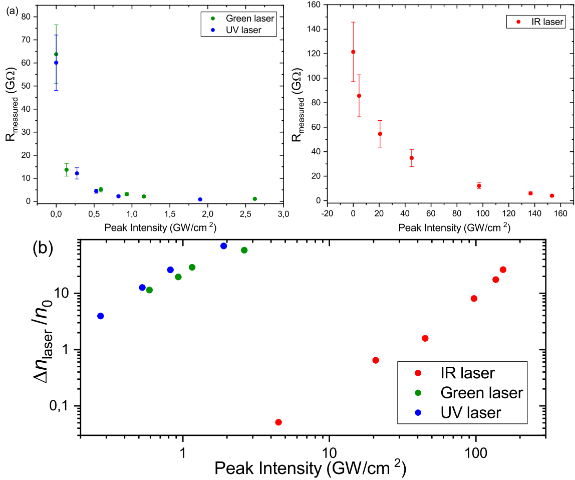
Figure 3.17: (a) Evolution of the measured resistance of the diamond needle at T = 80\text{ K} , p_{\text{He}} = 4 \cdot 10^{-5}\text{ mbar} for different laser peak intensity and wavelengths (Green, UV on the left and IR on the right). (b) Evolution of \frac{\Delta n_{\text{laser}}}{n_0} defined in Equation 3.10 for different laser peak intensity and for the three different wavelengths.
