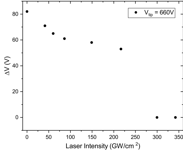
Figure 4.47: Voltage drop as a function of the laser peak intensity in the case of high applied voltage: V_{tip} = 660\text{ V} .
