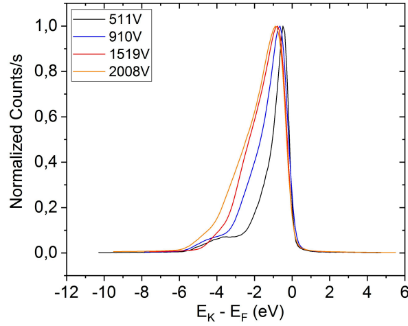
Figure 3.31: Energy spectra of diamond D5 taken at different applied voltages; Aperture 4, CAE 100 eV
