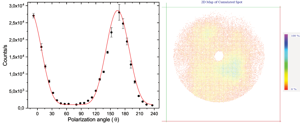
Figure 2.25: Laser assisted field emission from tungsten as a function of the laser polarization and relative emission pattern, taken at V_{applied} = 300\text{ V} and laser peak intensity I_{laser} = 50\text{ GW/cm}^2 . The fit is done with a \propto \cos^{2n}(\theta) curve where n = 3 indicating a three photon absorption process.
