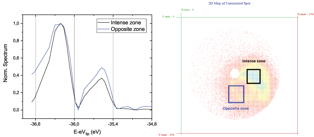
Figure 4.46: Two different emission spectra taken at V_{tip} = 80\text{ V} from two different regions of the emission ring pattern at I_{laser} = 279\text{ GW/cm}^2 .
