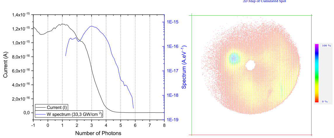
Figure 2.22: Field emission spectrum under laser illumination with I_{laser} = 33.3 \text{ GW/cm}^2 and at V_{applied} = 300 \text{ V} and relative emission pattern. The abscissa is calculated using (K_E - E_F)/\hbar\nu_{laser} in eV with \hbar\nu_{laser} = 1.2 \text{ eV} .
