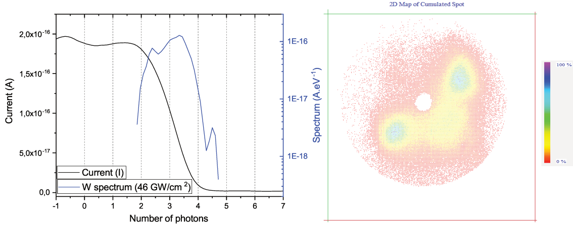
Figure 2.26: Field emission spectrum under laser illumination with I_{laser} = 46\text{ GW/cm}^2 and at V_{applied} = 350\text{ V} and relative emission pattern. The abscissa is calculated using (K_E - E_F)/\hbar\nu_{laser} in eV with \hbar\nu_{laser} = 1.2\text{ eV} .
