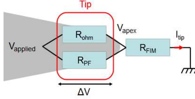
Figure 3.14: Electrical equivalent modellization for the conduction process inside diamond nano-needles.
