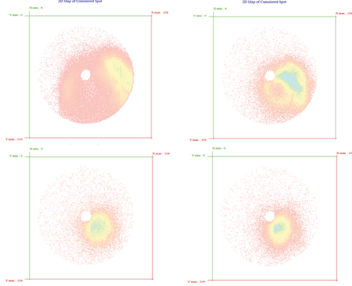
Figure 4.43: Field emission patterns at V_{tip} = 80 V increasing the laser peak intensity (top left I_{laser} = 279 GW/cm^2 , top right I_{laser} = 285 GW/cm^2 , bottom left I_{laser} = 314 GW/cm^2 and bottom right I_{laser} = 374 GW/cm^2 ).
