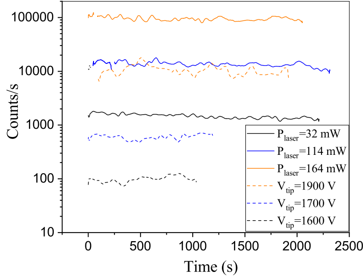
Figure 4.5: Emission currents as a function of time, full line correspond to laser assisted emission while dashed lines are emission currents in dark.
