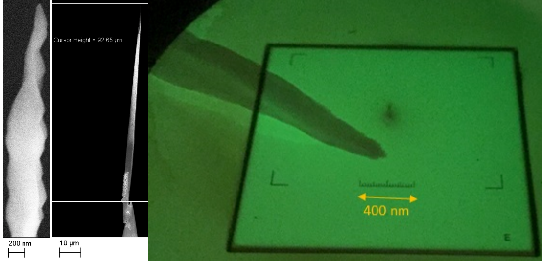
Figure 3.30: (a) Diamond D5, length \sim 90 \mu m , tip apex \sim 25 nm . (b) Diamond C6, length \sim 14 \mu m , tip apex \sim 25 nm
