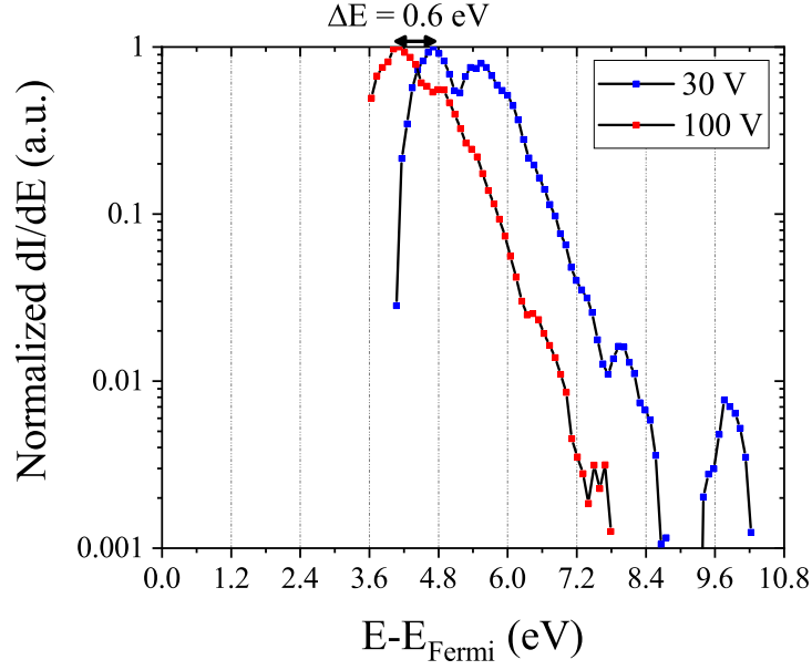
Figure 4.21: Electron energy spectra shift taken at 100 kHz with laser peak intensity of 18 GW/cm^2 for V_{tip} = 30 V (blue dots) and V_{tip} = 100 V (red dots).
