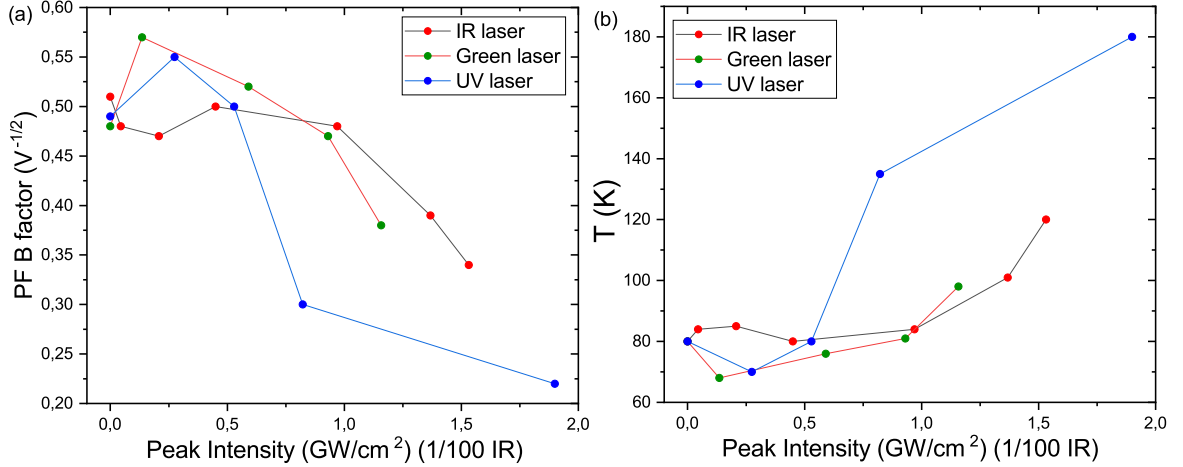
Figure 3.18: (a) Evolution of the Poole-Frenkel factor B and (b) evolution of the temperature T estimated using Equation 3.12, as function of the peak laser intensity and wavelength.
