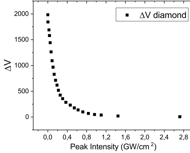
Figure 3.5: Voltage drop of a diamond sample in function of the laser peak intensity at constant applied voltage V_{\text{applied}} = 7.43 \text{ kV} , pressure p_{\text{He}} = 1.8 \cdot 10^{-5} \text{ mbar} . The laser has a wavelength \lambda = 343 \text{ nm} , at laser frequency 100 \text{ kHz} with pulse duration of 500 \text{ fs} .
