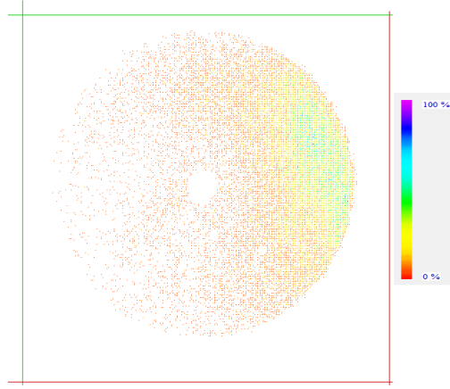
Figure 4.18: Emission pattern at V_{tip} = 100 V under laser illumination at 100 kHz at a laser peak intensity of 15 \text{ GW/cm}^2 . The associated emission spectrum is shown in Figure 4.19.
