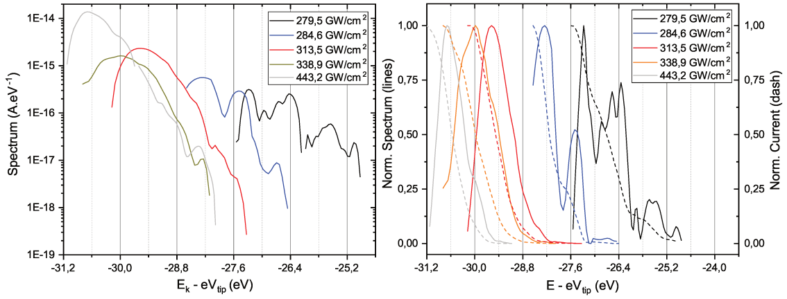
Figure 4.45: Energy spectra taken at V_{tip} = 80\text{ V} increasing the laser peak intensity, in semi-log scale (on the left) and linear scale (on the right).
