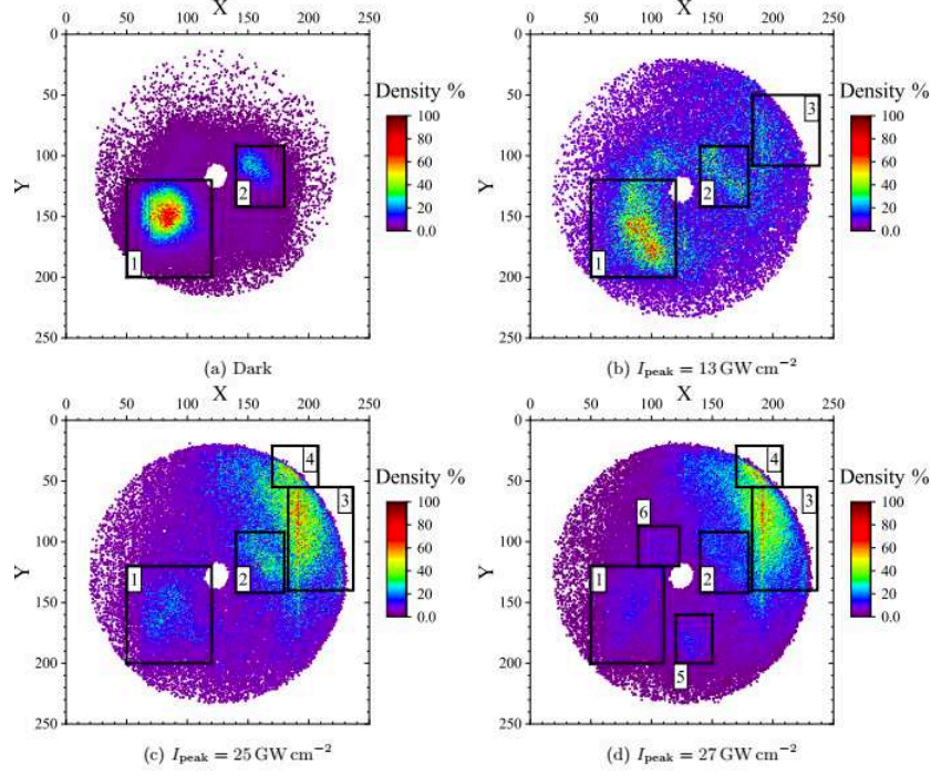
Figure 4.11: Emission pattern at V_{tip} = 300V : (a) in the dark; and under laser illumination at 37.5\text{ kHz} (b) I_{peak} = 13\text{ GW/cm}^2 (c) I_{peak} = 25\text{ GW/cm}^2 (d) I_{peak} = 27\text{ GW/cm}^2 . The (X ; Y) coordinates indicate the position on the CCD camera in number of pixels. The colors map corresponds to the normalized density of impacts.
