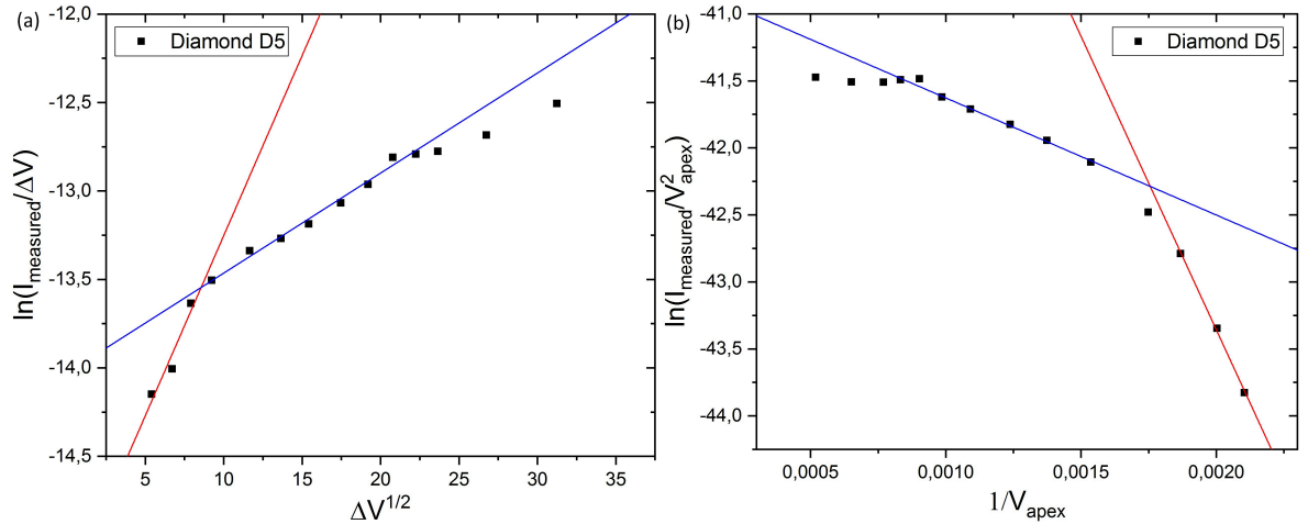
Figure 3.33: (a) \Delta V - V characteristic of the data presented in Figure 3.32(a) represented in PF coordinates. (b) The same data plotted in FN coordinates as a function of V_{apex} which is linked to the electric field at the diamond-vacuum junction.
