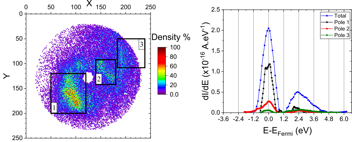
Figure 4.12: (left) Field emission pattern and (right) normalized energy spectra of the poles 1 (black dots), 2 (red dots), 3 (green dots) defined in (left), at V_{\text{tip}} = 300 \text{ V} under laser illumination with 37.5 \text{ kHz} repetition rate and I_{\text{peak}} = 13 \text{ GW/cm}^2 .
