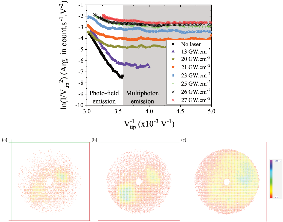
Figure 4.8: FN plots from diamond for different laser peak intensity at a repetition rate of 37.5\text{ kHz} . At high applied voltages (left side of the dashed line) the I - V characteristic is linear in FN coordinates corresponding to photo-field emission while at low applied voltages (right side of the dashed line) the I - V characteristic is constant in FN coordinates denoting multi-photon above barrier emission regime. Emission patterns during FN measurements taken in (a) dark regime(no laser illumination), (b) at 13\text{ GW/cm}^2 and (c) at 26\text{ GW/cm}^2 .
