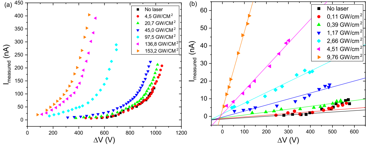
Figure 3.12: I - \Delta V characteristic at T = 80\text{K} . (a) variation of V_{\text{applied}} between 5 and 10 kV at different laser intensities powers (IR \lambda = 1030\text{ nm} , and p_{\text{He}} = 4 \cdot 10^{-5}\text{ mbar} ); (b) variation of p_{\text{He}} between 10^{-7} and 5 \cdot 10^{-5} at V_{\text{applied}} = 5\text{ kV} and different IR laser powers. The linear fit are of the function I_{\text{measured}} = (1/R_{\text{measured}})V_{\text{apex}} , R_{\text{measured}} varying from 120 \pm 34\text{ G}\Omega (no laser) to 1.8 \pm 0.2\text{ dG}\Omega ( 28\text{ mW/cm}^2 ).
