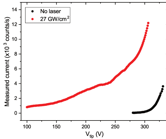
Figure 4.4: I-V characteristic of electron emission obtained in dark (black dots) and under laser illumination at 37.5\text{ kHz} (red dots).
