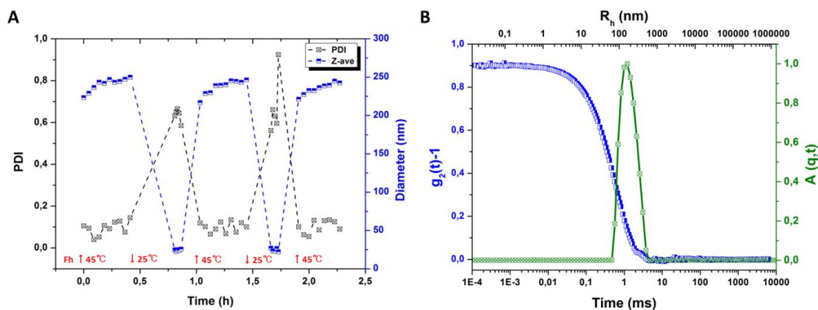
Figure 2. (A) Z-average size and polydispersity as a function of time upon repeated fast heating (45 °C) and cooling (25 °C) of Dex- b -ELP (125 \mu M) in water on DLS. (B) DLS autocorrelation function ( g_2(t)-1 ) and relaxation-time distribution ( A(q,t) ) for Dex- b -ELP (125 \mu M) in water at 45 °C, 90°.
