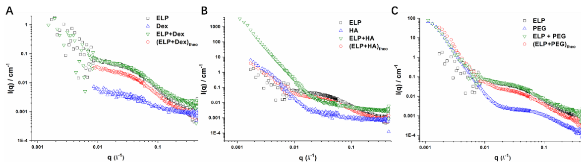
Figure S16. SANS curves of ELP, polysaccharide, their physical mixture and theoretical mixture curves in D_2O at the temperature below T_t . (A) Dex- b -ELP, (B) HA- b -ELP, (C) PEG- b -ELP. Theoretical mixture curves were normalized with concentration.
