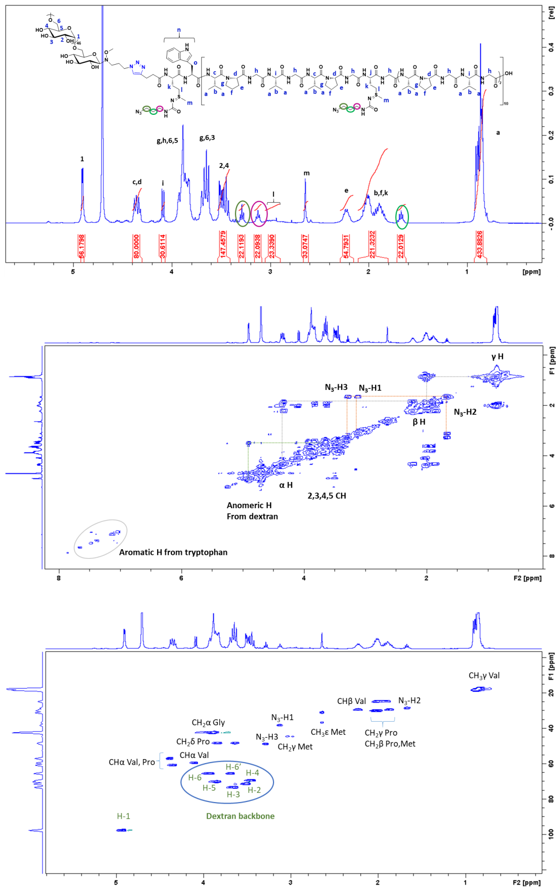
Figure 3. 1 H, COSY and HSQC NMR spectra of Dex- b -ELP OX -N 3 in D 2 O at 25 °C.
