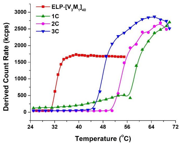
Figure S6. Scattered light intensity of ELP[V 3 M 1 -40], compound 1C, 2C and 3C at 125 \mu M in Mili-Q water as function of temperature.
