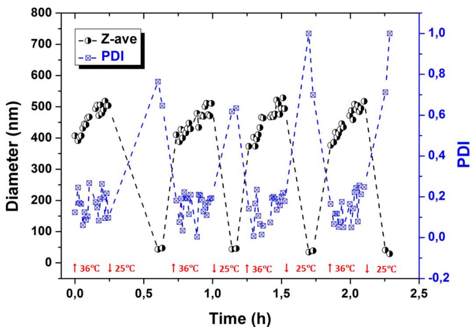
Figure S19. Z-average size and polydispersity as a function of time upon repeated fast heating (36 ^\circ\text{C} ) and cooling (25 ^\circ\text{C} ) of Lam- b -ELP.
