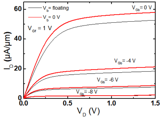
Figure 2.11: Output of I_D(V_D) characteristics of 5-terminal ultrathin FDSOI MOSFETs measured with the body contact grounded or floated. V_{Gf} = 1 V, t_{si} = 8 nm, t_{BOX} = 25 nm, W = 10 \mu\text{m} , and L_G = 5 \mu\text{m} .
