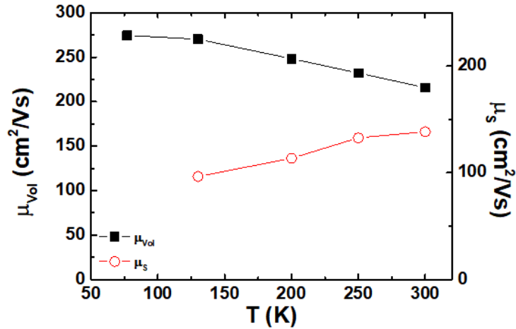
Figure 4.18: Bulk \mu_{vol} and surface mobility \mu_s as a function of temperature T .
