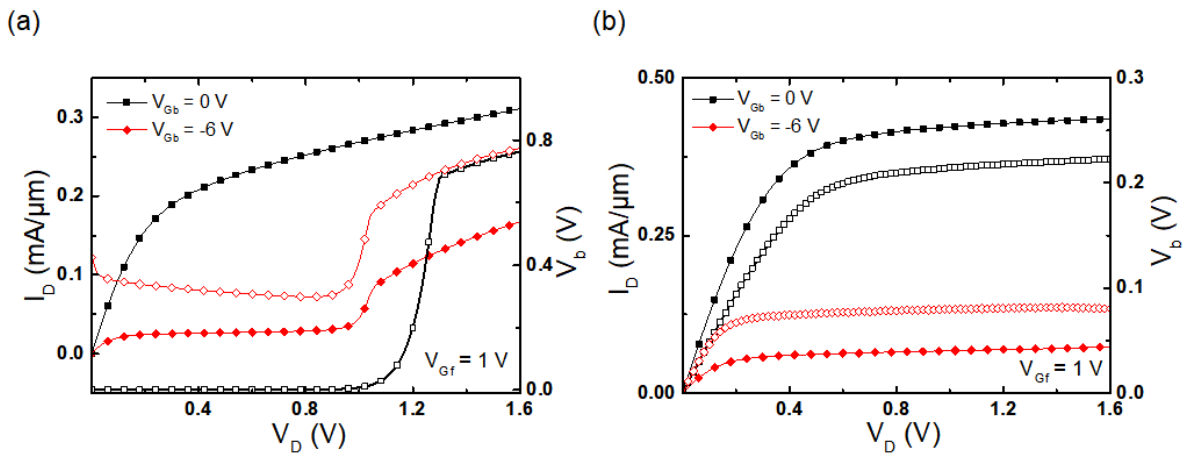
Figure 3.8: I_D(V_D) characteristics with measured body potential variation in (a) a thick ( t_{Si} = 25 nm) and (b) an ultrathin ( t_{Si} = 8 nm) MOSFET. t_{BOX} = 25 nm, t_{ox} = 2.9 nm and L_G = 100 nm. V_{Gf} = 1 V and V_{Gb} = 0, -6 V.
