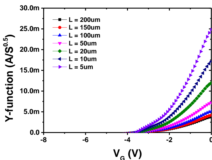
Figure 4.12: Y-function in depletion regime Y_{\text{vol}}(V_G) for 200 nm thick InGaAs devices with different gate lengths. For W = 10 \mu\text{m} and V_D = 0.2 \text{ V} .
