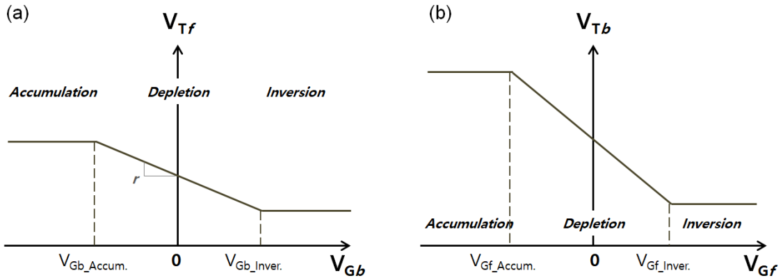
Figure 1.15: The classical inter-gate coupling model proposed by Lim and Fossum for (a) front- and (b) back-interface threshold voltage. Three distinct domains can be indicated, depending on the opposite interface conditions: accumulation, depletion, and inversion, respectively.
