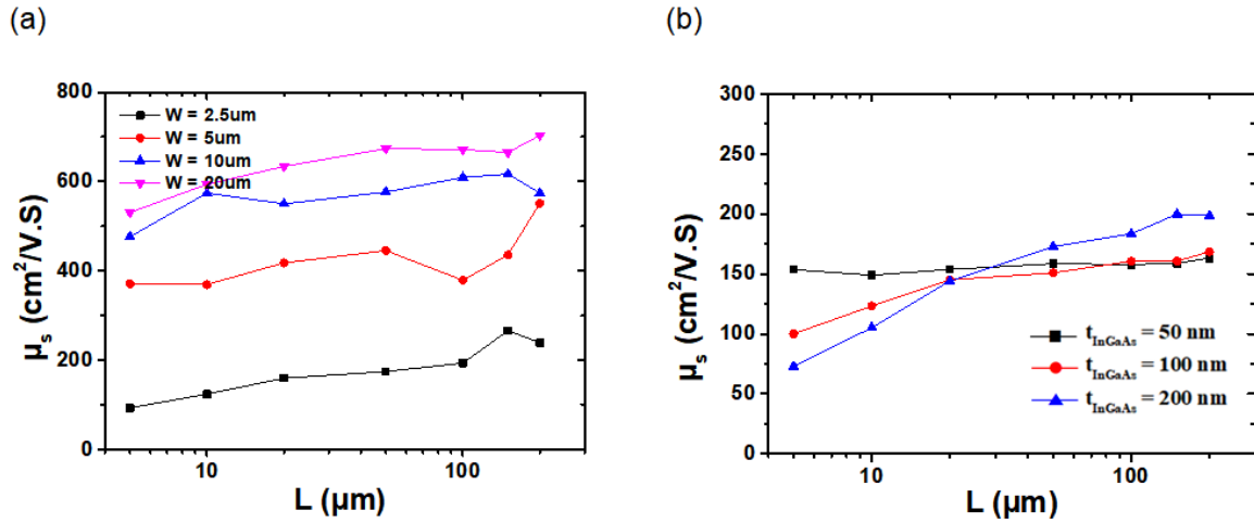
Figure 4.16: Extracted surface mobility versus gate length in (a) 200 nm thick devices with different widths, and (b) narrow devices of 2.5 \mu\text{m} with variable thickness. V_D = 0.2 \text{ V}
