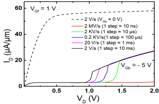
Figure 2.20: Transient simulation of output characteristics for a unit step time increased from 10 ns to 10 ms, respectively. V_{Gf} = 1 V, V_{Gb} = -5 V, t_{si} = 25 nm, t_{BOX} = 25 nm, W = 10 \mu m, L = 1 \mu m.
