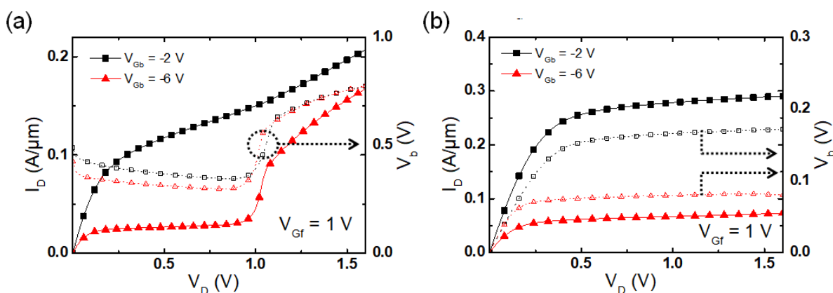
Figure 2.9: Output DC characteristics and corresponding body potential V_b in FD-SOI MOSFETs with variable Si film thickness. (a) t_{Si} = 25 nm, (b) t_{Si} = 7 nm, L_G = 100 nm and t_{BOX} = 25 nm.
