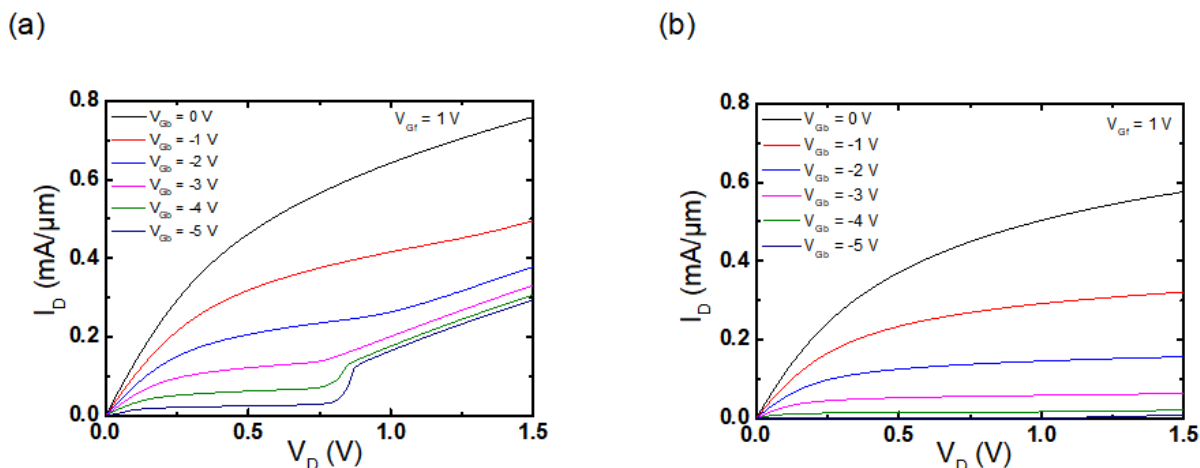
Figure 2.19: Simulated I_D(V_D) characteristics for different back-gate voltages: (a) t_{Si} = 25\text{ nm} , (b) t_{Si} = 8\text{ nm} . L = 100\text{ nm} , t_{BOX} = 25\text{ nm} , V_{Gf} = 1\text{ V} , V_{Gb} = 0 to -5\text{ V} .
