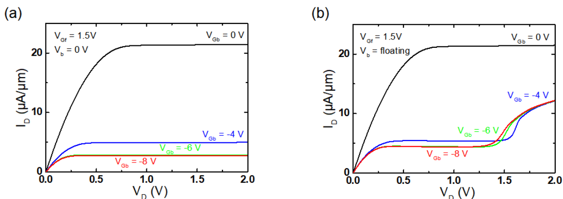
Figure 2.8: Comparison of I_D(V_D) characteristics of 5-terminal FDSOI MOSFETs measured with the body contact (a) V_b = 0 V; the excess holes are expelled through the grounded body as in bulk silicon device or (b) the body floating condition as for SOI device. V_{Gf} = 1.5 V, t_{Si} = 25 nm, t_{BOX} = 25 nm, W = 10 \mu m, and L_G = 5 \mu m.
