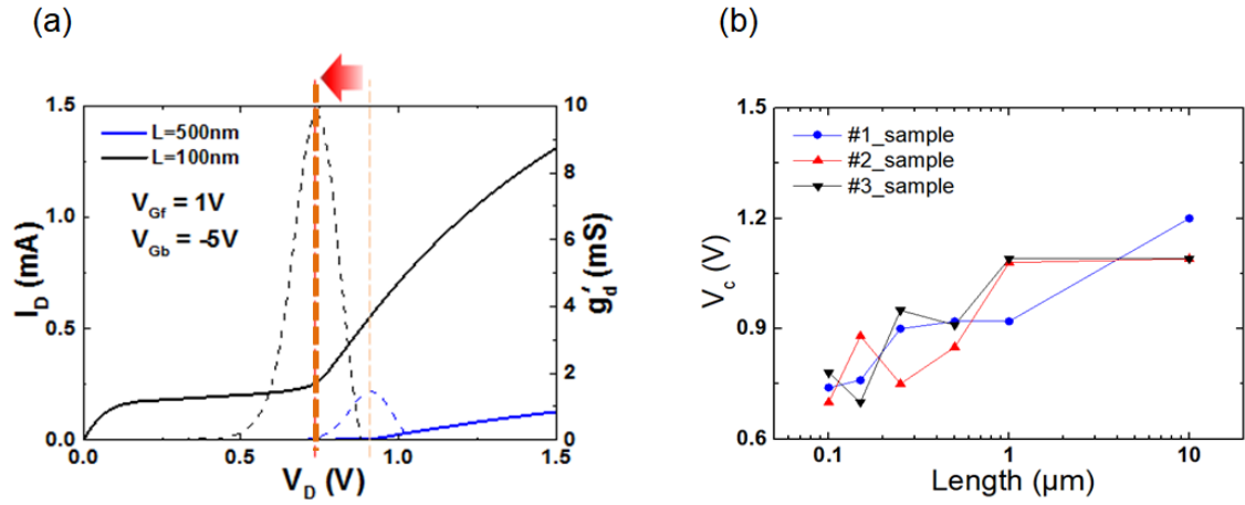
Figure 2.6: (a) Experimental I_D(V_D) characteristic and output conductance g'_d(V_D) curves for L = 500\text{ nm} and 100\text{ nm} . (b) The critical voltage V_c tendency extracted from the peak of output conductance versus channel lengths. For V_{Gf} = 1\text{ V} , V_{Gb} = -5\text{ V} and W = 10\text{ }\mu\text{m} .
