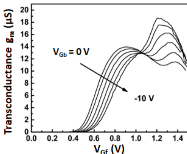
Figure 2.25: Transconductance vs. front-gate voltage in FDSOI n-MOSFET showing the impact of GIFBE. t_{ox} = 1.6 nm, t_{Si} = 17 nm, t_{BOX} = 145 nm, V_D = 0.1 V [11].
