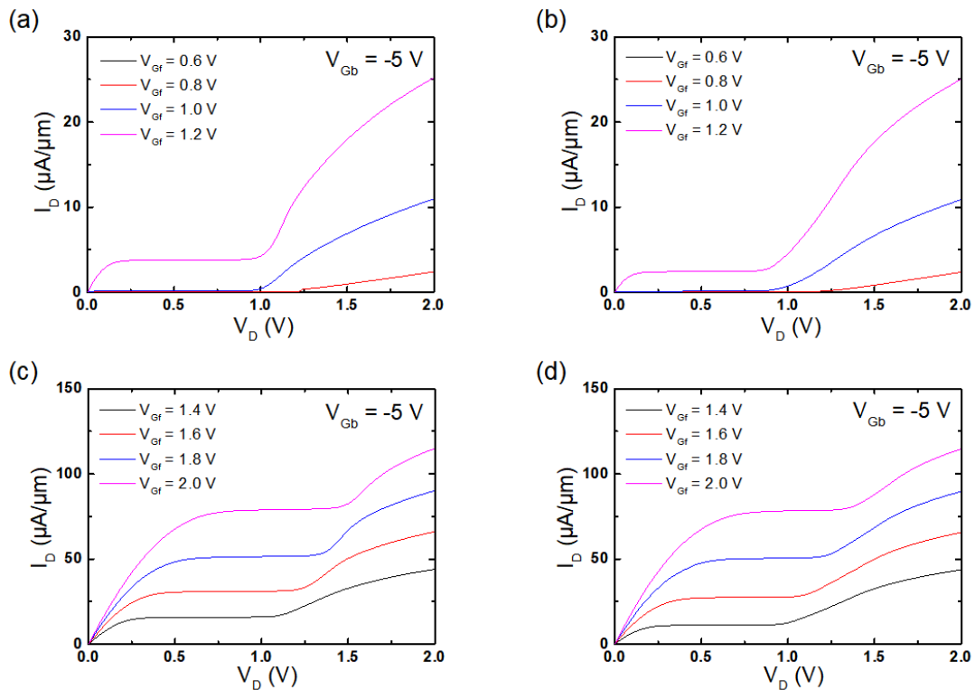
Figure 2.7: Comparison of output characteristics with different front gate voltages (from 0.6\text{ V} to 2.0\text{ V} ) between the normal n-MOSFET (a, c), and H-gate body contact n-MOSFET with floating body (b, d). For t_{Si} = 25\text{ nm} , t_{BOX} = 25\text{ nm} , L = 1\text{ }\mu\text{m} and W = 10\text{ }\mu\text{m} .
