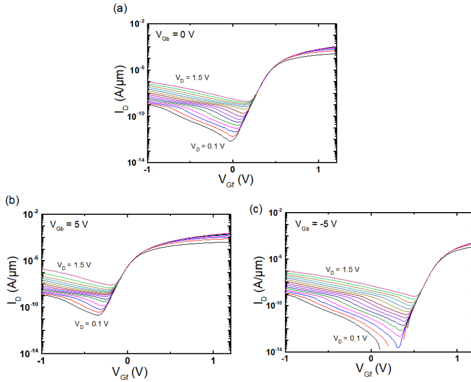
Figure 2.36: Experimental drain current characteristics, from low (0.1 V) to high drain bias (1.5 V), as a function of the front-gate voltage with different back-gate biases. (a) V_{Gb} = 0 \text{ V} , (b) V_{Gb} = 5 \text{ V} , and (c) V_{Gb} = -5 \text{ V} , respectively. t_{Si} = 8 \text{ nm} , t_{BOX} = 25 \text{ nm} , W = 10 \mu\text{m} , L = 1 \mu\text{m} .
