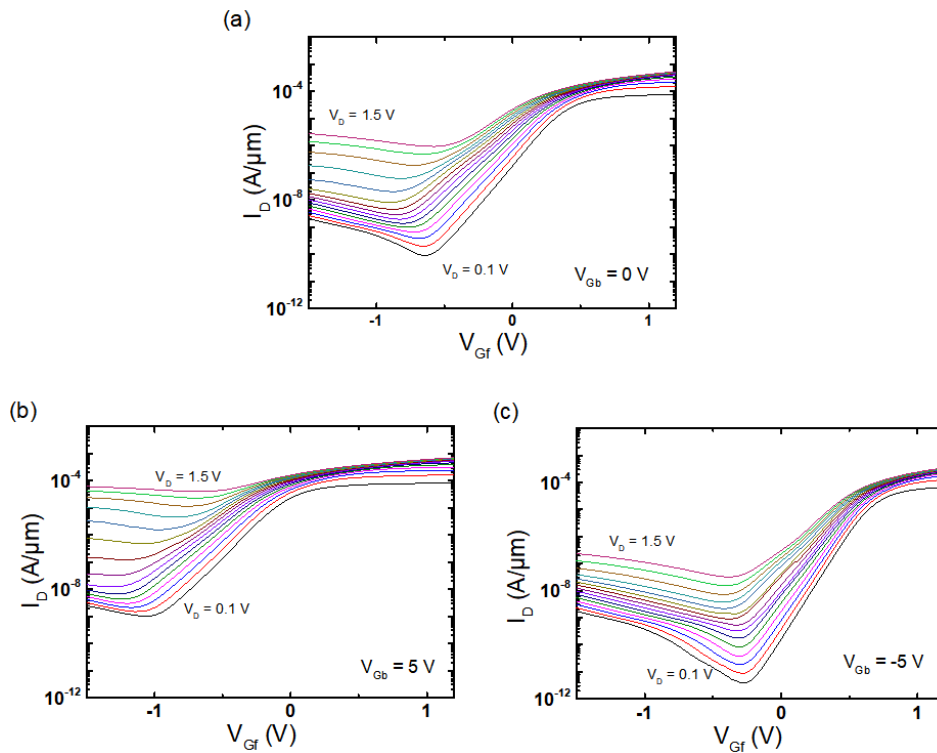
Figure 2.37: Experimental drain current characteristics for a short channel device with different back-gate biases (a) V_{Gb} = 0 \text{ V} , (b) V_{Gb} = 5 \text{ V} , and (c) V_{Gb} = -5 \text{ V} . t_{Si} = 8 \text{ nm} , t_{BOX} = 25 \text{ nm} , W = 10 \mu\text{m} , L = 30 \text{ nm} .
