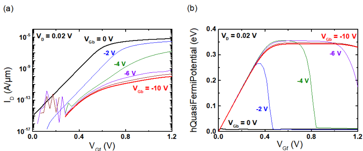
Figure 3.29: TCAD device simulation of (a) I_D ( V_{Gf} ) versus front-gate bias and (b) Quasi-Fermi potential for holes. t_{Si} = 8\text{ nm} , t_{BOX} = 25\text{ nm} , L_G = 100\text{ nm} , V_D = 0.02\text{ V} , and V_{Gb} = 0\text{ V} to -10\text{ V} (step = -2\text{ V} ).
