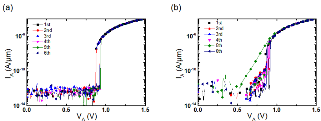
Figure 4.30: (a) I_A ( V_A ) characteristics without light, and (b) with light. For V_{Gf} = V_{Gb} = 0 V, L_G = 2 \mu\text{m} , L_i = 0.5 \mu\text{m} .
