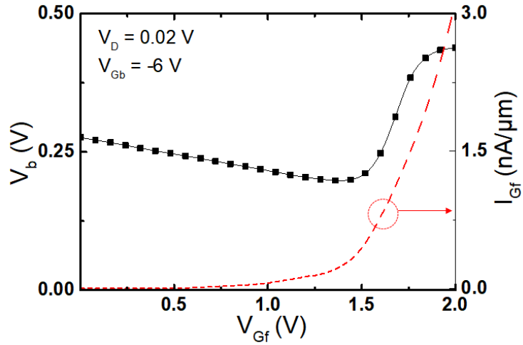
Figure 3.10: Correlation between measured V_b and gate current I_{Gf} versus front-gate bias. t_{Si} = t_{BOX} = 25 nm, t_{ox} = 2.9 nm and L_G = 1 \mu\text{m} . V_D = 0.02 V, V_{Gb} = -6 V.
