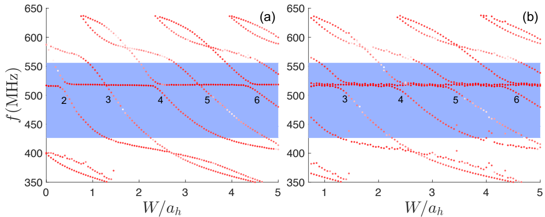
FIGURE 5.17 – Love modes eigenfrequencies as a function of the cavity width when (a) a pillar is placed in the center of the cavity; (b) two pillars are inserted respectively at the two edges of the cavity. Blue zone is the predicted band gap of the perfect holey PnC. The numbers denote the order of the fundamental cavity modes. r_h=0.2a , r_p=0.18a_p , H=2.4\mu\text{m} , h = 0.6a_p , a = 4\mu\text{m} , a_p = 2\mu\text{m} . Holey PnC size is three on each side of the cavity.
