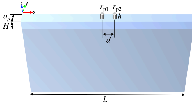
FIGURE 4.6 – Unit cell of two lines of cylindrical Ni pillars on the \text{SiO}_2 film deposited on a 90ST-cut quartz. The period is a_p along the y direction. Love waves propagate along the x -axis. r_{p1}=r_{p2}=0.2a_p , h=0.6a_p , H=2.4\mu\text{m} , L=20a_p , a_p=2\mu\text{m} .
