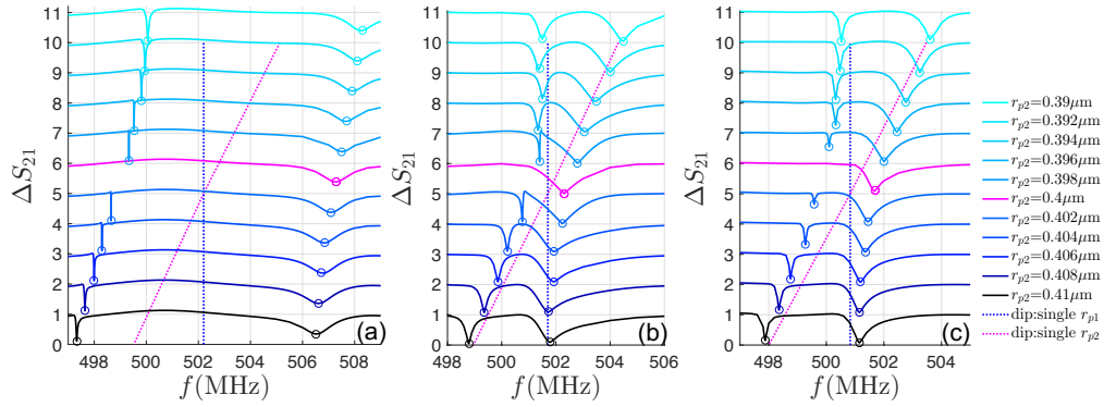
FIGURE 4.27 – Normalized transmission spectra of Love waves for a_p = (a) 1\mu\text{m} , (b) 2\mu\text{m} and (c) 4\mu\text{m} , when gradually changing r_{p2} from 0.39\mu\text{m} to 0.41\mu\text{m} . Dotted blue and rose lines indicate the single pillar dip frequencies with a periodicity of 2a_p and a radius equal to r_{p1} and r_{p2} , respectively. r_{p1}=0.4\mu\text{m} .
