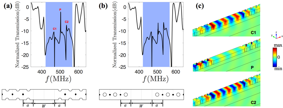
FIGURE 5.12 – Transmission spectra for the defect-included (a) Ds-PnC and (b) Ls-PnC with W = 5a . Blue zones denote the corresponding band gap of the two perfect PnC. (c) Displacement fields U_y of the cavity modes C1, C2 and pillar mode P for the defect-included Ds-PnC. r_h = 0.2a , r_p = 0.1a , h = 0.3a , H = 0.6a , a = 4\mu\text{m} , N_{PnC} = 4 .
