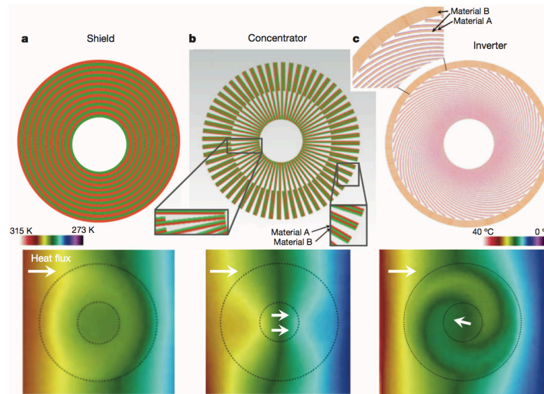
FIGURE 1.30 – Thermal meta-materials : (a) A thermal shield (top), bottom shows corresponding measured temperature profile for horizontal heat flux (white arrow). (b) A thermal concentrator. (c) A thermal inverter. [190]
