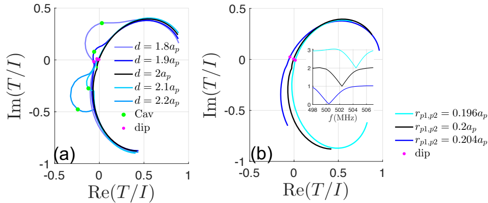
FIGURE 4.9 – (a) Complex plots of the normalized transmission in the frequency range [500, 505] MHz for d varies from 1.8a_p to 2.2a_p . The rose and green marks correspond to the dip and cavity mode frequencies, respectively. r_{p1}=r_{p2}=0.2a_p . (b) Complex plots of the normalized transmissions for d = 2a_p \approx \lambda/2 when all the pillars' radius vary from 0.196a_p to 0.204a_p . Inset shows the transmission spectra of corresponding curves.
