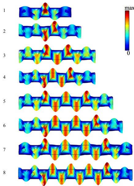
FIGURE 5.6 – Displacement and deformation in xy plane corresponding to cavity modes of different orders (from 1 to 8). r_h = 0.2a , H = 0.6a , a = 4\mu\text{m} , N_{PnC} = 3 .
