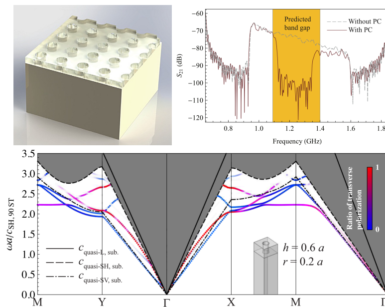
FIGURE 1.20 – (a) Schematic of the PnC composed of holes etched on a \text{SiO}_2 plate deposited on a quartz substrate; (b) Transmission of Love waves through the PnC along the direction \Gamma X ; (c) PnC band structure. Red indicates Love modes, blue indicates Rayleigh modes. [12, 131]
