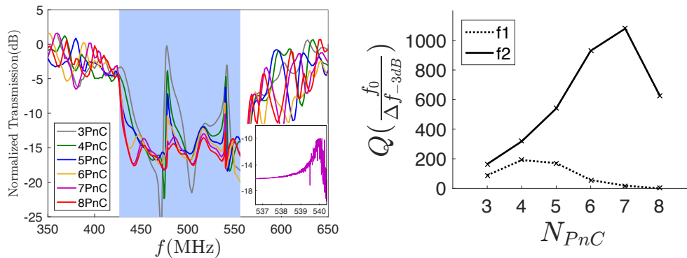
FIGURE 5.8 – (a) Transmission spectra of the PnC containing the defect, with the number of PnC holes on each side of the cavity varies from 3 to 8. Blue zone is the predicted band gap of the perfect PnC. Inset shows the zoomed peak at 540 MHz for N_{PnC} = 7 ; (b) Quality factors of the defect modes as a function of the number of PnC holes on each side of the cavity. W = 5a , r = 0.2a , H = 0.6a , a = 4\mu\text{m} .
