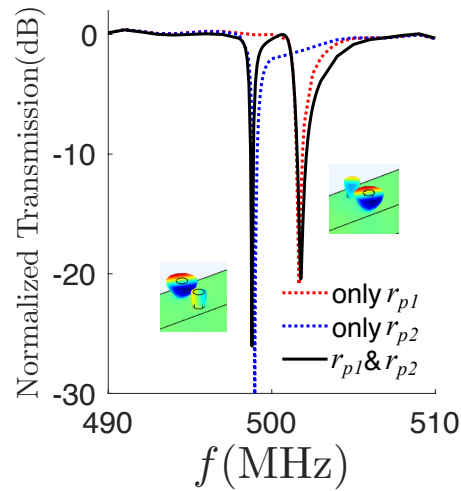
FIGURE 4.22 – Normalized transmission spectra of Love waves through the pillar line. u_y for two dipoles are shown aside. r_{p1} = 0.2a_p , r_{p2} = 0.205a_p . H = 2.4\mu\text{m} , a_p = 2\mu\text{m} .
