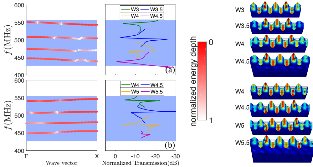
FIGURE 5.7 – Normalized transmission spectra for the defect-included holey PnC on the (a) 5 th and (b) 6 th cavity mode. Corresponding dispersion curve for each peak is shown on the left. Blue zones denote the predicted band gap of the perfect PnC. The displacement field of each mode at point X is shown on the right side. r_h = 0.2a , H = 0.6a , a = 4\mu\text{m} , N_{PnC} = 4 .
