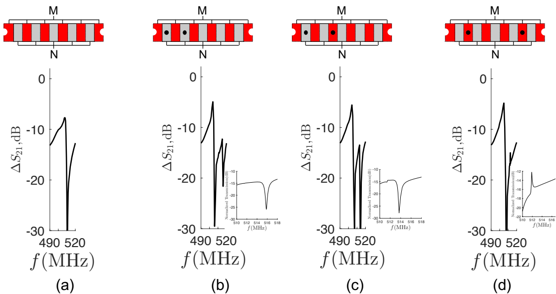
FIGURE 5.21 – (a)Transmission curve of Love waves for the cavity mode at 507.5 MHz. (b)(c)(d) Transmission spectra when two pillar is at (b) NN, (c) NM, (d) MM, respectively. Pillar position is presented by the cavity division diagram on top of the transmission curves. r_h=0.2a , r_p=0.18a_p , a = 4\mu\text{m} , a_p = 2\mu\text{m}
