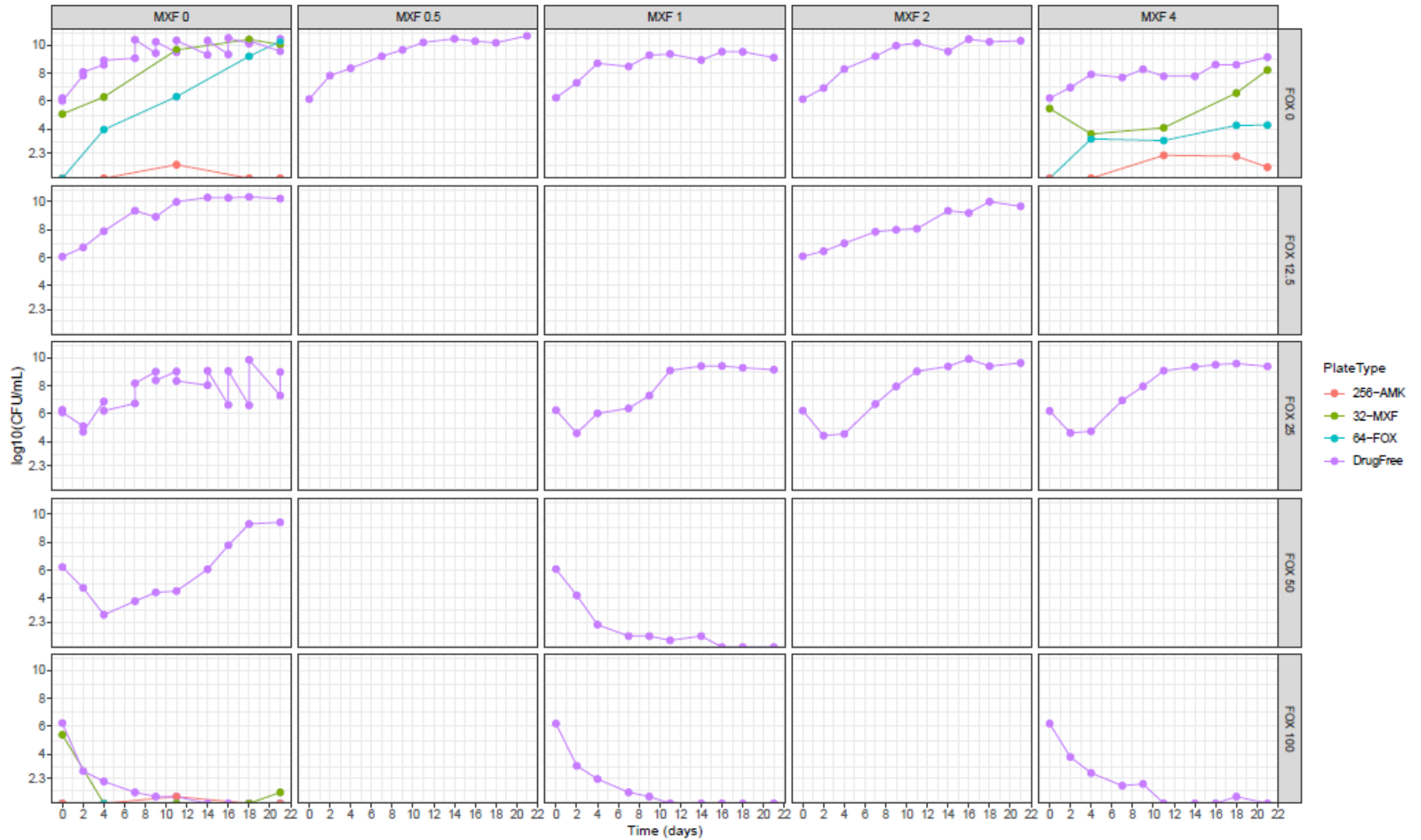
Figure XVI: Effect of cefoxitin and moxifloxacin combination at different concentrations achievable in humans. CFUs were determined at 0, 2, 4, 7, 9, 11, 14, 18 and 21 days.
