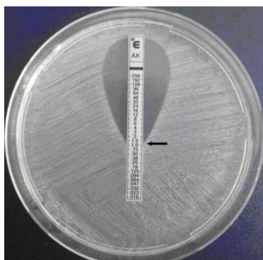
Figure 5: (A) AST by E-test method for single antibiotic, where arrow indicated the value for MIC (B) set up on agar plate for E-test combination testing
