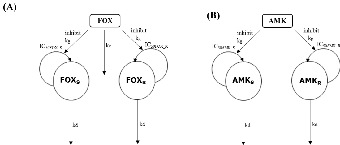
Figure S1: Schematic diagram of the final PK/PD model (A) FOX (B) AMK. Bacteria multiplied with a first-order rate constant ( k_g ) in the susceptible ( S ) and resistant ( R ) bacterial compartment and all bacteria had natural death-rate ( k_d ). Cefoxitin followed a with a first-order degradation process ( k_e ). Antibiotic compartment was driven to the bacterial growth inhibition following an I_{max} model \left(1 - \left(\frac{I_{max} \times C^{\gamma}}{IC_{50}^{\gamma} + C^{\gamma}}\right)\right) .
