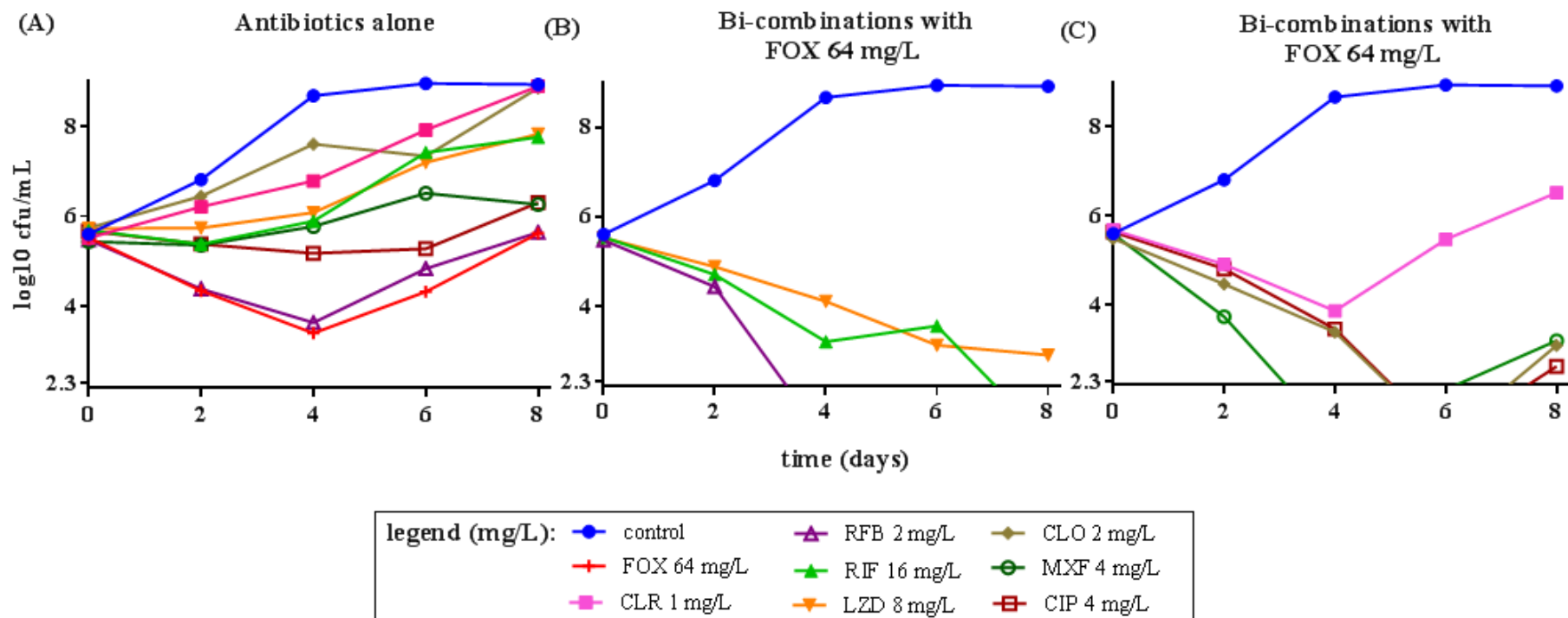
Figure 3: Effect of various combinations on M. abscessus T28. (A) Activity of several screened antibiotics alone, (B) ceftioxin in combination with linezolid, rifampicin and rifabutin, and (C) ceftioxin in combination with clarithromycin, clofazimine, moxifloxacin and ciprofloxacin. 50% amount of FOX was compensated each 24h up to 8 days to maintain the FOX amount constant throughout the experiment. CFUs were determined at the interval of 2 days. The dashed line represents the limit of quantification.
