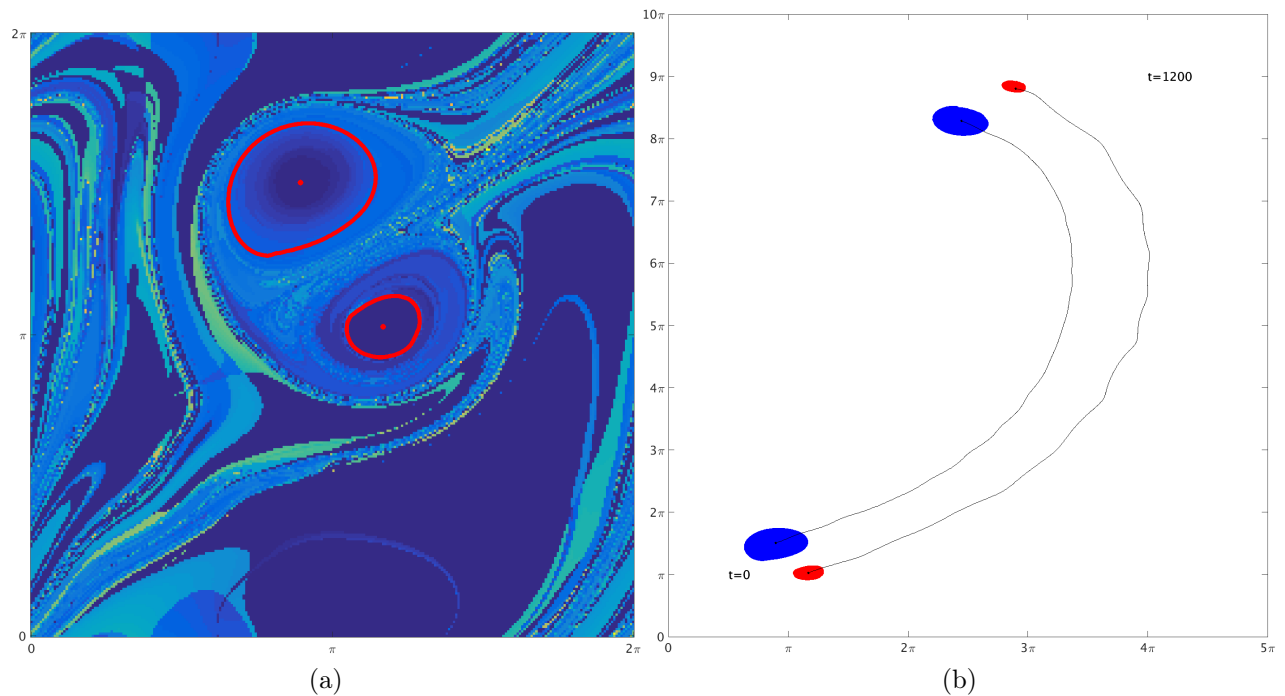
Figure 6-10: a) Coherent vortices and their centers at time t_0 extracted from the velocity field generated by Navier-Stokes model 6.5 using definition.1 with the \mathcal{L}ACCL_{t_0}^{t_f}(\mathbf{x}_0) map shown in background . b) Their initial and final positions under Lagrangian advection. (See the supplemental movie M3 for the complete advection sequence of these vortices.)
