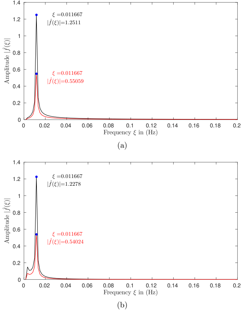
Figure 7-3: Frequency-domain representation of the particles' trajectories in Fig.7-1, red an black trajectories have the same frequency but different amplitudes: a) within x -direction, b) within y -direction.
