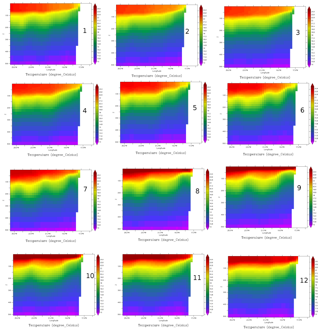
Figure 3-10: GLORYS2V4: monthly Temperature V-section of the year 2010 in the point (lat = 21.42^{\circ}N lon = -18.51^{\circ}N )
