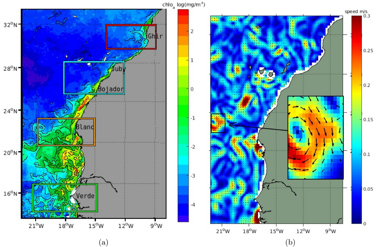
Figure 5-1: a) Chlorophyll image with MSM fronts overlaid on top, b) Surface velocity and direction. Both at the same date (01-March-2003).
