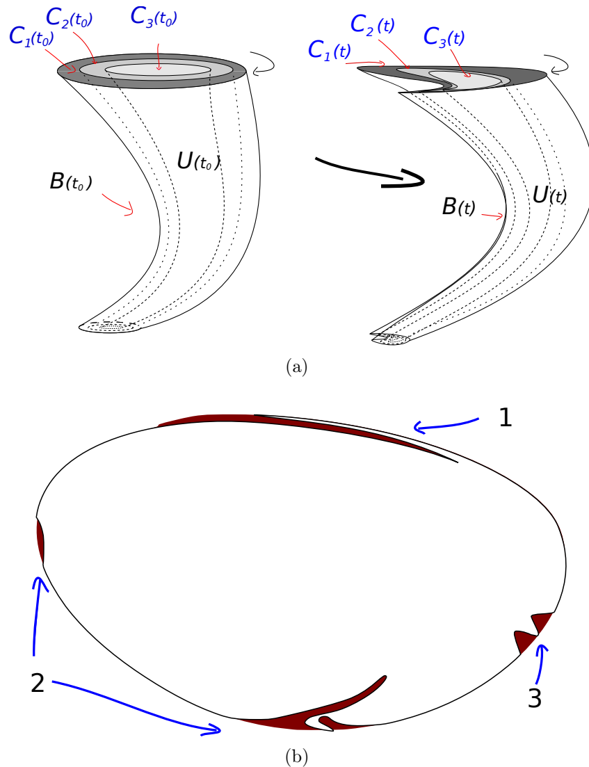
Figure 7-4: a) Initial and time t positions of a coherent Lagrangian vortex \mathbf{U}(t) and a Lagrangian vortex boundary \mathbf{B}(t) . Also shown within \mathbf{U}(t) are different vortex cores \mathbf{C}(t) along which particles' trajectories share different frequencies over the time interval [t_0, t] . b) An example of a closed material line which profits from the relaxation of convexity to small convexity deficiency. Dark red area indicates the area difference between the closed material line and its convex hull: (1) minor tangential filamentation, (2) deformation by smaller-scale vortices, (3) discrete approximation of a convexity.
