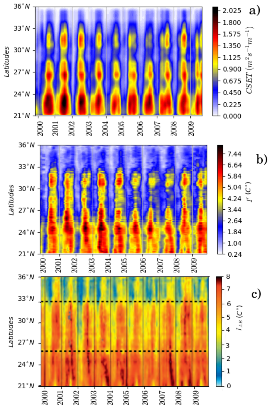
Figure 3-4: Space-time Hovmöller plot of the seasonal and interannual variability of: a) I_{CSET} b) I' index and c) I_{AB} index between 2000 and 2009.
