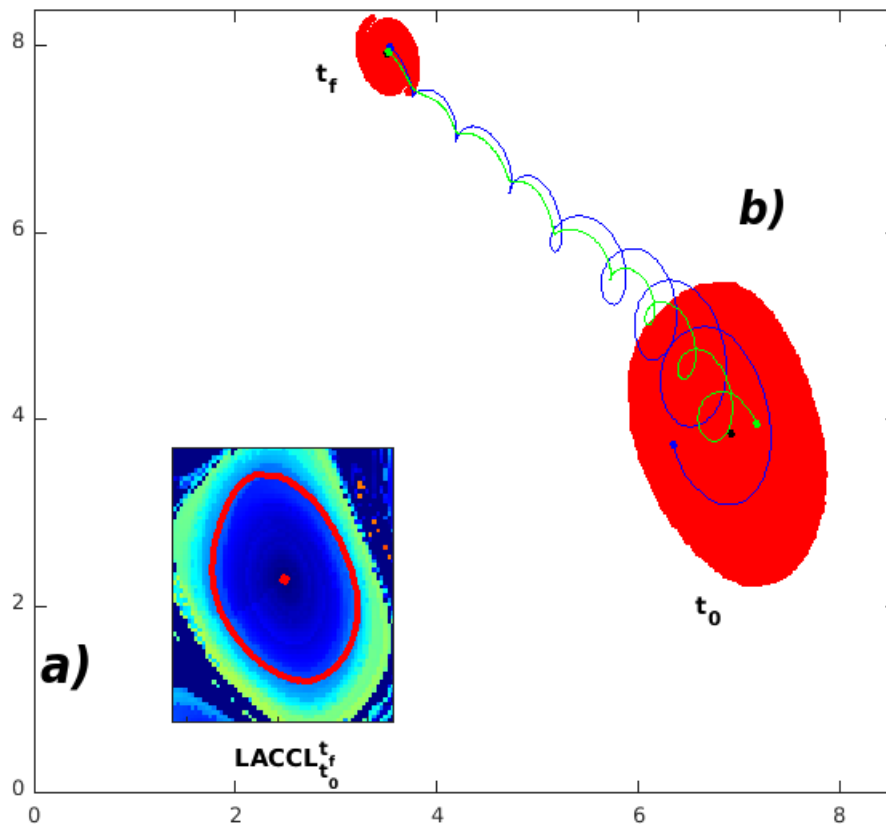
Figure 6-14: a) Coherent vortex and its center at time t_0 extracted using definition.1 with the \mathcal{LACCL}_{t_0}^{t_f}(\mathbf{x}_0) map shown in background . b) Its initial and final positions under Lagrangian advection. (See the supplemental movie M6 for the complete advection sequence of this vortices.).
