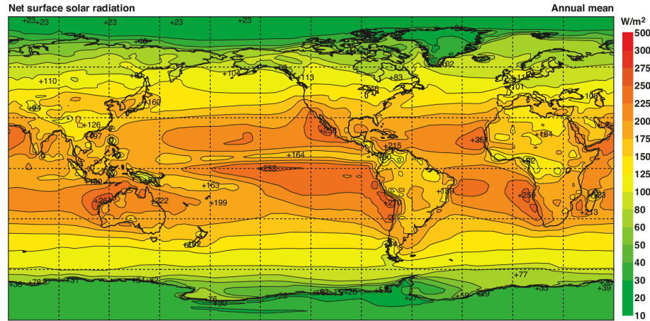
Figure 1-2: Heating of earth's surface by solar radiation, in W/m^2 , calculated from the ECMWF 40-year reanalysis of atmospheric data. The tropics absorb more heat than they lose, while the poles lose more heat than they absorb. This imbalance drives the planetary heat engine 2 .
