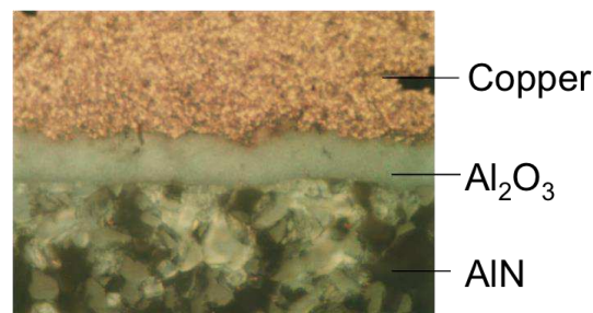
Figure 52 : Interface DBC [40]
