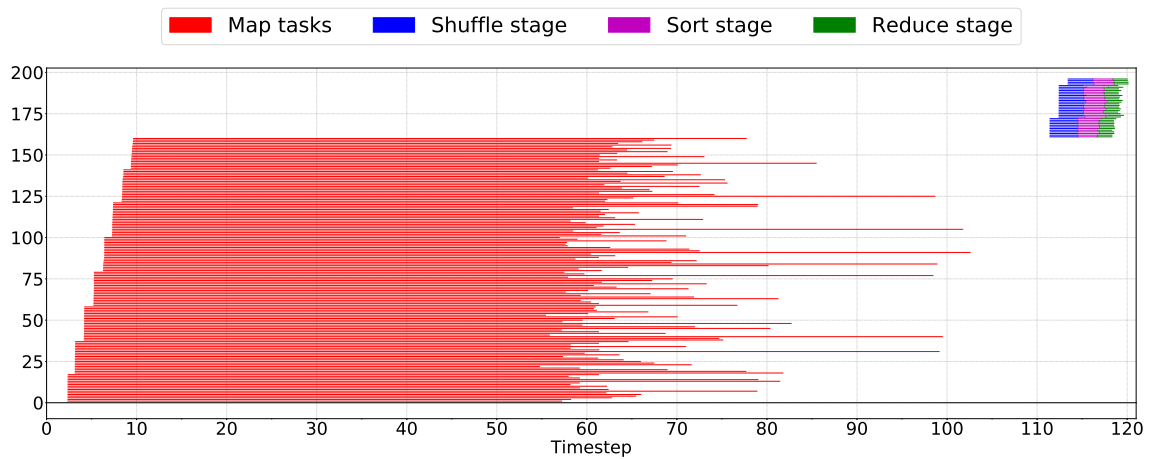
Figure 11.7: Tasks of Wordcount application under default EC and EC-aware placements (non-overlapping shuffle) for 40 GB input size.
